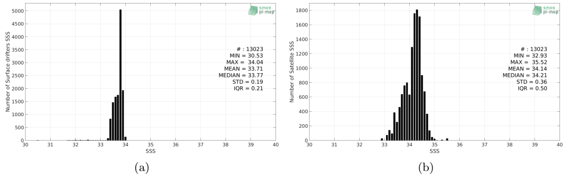
Figure 2: Histograms of SSS from Surface drifters (a) and SMOS L3 v2 - 9-Days (BEC) (b) considering all match-up pairs per bins of 0.1 over the Southern Ocean Pi-MEP region and for the full satellite product period.
