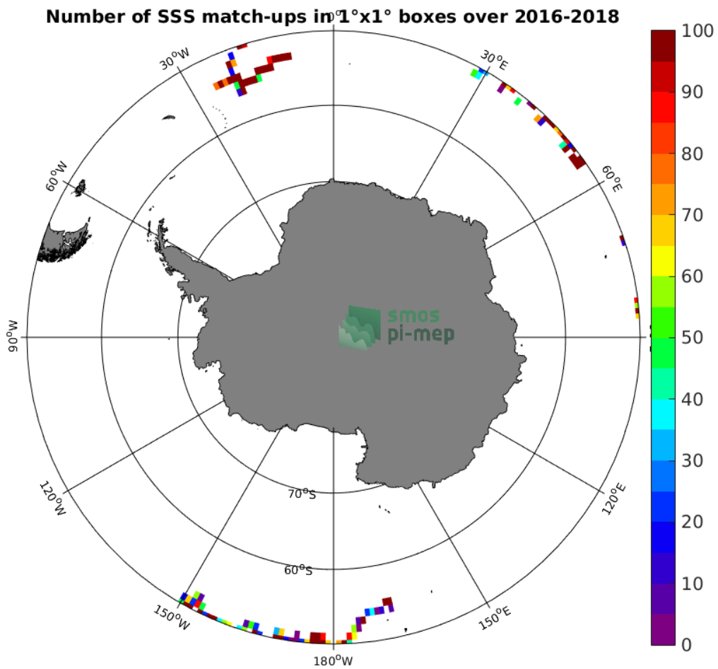
Figure 3: Number of SSS match-ups between Surface drifters SSS and the SMOS L3 v2 - 9-Days (BEC) SSS product for the Southern Ocean Pi-MEP region over 1^\circ \times 1^\circ boxes and for the full satellite product period.
