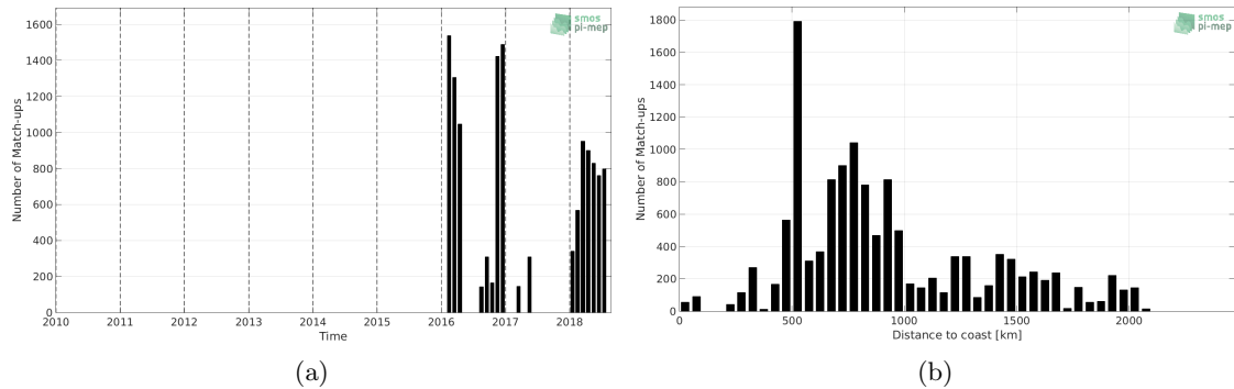
Figure 1: Number of match-ups between Surface drifters and SMOS L3 v2 - 9-Days (BEC) SSS as a function of time (a) and as function of the distance to coast (b) over the Southern Ocean Pi-MEP region and for the full satellite product period.
