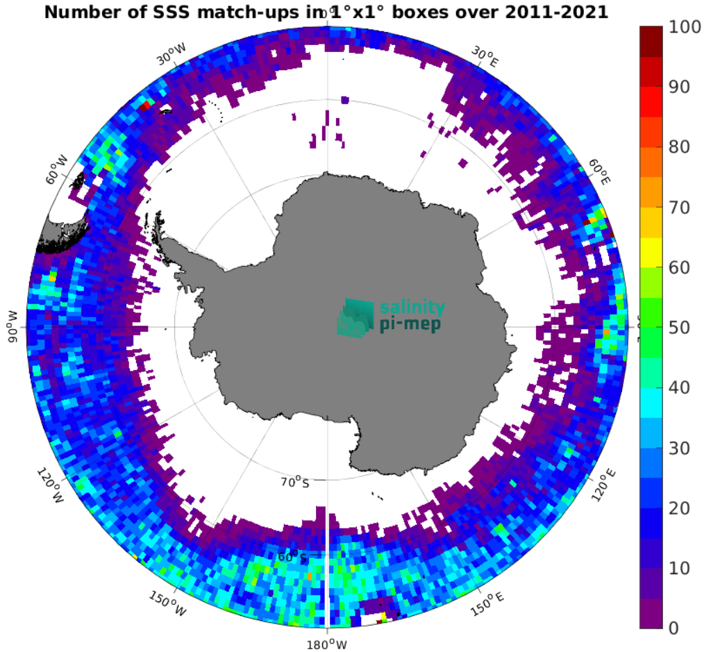
Figure 5: Number of SSS match-ups between Argo SSS and the SMOS SSS L3 v2 - 9-Days (BEC) SSS product for the Southern Ocean Pi-MEP region over 1^\circ \times 1^\circ boxes and for the full satellite product period.
