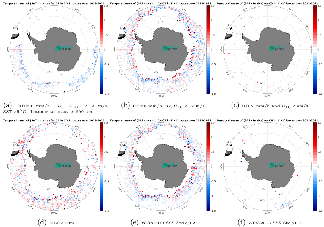
Figure 14: Temporal mean gridded over spatial boxes of size 1^\circ \times 1^\circ of \Delta SSS (SMOS SSS L3 v2 - 9-Days (BEC) - Argo) for 6 different subdatasets corresponding to:RR=0 mm/h, 3 < U_{10} < 12 m/s, SST>5°C, distance to coast > 800 km (a), RR=0 mm/h, 3 < U_{10} < 12 m/s (b), RR>1mm/h and U_{10} < 4 m/s (c),MLD<20m (d),WOA2013 SSS Std<0.2 (e),WOA2013 SSS Std>0.2 (f).
