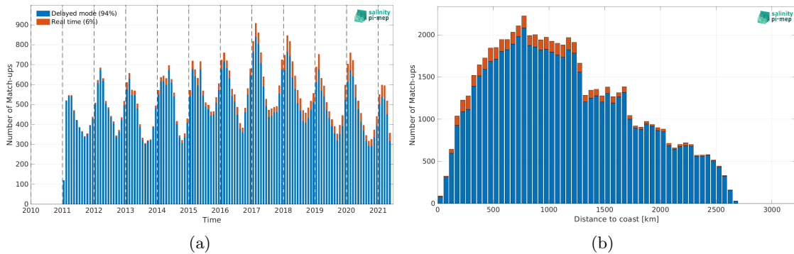
Figure 2: Number of match-ups between Argo and SMOS SSS L3 v2 - 9-Days (BEC) SSS as a function of time (a) and as function of the distance to coast (b) over the Southern Ocean Pi-MEP region and for the full satellite product period.
