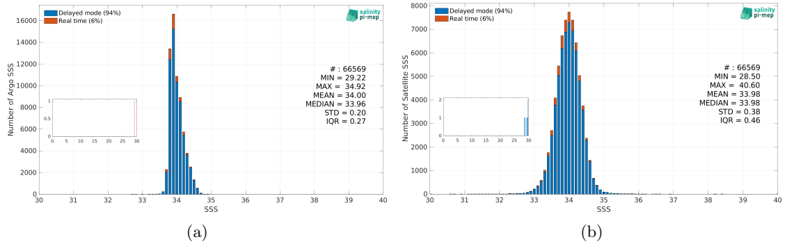
Figure 3: Histograms of SSS from Argo (a) and SMOS SSS L3 v2 - 9-Days (BEC) (b) considering all match-up pairs per bins of 0.1 over the Southern Ocean Pi-MEP region and for the full satellite product period.
