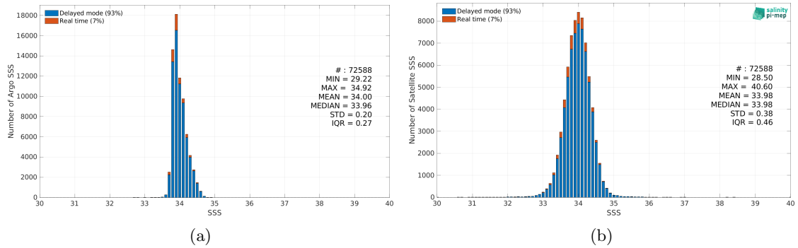
Figure 2: Histograms of SSS from Argo (a) and SMOS SSS L3 v2 - 9-Days (BEC) (b) considering all match-up pairs per bins of 0.1 over the Southern Ocean Pi-MEP region and for the full satellite product period.
