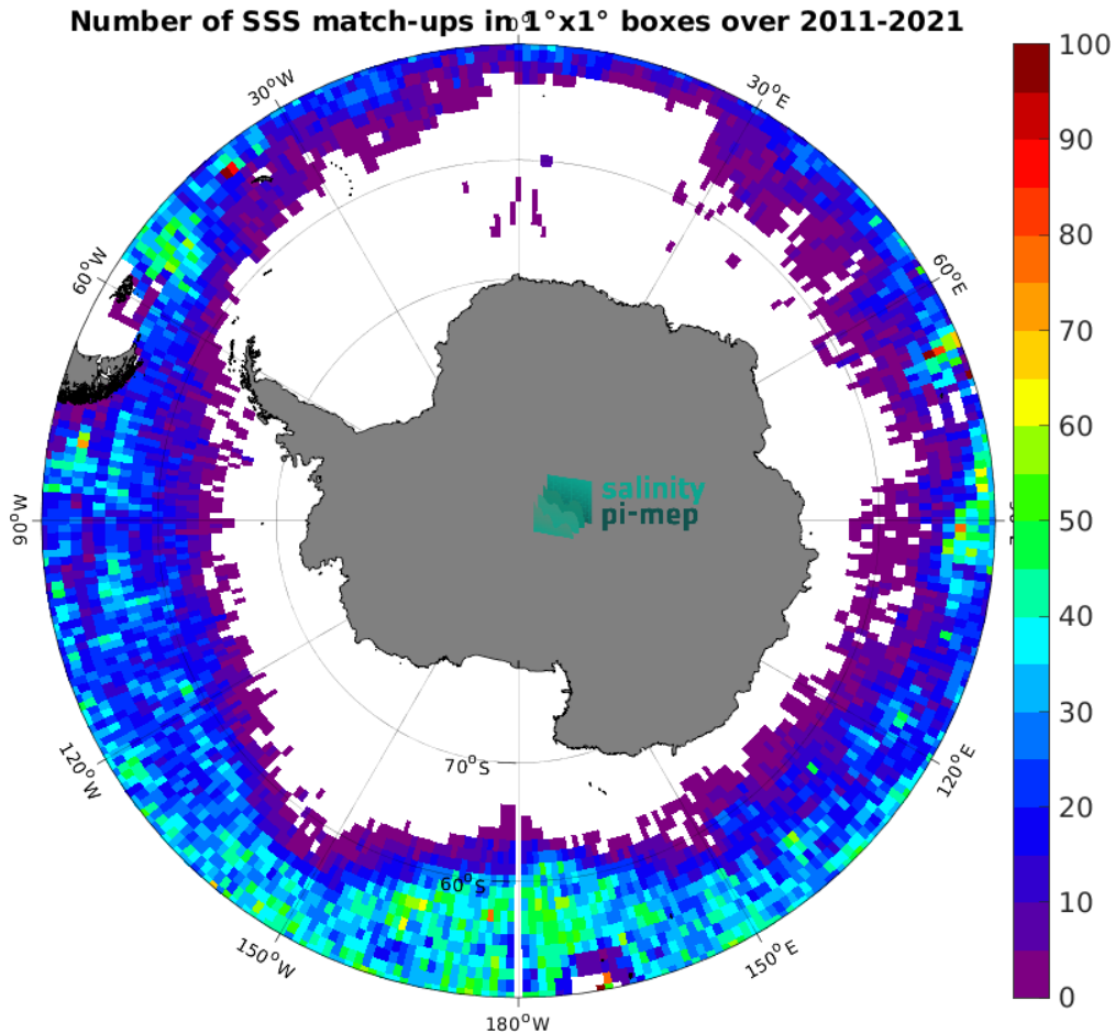
Figure 4: Number of SSS match-ups between Argo SSS and the SMOS SSS L3 v2 - 9-Days (BEC) SSS product for the Southern Ocean Pi-MEP region over 1^\circ \times 1^\circ boxes and for the full satellite product period.
