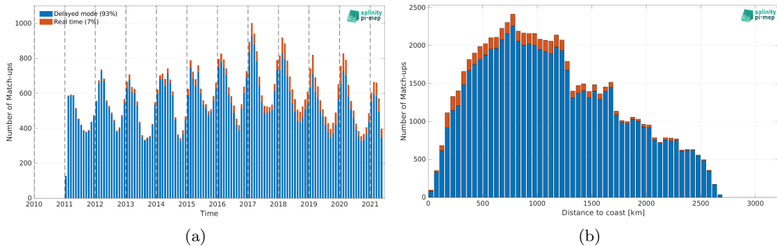
Figure 1: Number of match-ups between Argo and SMOS SSS L3 v2 - 9-Days (BEC) SSS as a function of time (a) and as function of the distance to coast (b) over the Southern Ocean Pi-MEP region and for the full satellite product period.
