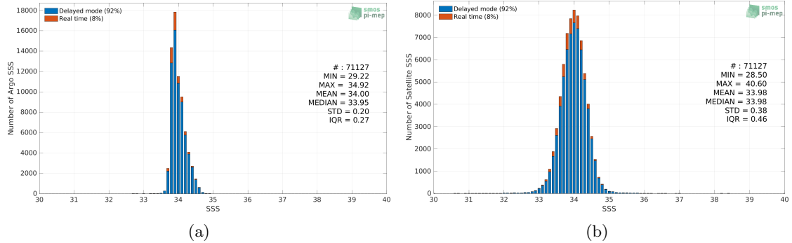
Figure 2: Histograms of SSS from Argo (a) and SMOS SSS L3 v2 - 9-Days (BEC) (b) considering all match-up pairs per bins of 0.1 over the Southern Ocean Pi-MEP region and for the full satellite product period.
