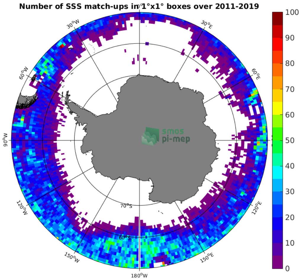
Figure 4: Number of SSS match-ups between Argo SSS and the SMOS SSS L3 v2 - 9-Days (BEC) SSS product for the Southern Ocean Pi-MEP region over 1^\circ \times 1^\circ boxes and for the full satellite product period.
