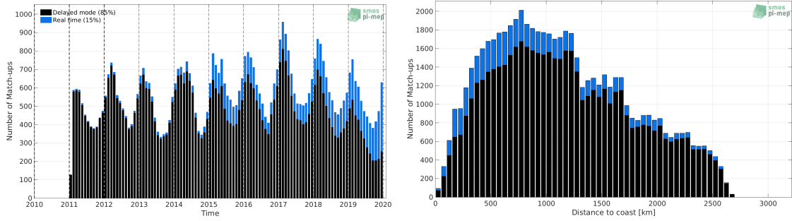
Figure 1: Number of match-ups between Argo and SMOS SSS L3 v2 - 9-Days (BEC) SSS as a function of time (a) and as function of the distance to coast (b) over the Southern Ocean Pi-MEP region and for the full satellite product period.
