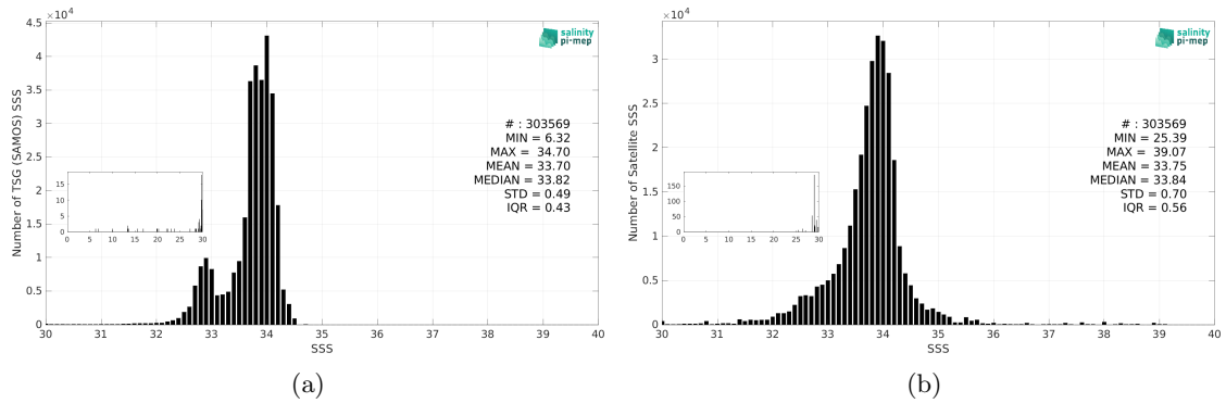
Figure 3: Histograms of SSS from TSG (SAMOS) (a) and SMOS SSS L3 Southern Ocean v1 - 9-Day running mean (BEC) (b) considering all match-up pairs per bins of 0.1 over the Southern Ocean Pi-MEP region and for the full satellite product period.
