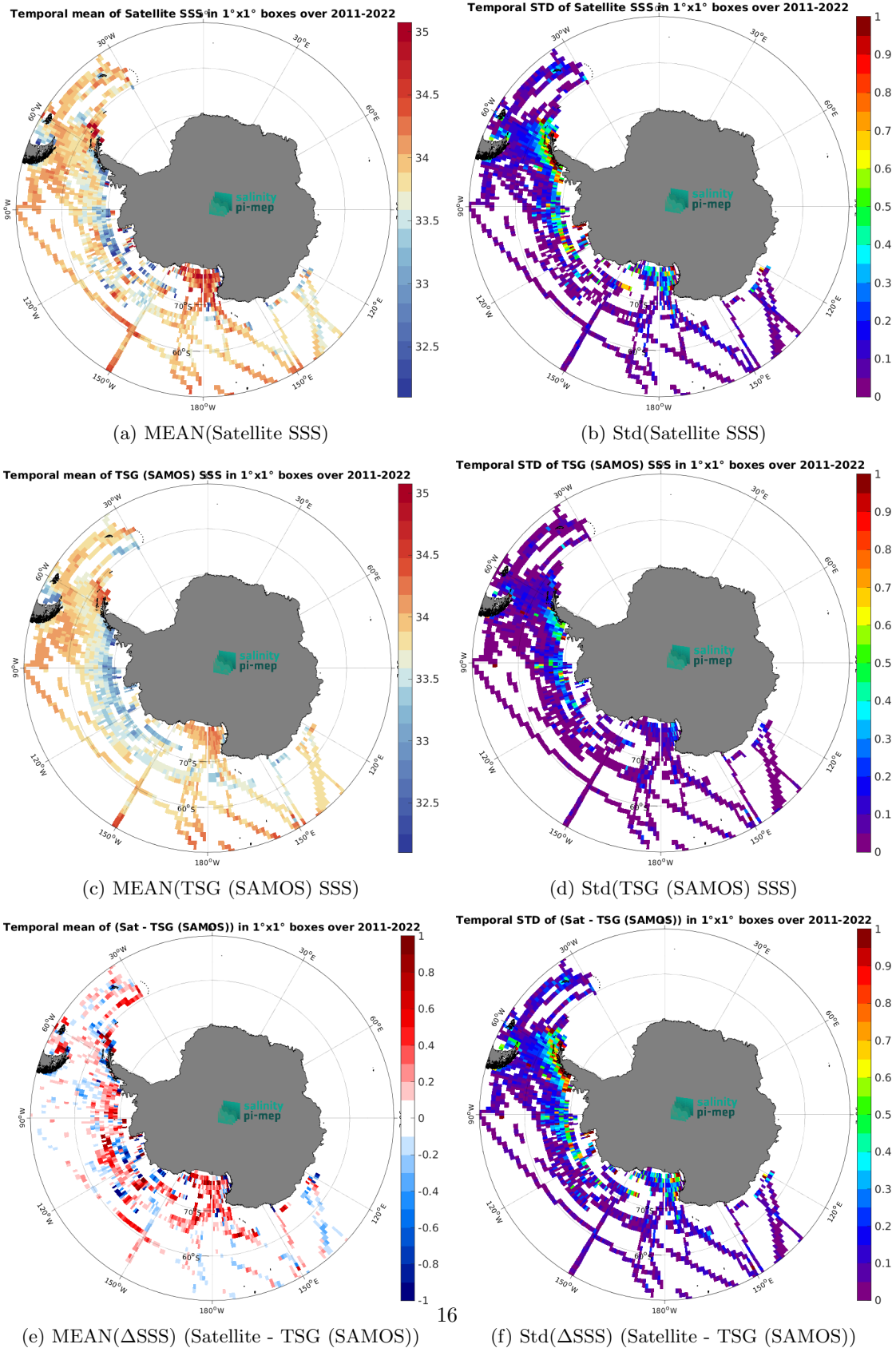
Figure 7: Temporal mean (left) and Std (right) of SSS from SMOS SSS L3 Southern Ocean v1 - 9-Day running mean (BEC) (top), TSG (SAMOS) (middle), and of \Delta SSS (Satellite - TSG (SAMOS)). Only match-up pairs are used to generate these maps.
