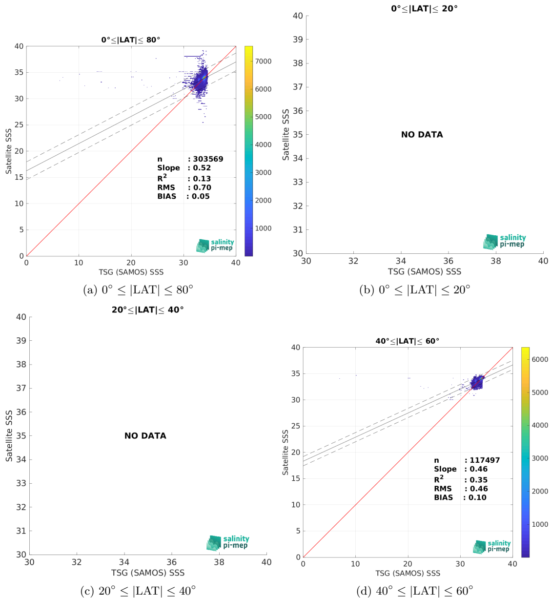
Figure 10: Contour maps of the concentration of SMOS SSS L3 Southern Ocean v1 - 9-Day running mean (BEC) SSS (y-axis) versus TSG (SAMOS) SSS (x-axis) at match-up pairs for different latitude bands. For each plot, the red line shows x=y . The black thin and dashed lines indicate a linear fit through the data cloud and the \pm 95\% confidence levels, respectively. The number match-up pairs n , the slope and R^2 coefficient of the linear fit, the root mean square (RMS) and the mean bias between satellite and in situ data are indicated for each latitude band in each plots.
