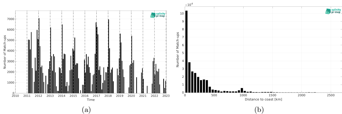
Figure 2: Number of match-ups between TSG (SAMOS) and SMOS SSS L3 Southern Ocean v1 - 9-Day running mean (BEC) SSS as a function of time (a) and as function of the distance to coast (b) over the Southern Ocean Pi-MEP region and for the full satellite product period.
