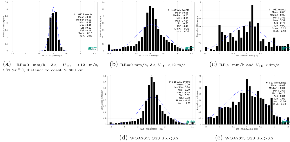
Figure 15: Normalized histogram of \Delta\text{SSS} (SMOS SSS L3 Southern Ocean v1 - 9-Day running mean (BEC) - TSG (SAMOS)) for 5 different subdatasets corresponding to: RR=0 mm/h, 3 < U_{10} < 12 m/s, SST>5°C, distance to coast > 800 km (a), RR=0 mm/h, 3 < U_{10} < 12 m/s (b), RR>1mm/h and U_{10} < 4 m/s (c), WOA2013 SSS Std<0.2 (d), WOA2013 SSS Std>0.2 (e).
