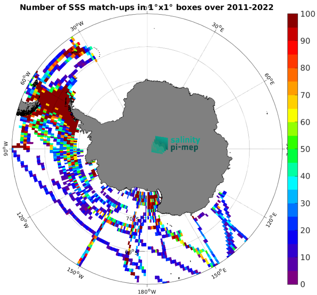
Figure 5: Number of SSS match-ups between TSG (SAMOS) SSS and the SMOS SSS L3 Southern Ocean v1 - 9-Day running mean (BEC) SSS product for the Southern Ocean Pi-MEP region over 1^\circ \times 1^\circ boxes and for the full satellite product period.
