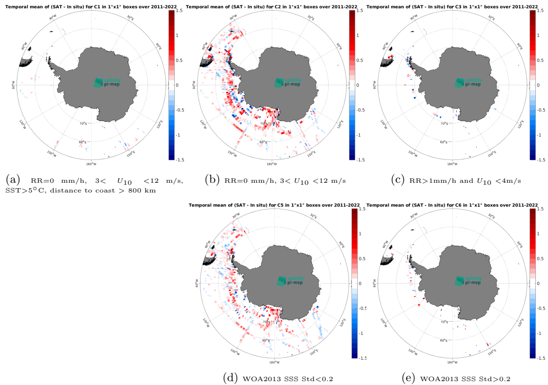
Figure 14: Temporal mean gridded over spatial boxes of size 1^\circ \times 1^\circ of \Delta SSS (SMOS SSS L3 Southern Ocean v1 - 9-Day running mean (BEC) - TSG (SAMOS)) for 5 different subdatasets corresponding to:RR=0 mm/h, 3 < U_{10} < 12 m/s, SST >5^\circ C, distance to coast > 800 km (a), RR=0 mm/h, 3 < U_{10} < 12 m/s (b), RR >1 mm/h and U_{10} < 4 m/s (c), WOA2013 SSS Std <0.2 (d), WOA2013 SSS Std >0.2 (e).
