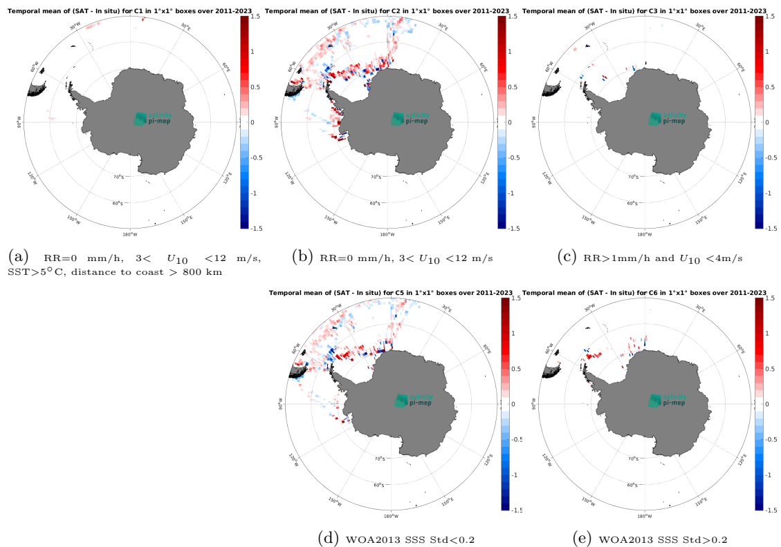
Figure 14: Temporal mean gridded over spatial boxes of size 1^\circ \times 1^\circ of \Delta\text{SSS} (SMOS SSS L3 Southern Ocean v1 - 9-Day running mean (BEC) - TSG (Polarstern)) for 5 different subdatasets corresponding to:RR=0 mm/h, 3 < U_{10} < 12 m/s, SST >5^\circ\text{C} , distance to coast > 800 km (a), RR=0 mm/h, 3 < U_{10} < 12 m/s (b), RR >1 mm/h and U_{10} < 4 m/s (c), WOA2013 SSS Std <0.2 (d), WOA2013 SSS Std >0.2 (e).
