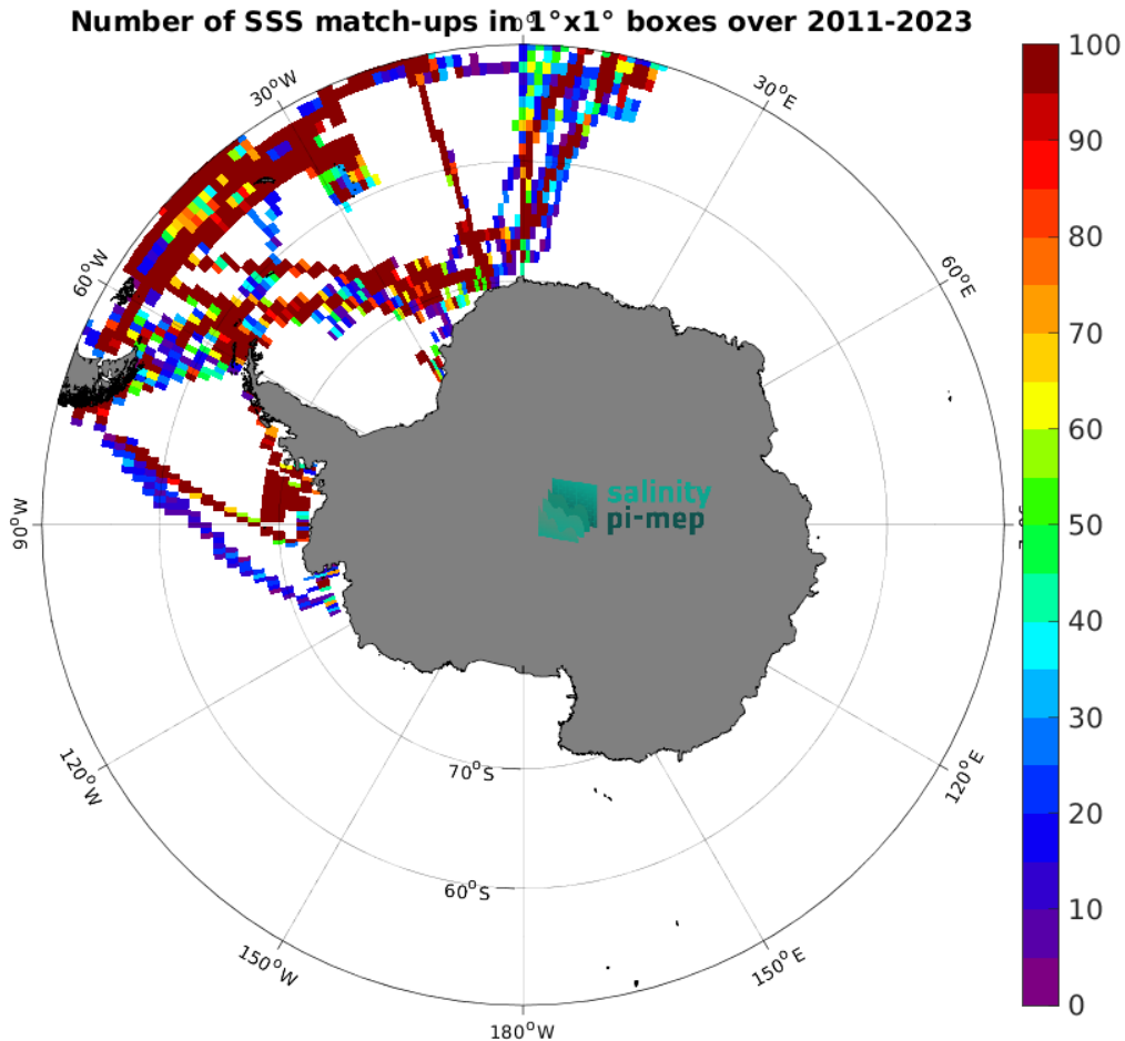
Figure 5: Number of SSS match-ups between TSG (Polarstern) SSS and the SMOS SSS L3 Southern Ocean v1 - 9-Day running mean (BEC) SSS product for the Southern Ocean Pi-MEP region over 1^\circ \times 1^\circ boxes and for the full satellite product period.
