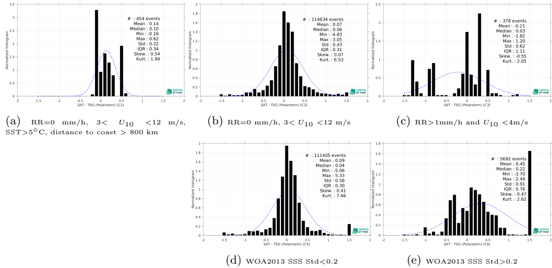
Figure 15: Normalized histogram of \Delta SSS (SMOS SSS L3 Southern Ocean v1 - 9-Day running mean (BEC) - TSG (Polarstern)) for 5 different subdatasets corresponding to: RR=0 mm/h, 3 < U_{10} < 12 m/s, SST>5°C, distance to coast > 800 km (a), RR=0 mm/h, 3 < U_{10} < 12 m/s (b), RR>1mm/h and U_{10} < 4 m/s (c), WOA2013 SSS Std<0.2 (d), WOA2013 SSS Std>0.2 (e).
