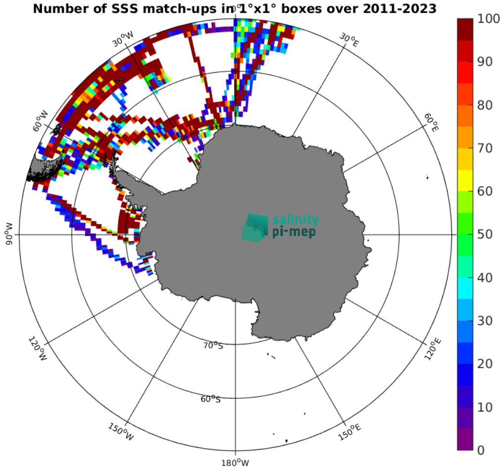
Figure 5: Number of SSS match-ups between TSG (Polarstern) SSS and the SMOS SSS L3 Southern Ocean v1 - 9-Day running mean (BEC) SSS product for the Southern Ocean Pi-MEP region over 1^\circ \times 1^\circ boxes and for the full satellite product period.
