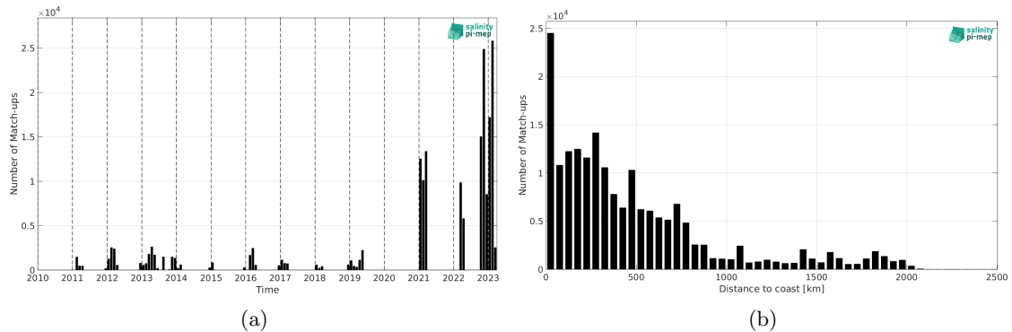
Figure 2: Number of match-ups between TSG (Polarstern) and SMOS SSS L3 Southern Ocean v1 - 9-Day running mean (BEC) SSS as a function of time (a) and as function of the distance to coast (b) over the Southern Ocean Pi-MEP region and for the full satellite product period.
