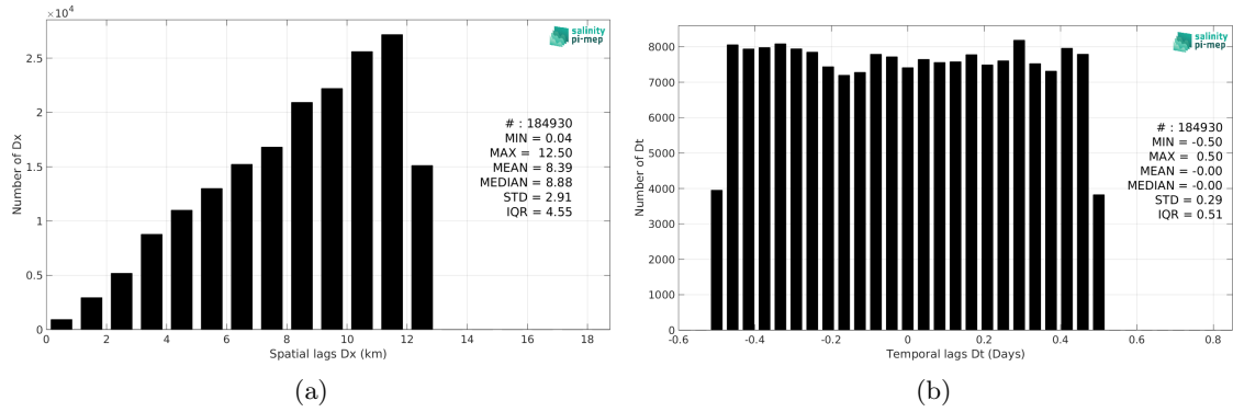
Figure 6: Histograms of the spatial (a) and temporal (b) lags between the location/time of the TSG (Polarstern) measurement and the date of the corresponding SMOS SSS L3 Southern Ocean v1 - 9-Day running mean (BEC) SSS pixel.
