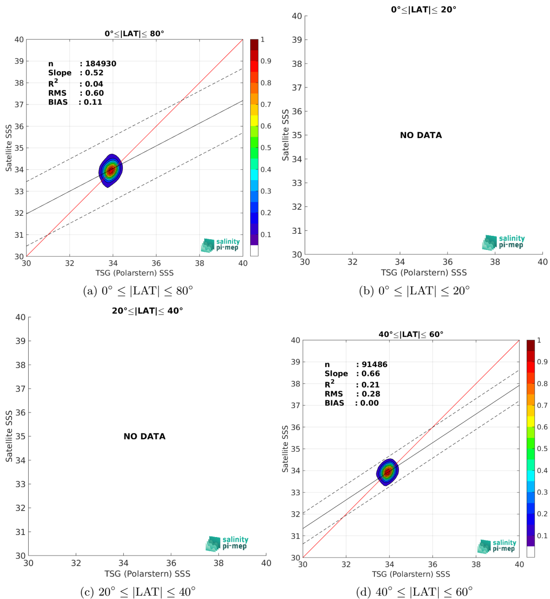
Figure 10: Contour maps of the concentration of SMOS SSS L3 Southern Ocean v1 - 9-Day running mean (BEC) SSS (y-axis) versus TSG (Polarstern) SSS (x-axis) at match-up pairs for different latitude bands. For each plot, the red line shows x=y . The black thin and dashed lines indicate a linear fit through the data cloud and the \pm 95\% confidence levels, respectively. The number match-up pairs n , the slope and R^2 coefficient of the linear fit, the root mean square (RMS) and the mean bias between satellite and in situ data are indicated for each latitude band in each plots.
