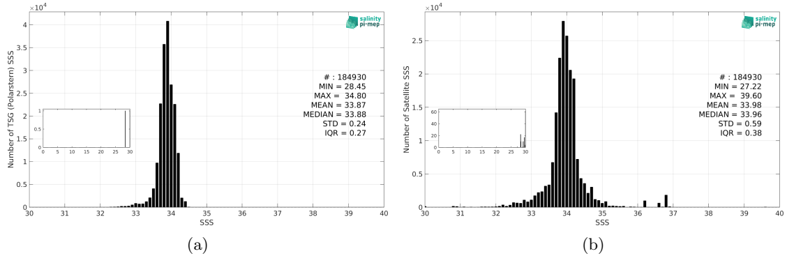
Figure 3: Histograms of SSS from TSG (Polarstern) (a) and SMOS SSS L3 Southern Ocean v1 - 9-Day running mean (BEC) (b) considering all match-up pairs per bins of 0.1 over the Southern Ocean Pi-MEP region and for the full satellite product period.
