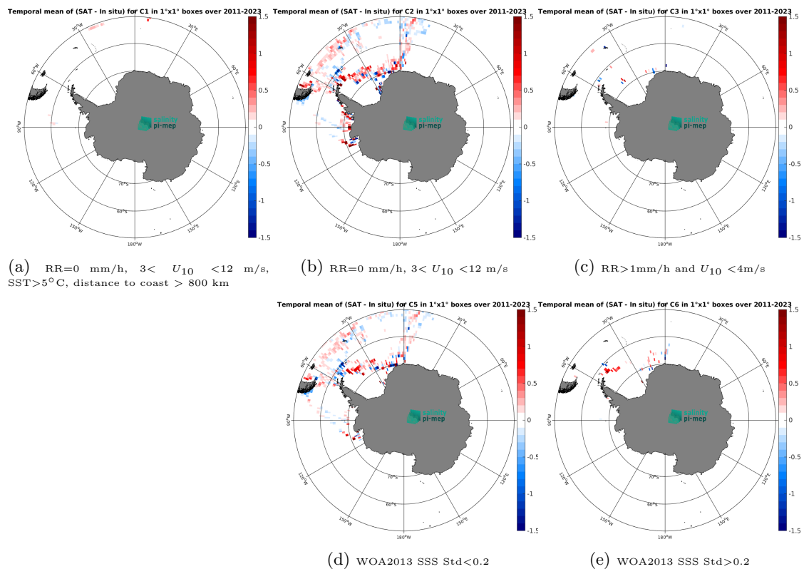
Figure 14: Temporal mean gridded over spatial boxes of size 1^\circ \times 1^\circ of \Delta SSS (SMOS SSS L3 Southern Ocean v1 - 9-Day running mean (BEC) - TSG (Polarstern)) for 5 different subdatasets corresponding to:RR=0 mm/h, 3 < U_{10} < 12 m/s, SST >5^\circ C, distance to coast > 800 km (a), RR=0 mm/h, 3 < U_{10} < 12 m/s (b), RR >1 mm/h and U_{10} < 4 m/s (c), WOA2013 SSS Std <0.2 (d), WOA2013 SSS Std >0.2 (e).
