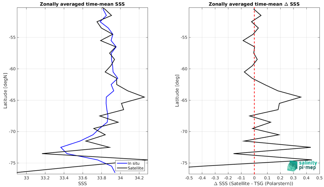
Figure 9: Left panel: Zonal mean SSS from SMOS SSS L3 Southern Ocean v1 - 9-Day running mean (BEC) satellite product (black) and from TSG (Polarstern) (blue). Right panel: Zonal mean of \Delta SSS (Satellite - TSG (Polarstern)) for all the collected Pi-MEP match-up pairs estimated over the full satellite product period.
