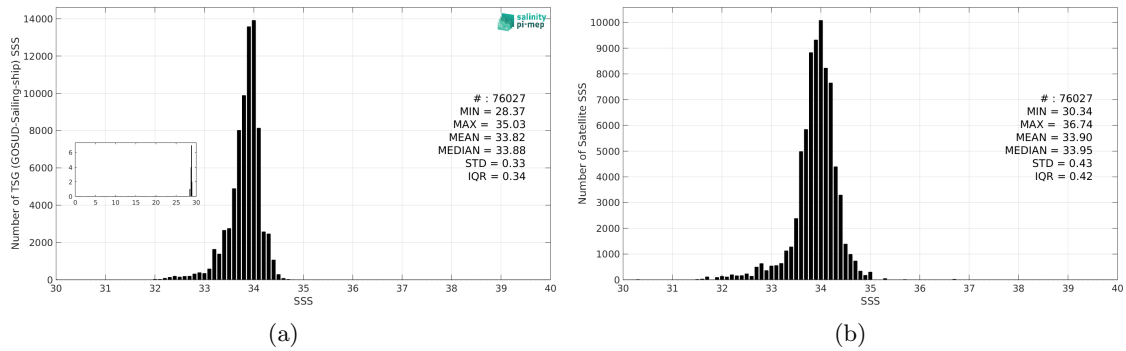
Figure 3: Histograms of SSS from TSG (GOSUD-Sailing-ship) (a) and SMOS SSS L3 Southern Ocean v1 - 9-Day running mean (BEC) (b) considering all match-up pairs per bins of 0.1 over the Southern Ocean Pi-MEP region and for the full satellite product period.
