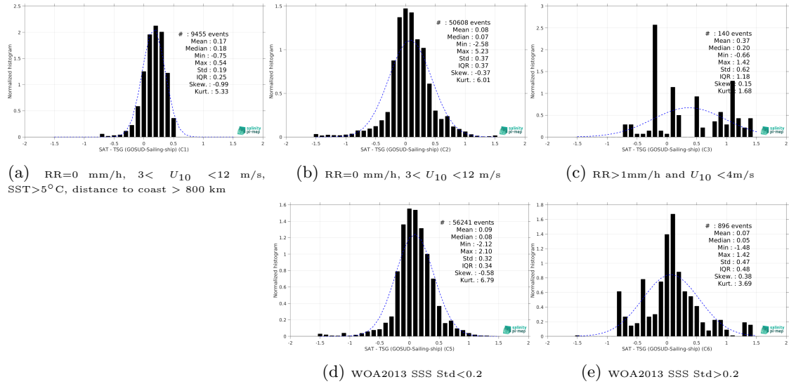
Figure 15: Normalized histogram of \Delta SSS (SMOS SSS L3 Southern Ocean v1 - 9-Day running mean (BEC) - TSG (GOSUD-Sailing-ship)) for 5 different subdatasets corresponding to: RR=0 mm/h, 3 < U_{10} < 12 m/s, SST>5°C, distance to coast > 800 km (a), RR=0 mm/h, 3 < U_{10} < 12 m/s (b), RR>1mm/h and U_{10} < 4 m/s (c), WOA2013 SSS Std<0.2 (d), WOA2013 SSS Std>0.2 (e).
