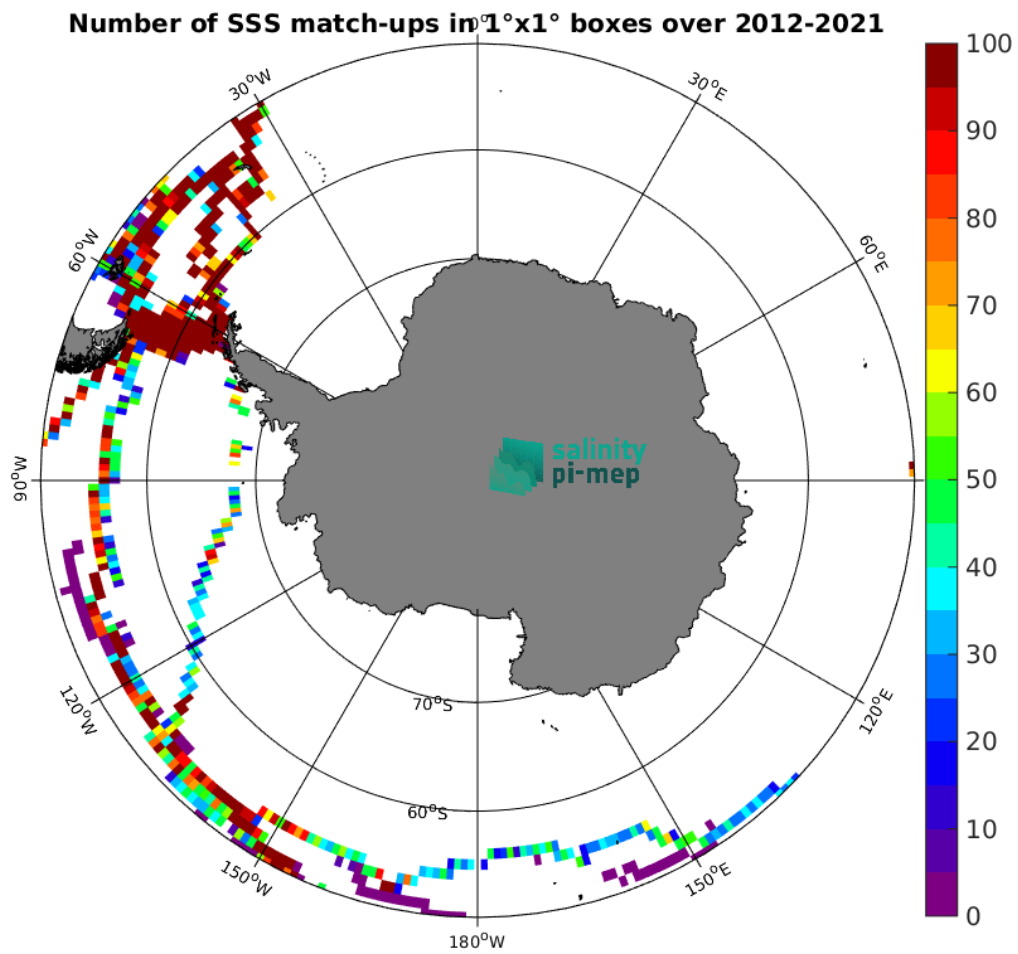
Figure 5: Number of SSS match-ups between TSG (GOSUD-Sailing-ship) SSS and the SMOS SSS L3 Southern Ocean v1 - 9-Day running mean (BEC) SSS product for the Southern Ocean Pi-MEP region over 1^\circ \times 1^\circ boxes and for the full satellite product period.
