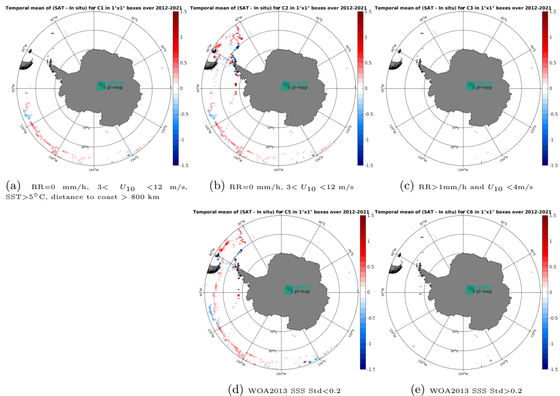
Figure 14: Temporal mean gridded over spatial boxes of size 1^\circ \times 1^\circ of \Delta SSS (SMOS SSS L3 Southern Ocean v1 - 9-Day running mean (BEC) - TSG (GOSUD-Sailing-ship)) for 5 different subdatasets corresponding to:RR=0 mm/h, 3 < U_{10} < 12 m/s, SST >5^\circ C, distance to coast > 800 km (a), RR=0 mm/h, 3 < U_{10} < 12 m/s (b), RR >1 mm/h and U_{10} < 4 m/s (c), WOA2013 SSS Std <0.2 (d), WOA2013 SSS Std >0.2 (e).
