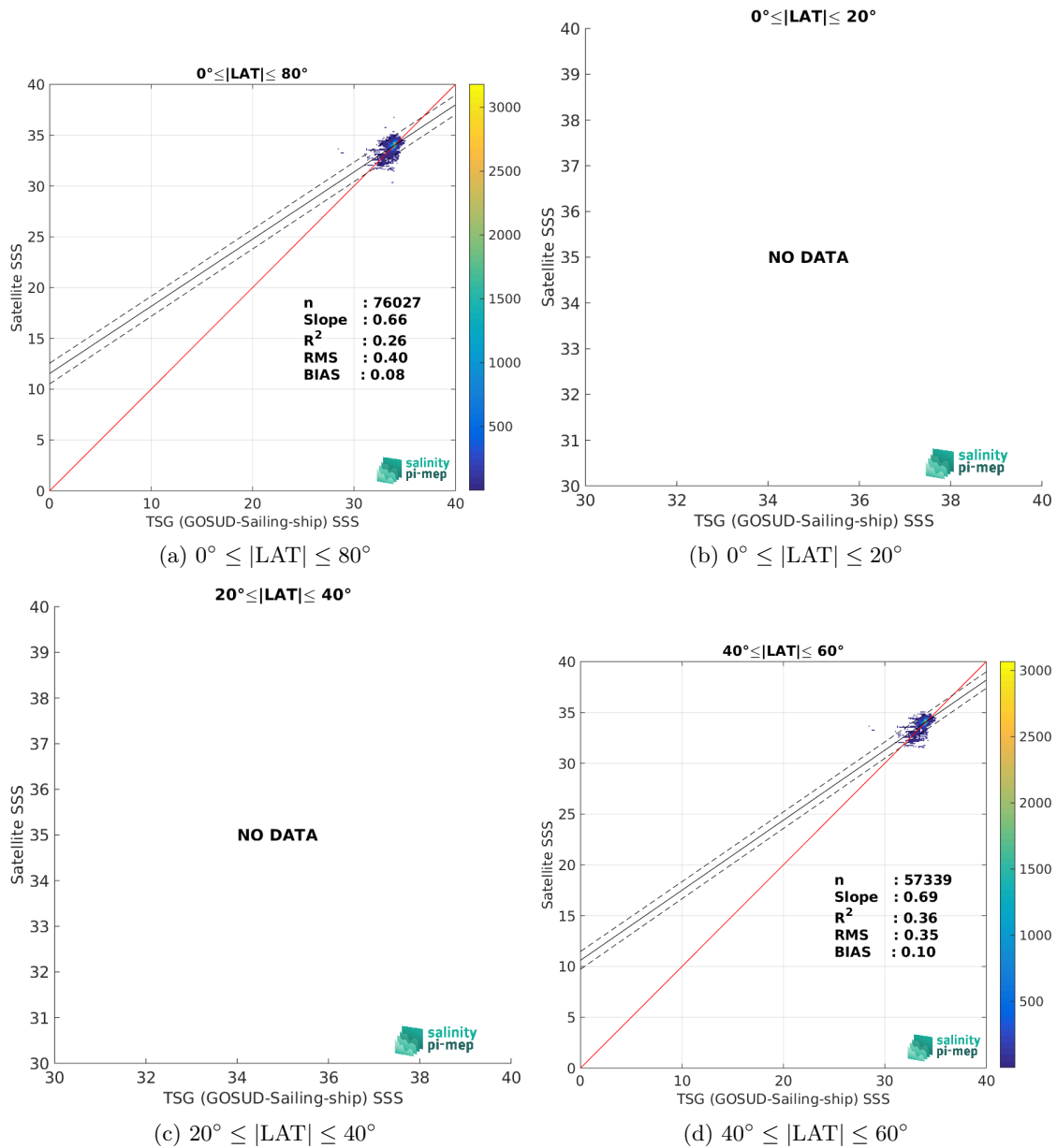
Figure 10: Contour maps of the concentration of SMOS SSS L3 Southern Ocean v1 - 9-Day running mean (BEC) SSS (y-axis) versus TSG (GOSUD-Sailing-ship) SSS (x-axis) at match-up pairs for different latitude bands. For each plot, the red line shows x=y . The black thin and dashed lines indicate a linear fit through the data cloud and the \pm 95\% confidence levels, respectively. The number match-up pairs n , the slope and R^2 coefficient of the linear fit, the root mean square (RMS) and the mean bias between satellite and in situ data are indicated for each latitude band in each plots.
