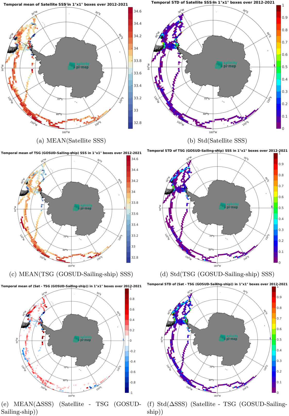
Figure 7: Temporal mean (left) and Std (right) of SSS from SMOS SSS L3 Southern Ocean v1 - 9-Day running mean (BEC) (top), TSG (GOSUD-Sailing-ship) (middle), and of \Delta SSS (Satellite - TSG (GOSUD-Sailing-ship)). Only match-up pairs are used to generate these maps.
