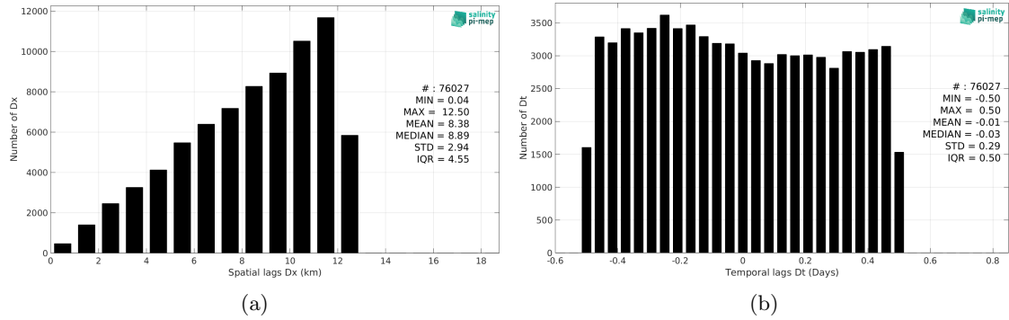
Figure 6: Histograms of the spatial (a) and temporal (b) lags between the location/time of the TSG (GOSUD-Sailing-ship) measurement and the date of the corresponding SMOS SSS L3 Southern Ocean v1 - 9-Day running mean (BEC) SSS pixel.
