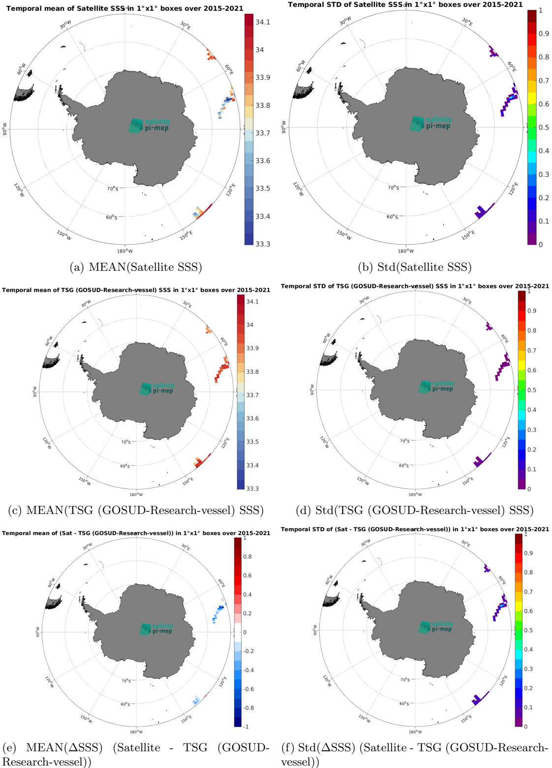
Figure 7: Temporal mean (left) and Std (right) of SSS from SMOS SSS L3 Southern Ocean v1 - 9-Day running mean (BEC) (top), TSG (GOSUD-Research-vessel) (middle), and of \Delta SSS (Satellite - TSG (GOSUD-Research-vessel)). Only match-up pairs are used to generate these maps.
