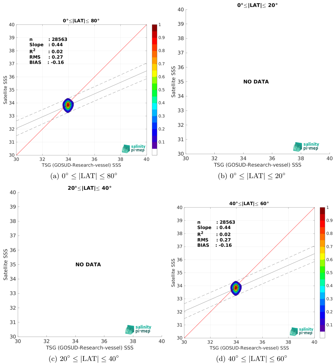
Figure 10: Contour maps of the concentration of SMOS SSS L3 Southern Ocean v1 - 9-Day running mean (BEC) SSS (y-axis) versus TSG (GOSUD-Research-vessel) SSS (x-axis) at match-up pairs for different latitude bands. For each plot, the red line shows x=y . The black thin and dashed lines indicate a linear fit through the data cloud and the \pm 95\% confidence levels, respectively. The number match-up pairs n , the slope and R^2 coefficient of the linear fit, the root mean square (RMS) and the mean bias between satellite and in situ data are indicated for each latitude band in each plots.
