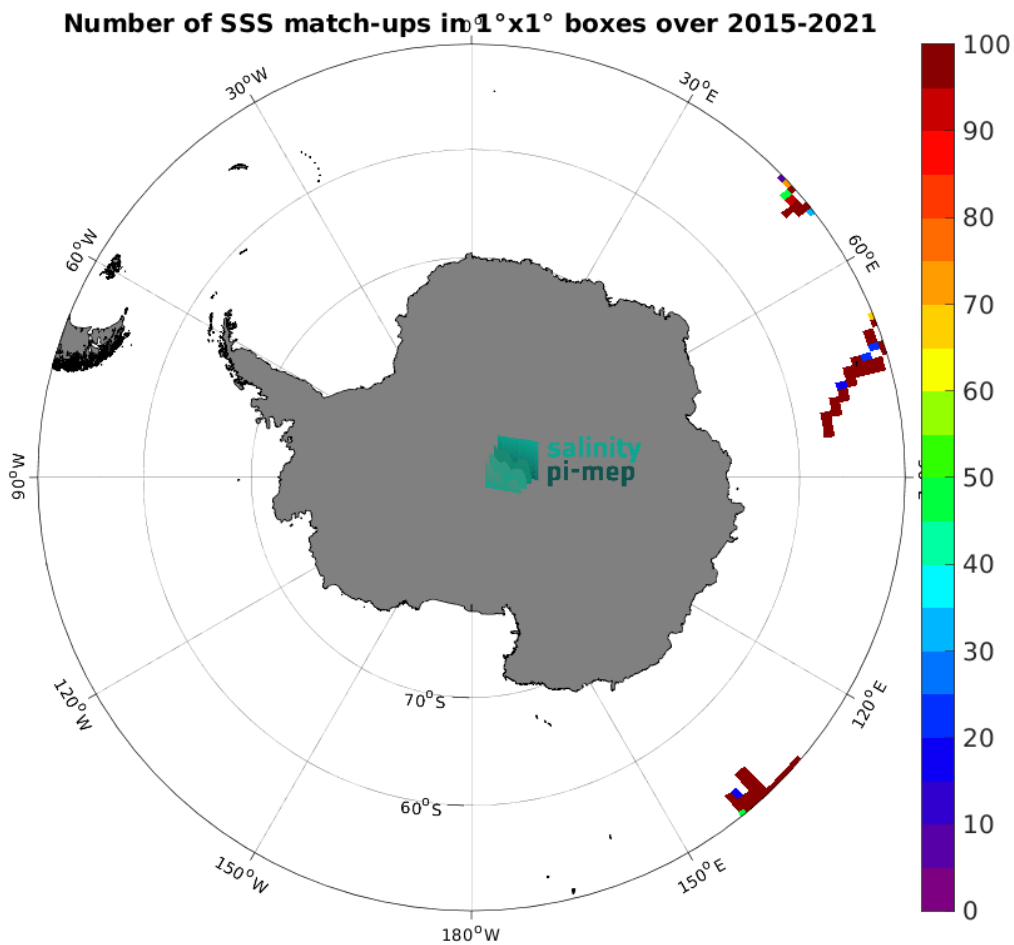
Figure 5: Number of SSS match-ups between TSG (GOSUD-Research-vessel) SSS and the SMOS SSS L3 Southern Ocean v1 - 9-Day running mean (BEC) SSS product for the Southern Ocean Pi-MEP region over 1^\circ \times 1^\circ boxes and for the full satellite product period.
