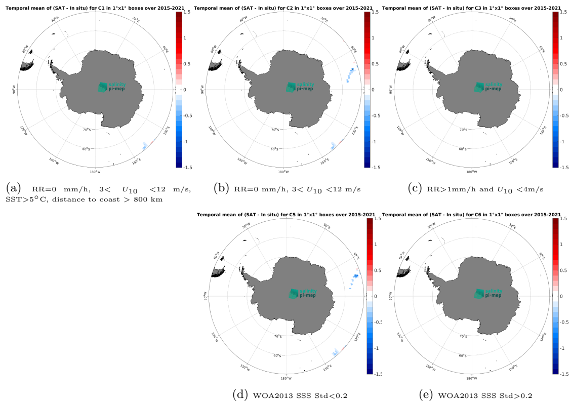
Figure 14: Temporal mean gridded over spatial boxes of size 1^\circ \times 1^\circ of \Delta SSS (SMOS SSS L3 Southern Ocean v1 - 9-Day running mean (BEC) - TSG (GOSUD-Research-vessel)) for 5 different subdatasets corresponding to:RR=0 mm/h, 3 < U_{10} < 12 m/s, SST > 5^\circ\text{C} , distance to coast > 800 km (a), RR=0 mm/h, 3 < U_{10} < 12 m/s (b), RR > 1 mm/h and U_{10} < 4 m/s (c), WOA2013 SSS Std < 0.2 (d), WOA2013 SSS Std > 0.2 (e).
