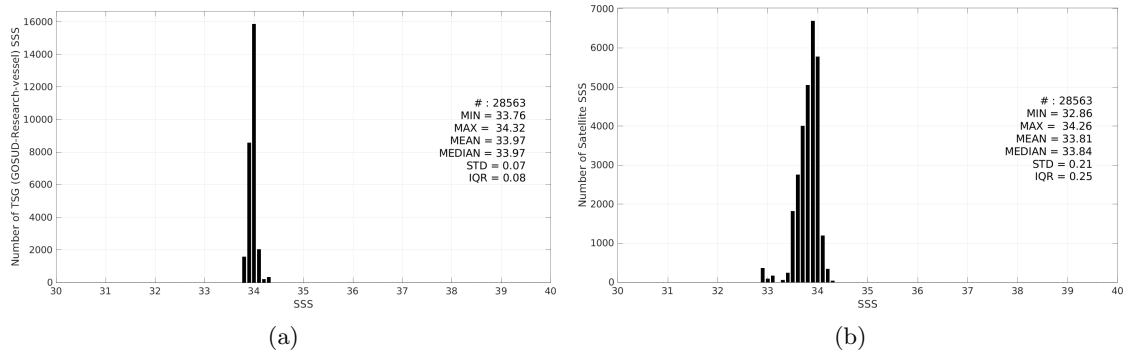
Figure 3: Histograms of SSS from TSG (GOSUD-Research-vessel) (a) and SMOS SSS L3 Southern Ocean v1 - 9-Day running mean (BEC) (b) considering all match-up pairs per bins of 0.1 over the Southern Ocean Pi-MEP region and for the full satellite product period.
