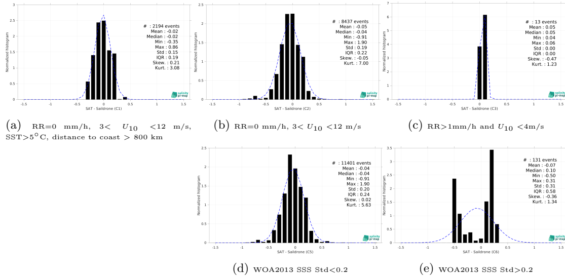
Figure 15: Normalized histogram of \Delta SSS (SMOS SSS L3 Southern Ocean v1 - 9-Day running mean (BEC) - Saildrone) for 5 different subdatasets corresponding to: RR=0 mm/h, 3 < U_{10} < 12 m/s, SST > 5°C, distance to coast > 800 km (a), RR=0 mm/h, 3 < U_{10} < 12 m/s (b), RR > 1mm/h and U_{10} < 4 m/s (c), WOA2013 SSS Std < 0.2 (d), WOA2013 SSS Std > 0.2 (e).
