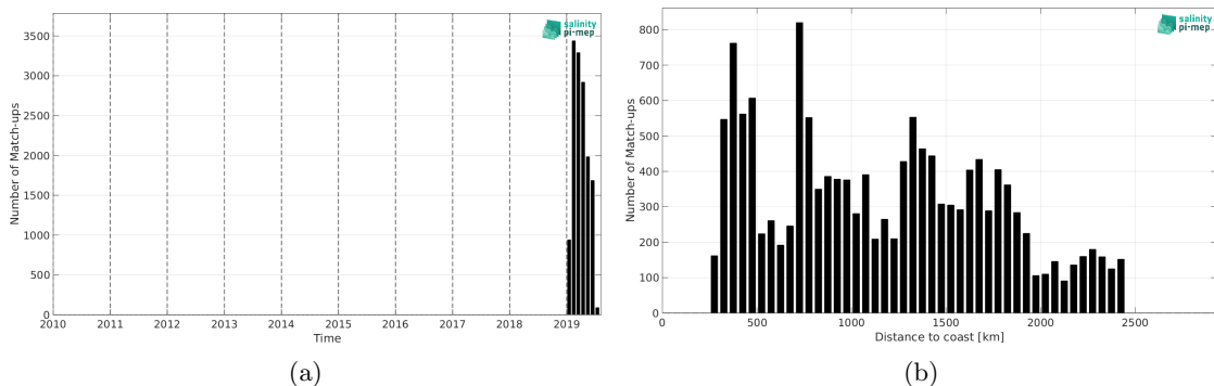
Figure 2: Number of match-ups between Saildrone and SMOS SSS L3 Southern Ocean v1 - 9-Day running mean (BEC) SSS as a function of time (a) and as function of the distance to coast (b) over the Southern Ocean Pi-MEP region and for the full satellite product period.
