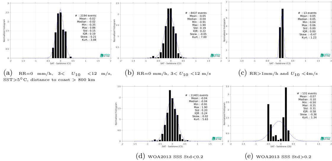
Figure 15: Normalized histogram of \Delta SSS (SMOS SSS L3 Southern Ocean v1 - 9-Day running mean (BEC) - Saldrone) for 5 different subdatasets corresponding to: RR=0 mm/h, 3 < U_{10} < 12 m/s, SST > 5°C, distance to coast > 800 km (a), RR=0 mm/h, 3 < U_{10} < 12 m/s (b), RR > 1mm/h and U_{10} < 4 m/s (c), WOA2013 SSS Std < 0.2 (d), WOA2013 SSS Std > 0.2 (e).
