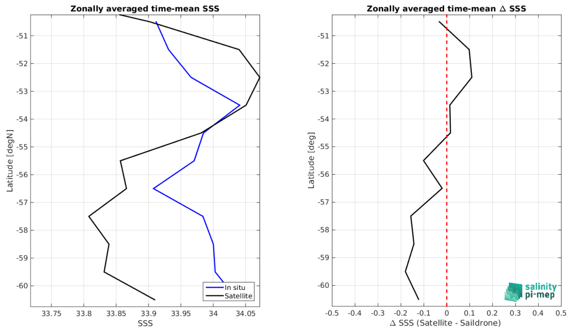
Figure 9: Left panel: Zonal mean SSS from SMOS SSS L3 Southern Ocean v1 - 9-Day running mean (BEC) satellite product (black) and from Saildrone (blue). Right panel: Zonal mean of \Delta SSS (Satellite - Saildrone) for all the collected Pi-MEP match-up pairs estimated over the full satellite product period.
