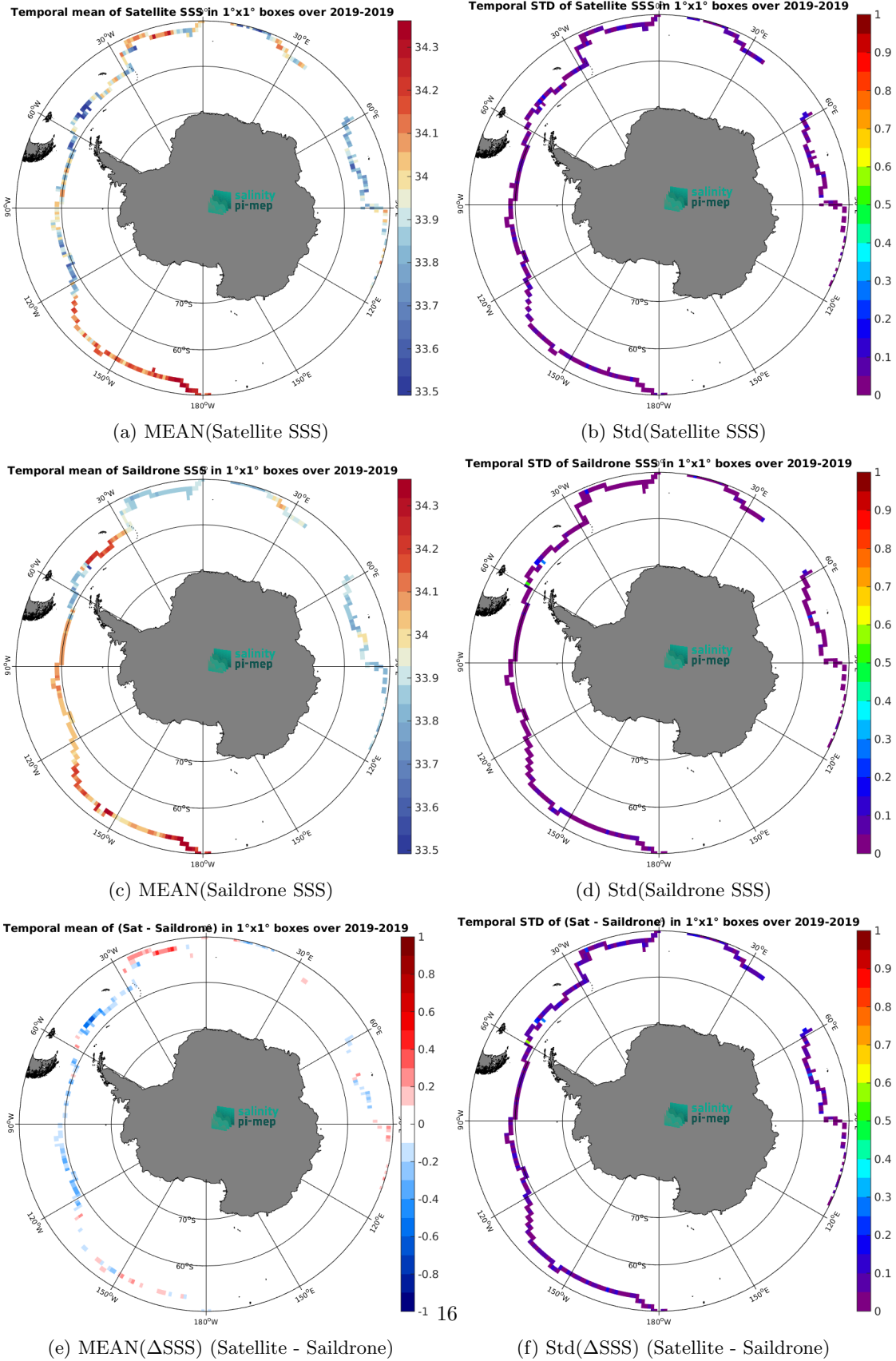
Figure 7: Temporal mean (left) and Std (right) of SSS from SMOS SSS L3 Southern Ocean v1 - 9-Day running mean (BEC) (top), Saildrone (middle), and of \Delta SSS (Satellite - Saildrone). Only match-up pairs are used to generate these maps.
