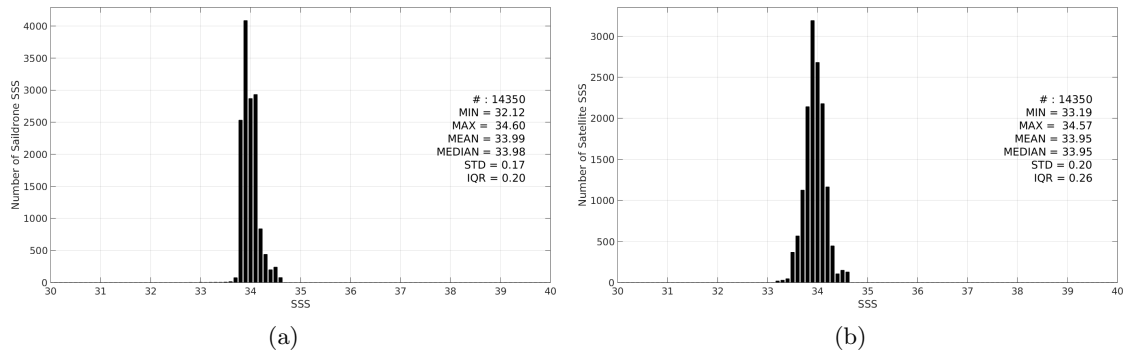
Figure 3: Histograms of SSS from Saildrone (a) and SMOS SSS L3 Southern Ocean v1 - 9-Day running mean (BEC) (b) considering all match-up pairs per bins of 0.1 over the Southern Ocean Pi-MEP region and for the full satellite product period.
