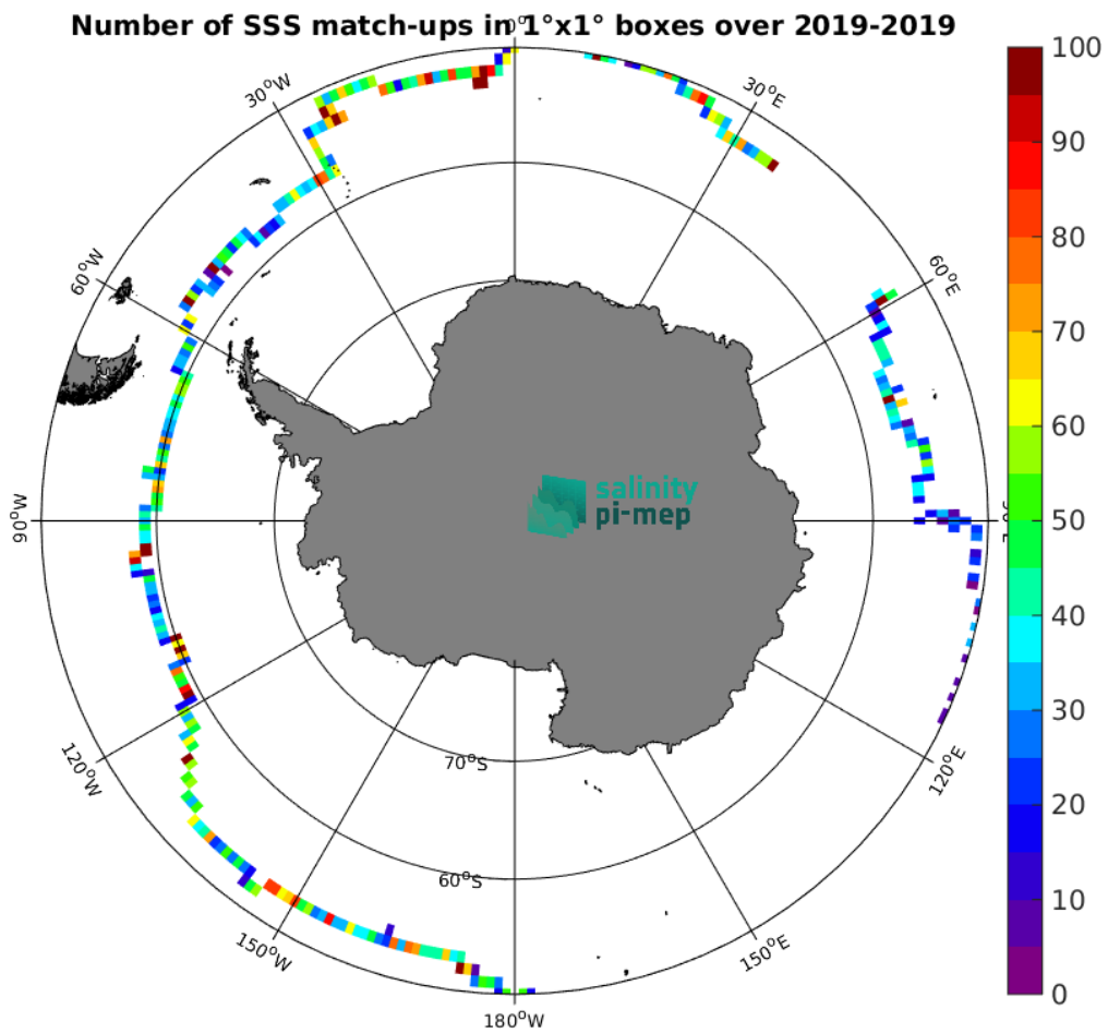
Figure 5: Number of SSS match-ups between Saildrone SSS and the SMOS SSS L3 Southern Ocean v1 - 9-Day running mean (BEC) SSS product for the Southern Ocean Pi-MEP region over 1^\circ \times 1^\circ boxes and for the full satellite product period.
