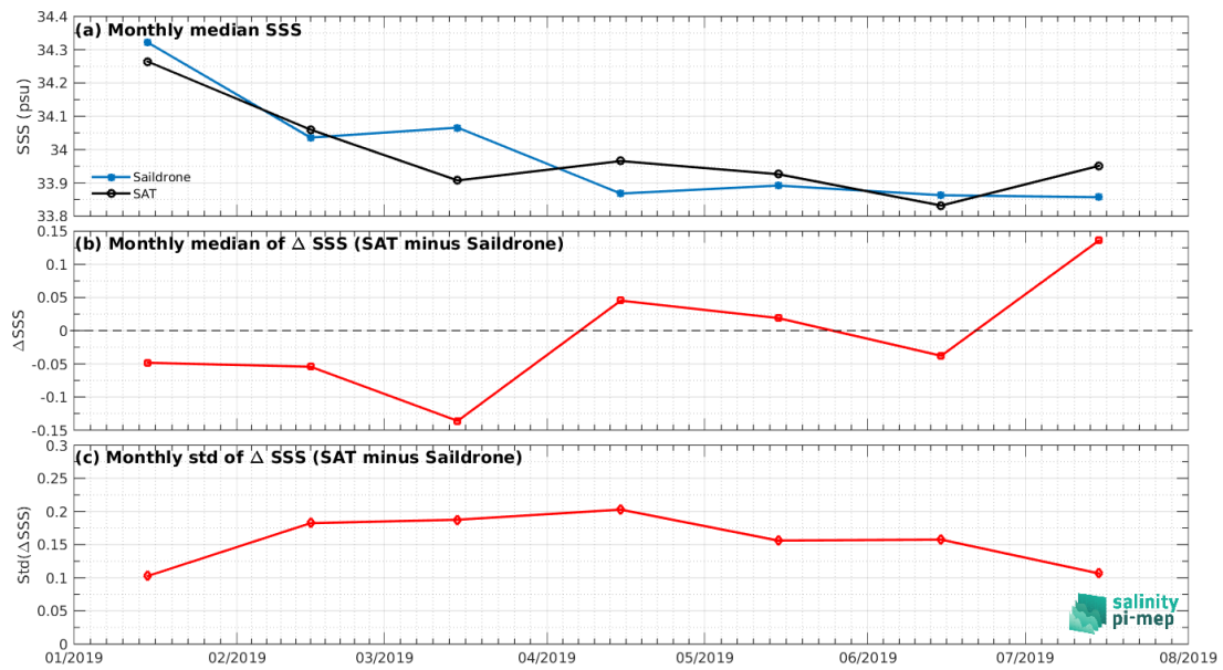
Figure 8: Time series of the monthly median SSS (top), median of \Delta SSS (Satellite - Sairdrone) and Std of \Delta SSS (Satellite - Sairdrone) over the Southern Ocean Pi-MEP region considering all match-ups collected by the Pi-MEP.
