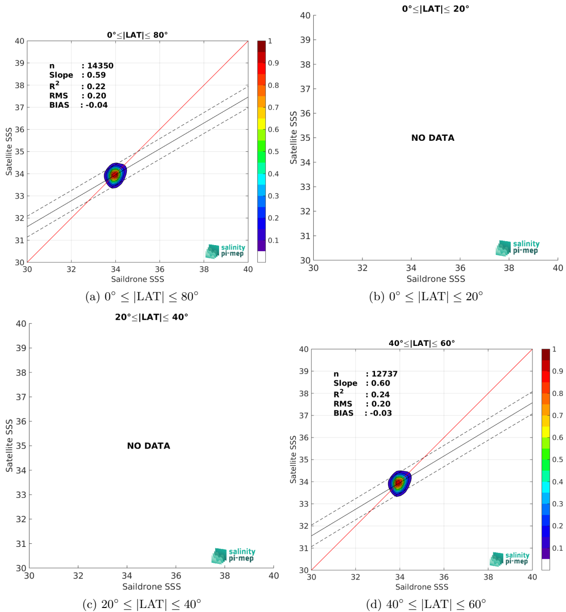
Figure 10: Contour maps of the concentration of SMOS SSS L3 Southern Ocean v1 - 9-Day running mean (BEC) SSS (y-axis) versus Sailldrone SSS (x-axis) at match-up pairs for different latitude bands. For each plot, the red line shows x=y . The black thin and dashed lines indicate a linear fit through the data cloud and the \pm 95\% confidence levels, respectively. The number match-up pairs n , the slope and R^2 coefficient of the linear fit, the root mean square (RMS) and the mean bias between satellite and in situ data are indicated for each latitude band in each plots.
