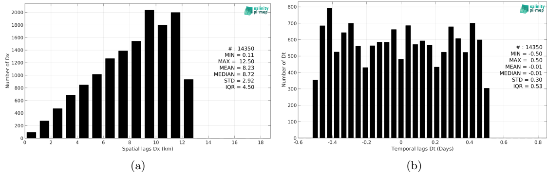
Figure 6: Histograms of the spatial (a) and temporal (b) lags between the location/time of the Saildrone measurement and the date of the corresponding SMOS SSS L3 Southern Ocean v1 - 9-Day running mean (BEC) SSS pixel.
