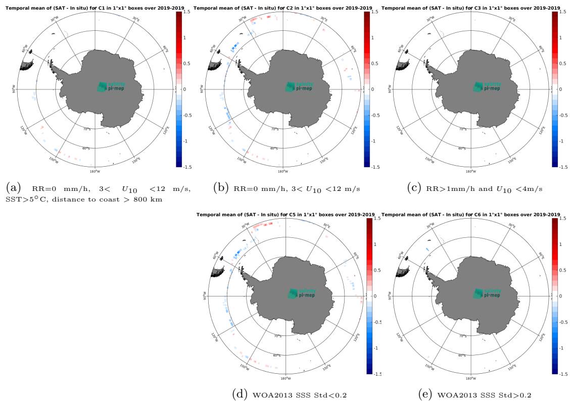
Figure 14: Temporal mean gridded over spatial boxes of size 1^\circ \times 1^\circ of \Delta SSS (SMOS SSS L3 Southern Ocean v1 - 9-Day running mean (BEC) - Saifdrone) for 5 different subdatasets corresponding to:RR=0 mm/h, 3 < U_{10} < 12 m/s, SST >5^\circ C, distance to coast > 800 km (a), RR=0 mm/h, 3 < U_{10} < 12 m/s (b), RR >1 mm/h and U_{10} < 4 m/s (c), WOA2013 SSS Std <0.2 (d), WOA2013 SSS Std >0.2 (e).
