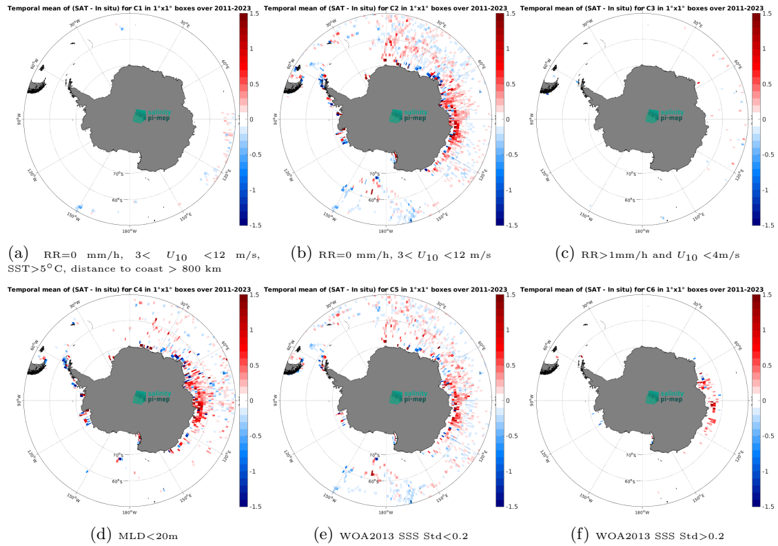
Figure 14: Temporal mean gridded over spatial boxes of size 1^\circ \times 1^\circ of \Delta\text{SSS} (SMOS SSS L3 Southern Ocean v1 - 9-Day running mean (BEC) - Marine mammals) for 6 different subdatasets corresponding to:RR=0 mm/h, 3 < U_{10} < 12 m/s, SST>5°C, distance to coast > 800 km (a), RR=0 mm/h, 3 < U_{10} < 12 m/s (b), RR>1mm/h and U_{10} < 4 m/s (c),MLD<20m (d),WOA2013 SSS Std<0.2 (e),WOA2013 SSS Std>0.2 (f).
