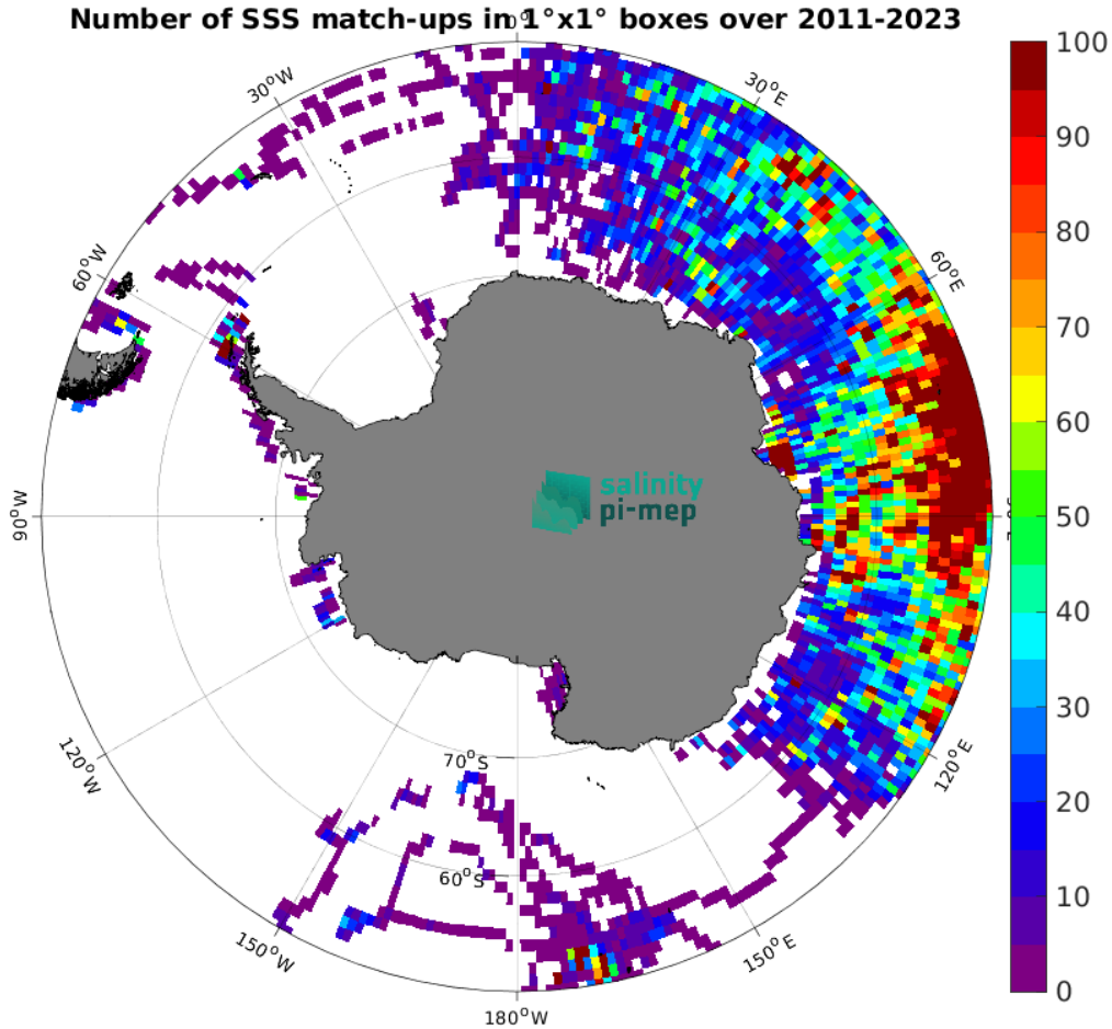
Figure 5: Number of SSS match-ups between Marine mammals SSS and the SMOS SSS L3 Southern Ocean v1 - 9-Day running mean (BEC) SSS product for the Southern Ocean Pi-MEP region over 1^\circ \times 1^\circ boxes and for the full satellite product period.
