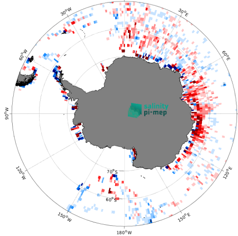
(e) MEAN( \Delta SSS) (Satellite - Marine mammals) 16
