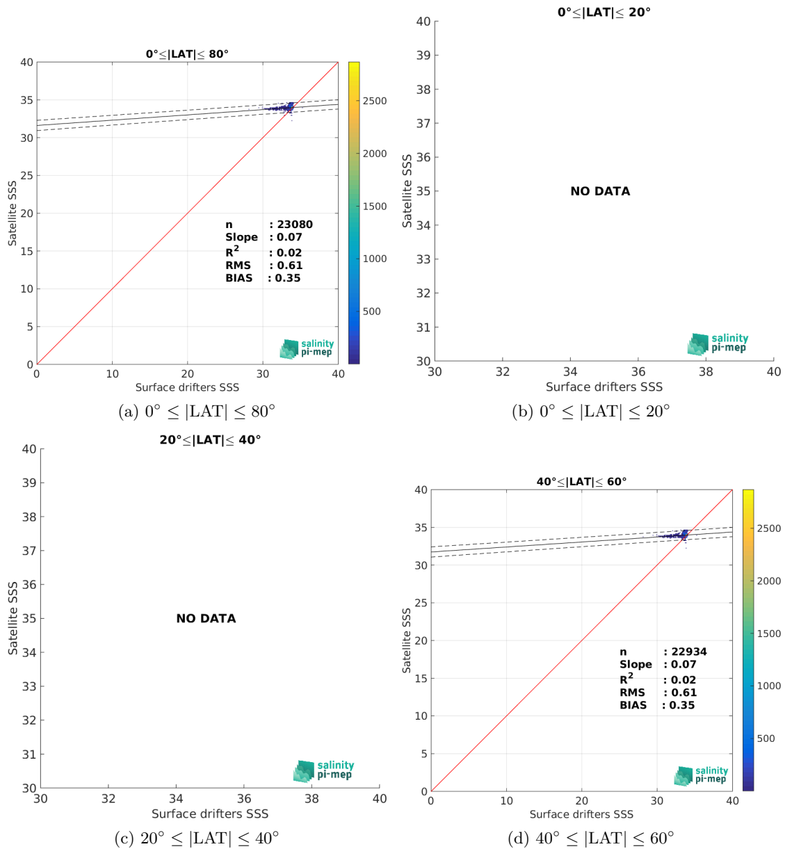
Figure 9: Contour maps of the concentration of SMOS SSS L3 Southern Ocean v1 - 9-Day running mean (BEC) SSS (y-axis) versus Surface drifters SSS (x-axis) at match-up pairs for different latitude bands. For each plot, the red line shows x=y . The black thin and dashed lines indicate a linear fit through the data cloud and the \pm 95\% confidence levels, respectively. The number match-up pairs n , the slope and R^2 coefficient of the linear fit, the root mean square (RMS) and the mean bias between satellite and in situ data are indicated for each latitude band in each plots.
