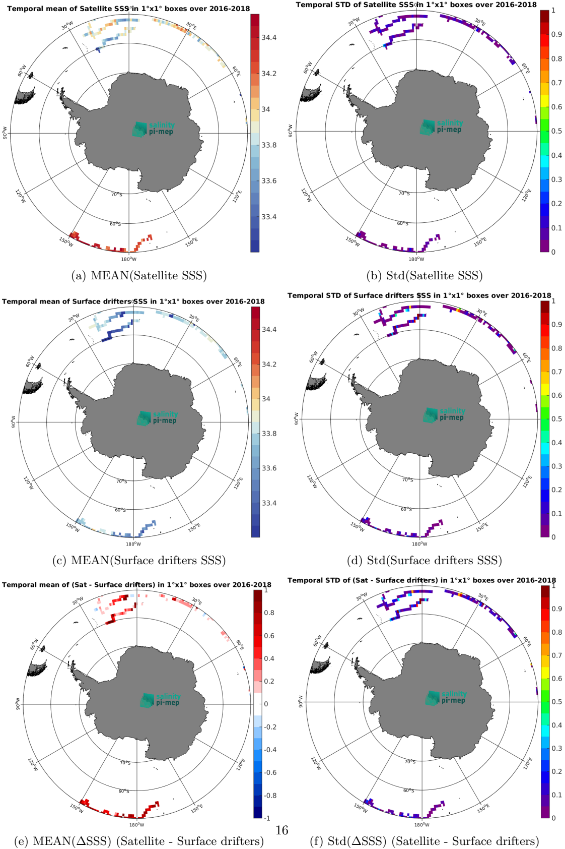
Figure 6: Temporal mean (left) and Std (right) of SSS from SMOS SSS L3 Southern Ocean v1 - 9-Day running mean (BEC) (top), Surface drifters (middle), and of \Delta SSS (Satellite - Surface drifters). Only match-up pairs are used to generate these maps.
