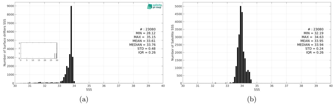
Figure 3: Histograms of SSS from Surface drifters (a) and SMOS SSS L3 Southern Ocean v1 - 9-Day running mean (BEC) (b) considering all match-up pairs per bins of 0.1 over the Southern Ocean Pi-MEP region and for the full satellite product period.
