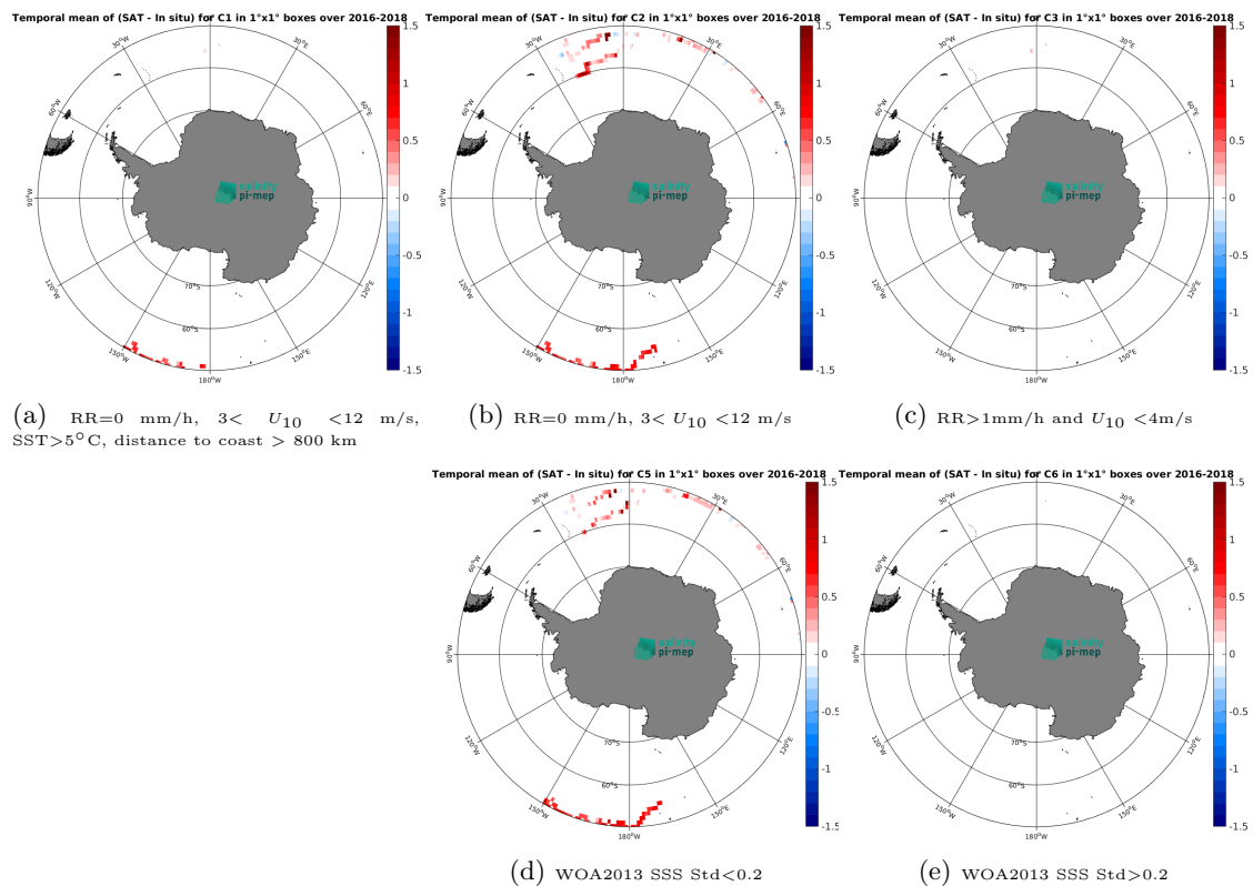
Figure 13: Temporal mean gridded over spatial boxes of size 1^\circ \times 1^\circ of \Delta SSS (SMOS SSS L3 Southern Ocean v1 - 9-Day running mean (BEC) - Surface drifters) for 5 different subdatasets corresponding to:RR=0 mm/h, 3 < U_{10} < 12 m/s, SST >5^\circ C, distance to coast > 800 km (a), RR=0 mm/h, 3 < U_{10} < 12 m/s (b), RR >1 mm/h and U_{10} < 4 m/s (c), WOA2013 SSS Std <0.2 (d), WOA2013 SSS Std >0.2 (e).
