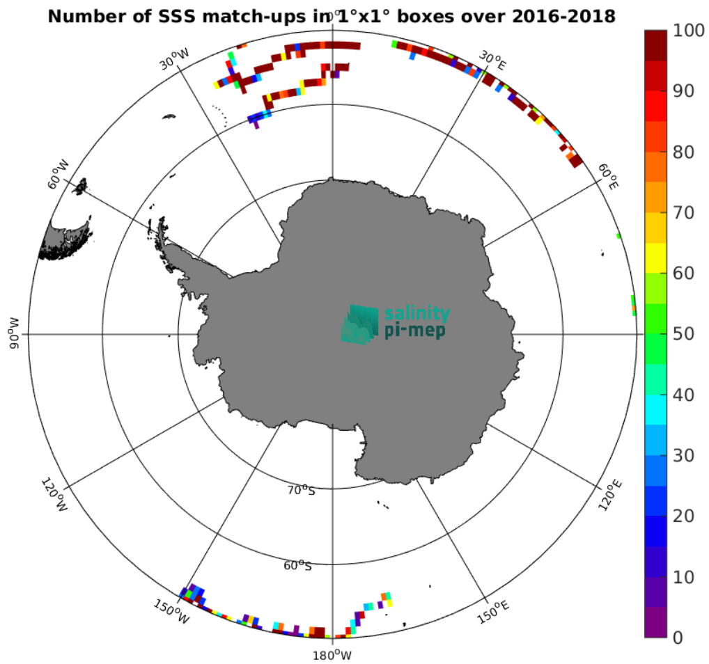
Figure 4: Number of SSS match-ups between Surface drifters SSS and the SMOS SSS L3 Southern Ocean v1 - 9-Day running mean (BEC) SSS product for the Southern Ocean Pi-MEP region over 1^\circ \times 1^\circ boxes and for the full satellite product period.
