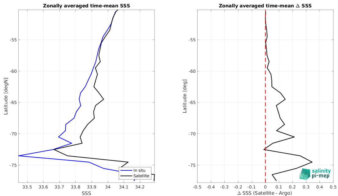
Figure 9: Left panel: Zonal mean SSS from SMOS SSS L3 Southern Ocean v1 - 9-Day running mean (BEC) satellite product (black) and from Argo (blue). Right panel: Zonal mean of \Delta SSS (Satellite - Argo) for all the collected Pi-MEP match-up pairs estimated over the full satellite product period.
