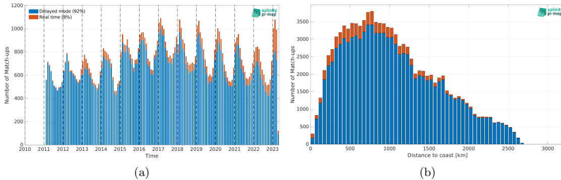
Figure 2: Number of match-ups between Argo and SMOS SSS L3 Southern Ocean v1 - 9-Day running mean (BEC) SSS as a function of time (a) and as function of the distance to coast (b) over the Southern Ocean Pi-MEP region and for the full satellite product period.
