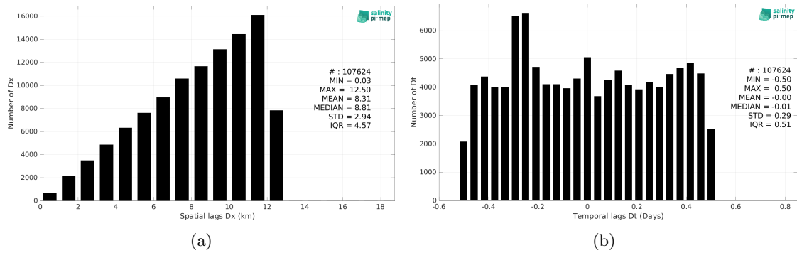
Figure 6: Histograms of the spatial (a) and temporal (b) lags between the location/time of the Argo measurement and the date of the corresponding SMOS SSS L3 Southern Ocean v1 - 9-Day running mean (BEC) SSS pixel.
