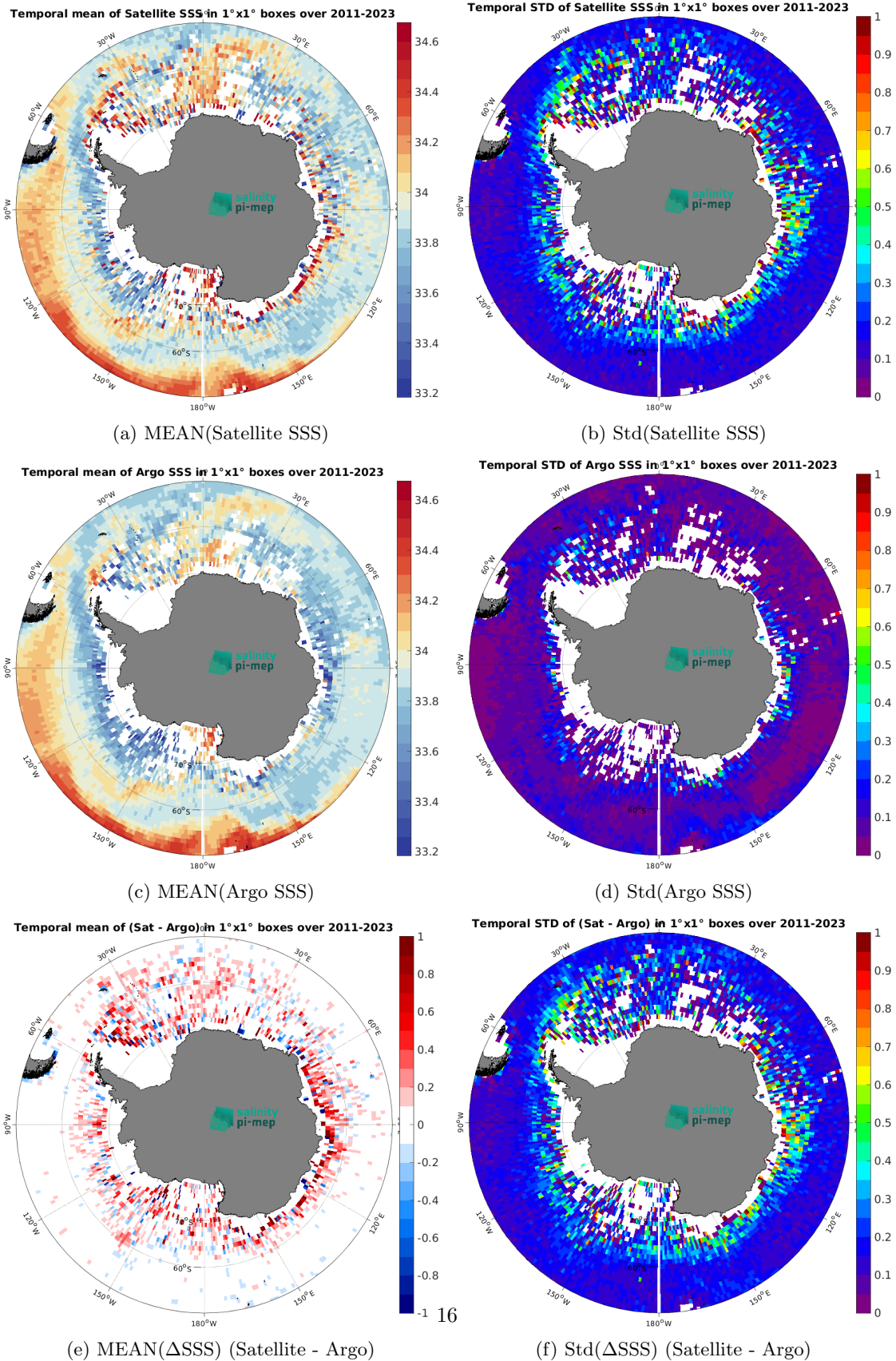
Figure 7: Temporal mean (left) and Std (right) of SSS from SMOS SSS L3 Southern Ocean v1 - 9-Day running mean (BEC) (top), Argo (middle), and of \Delta SSS (Satellite - Argo). Only match-up pairs are used to generate these maps.
