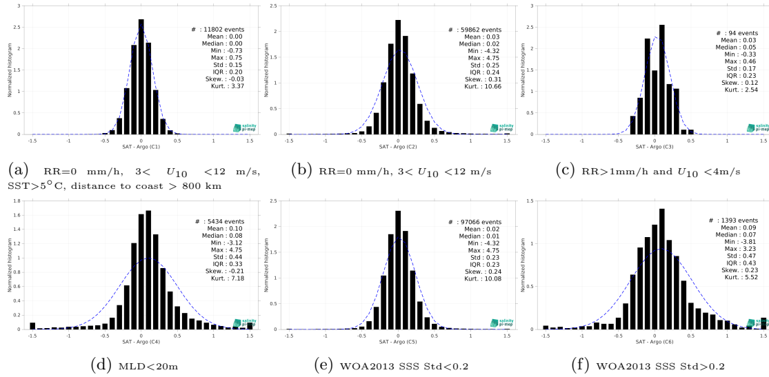
Figure 15: Normalized histogram of \Delta SSS (SMOS SSS L3 Southern Ocean v1 - 9-Day running mean (BEC) - Argo) for 6 different subdatasets corresponding to: RR=0 mm/h, 3 < U_{10} < 12 m/s, SST>5°C, distance to coast > 800 km (a), RR=0 mm/h, 3 < U_{10} < 12 m/s (b), RR>1mm/h and U_{10} < 4 m/s (c), MLD<20m (d), WOA2013 SSS Std<0.2 (e), WOA2013 SSS Std>0.2 (f).
