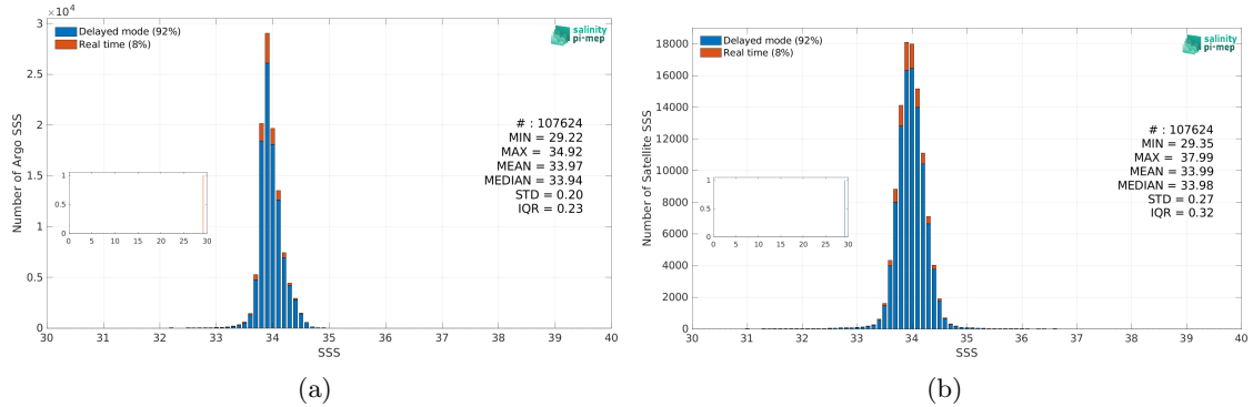
Figure 3: Histograms of SSS from Argo (a) and SMOS SSS L3 Southern Ocean v1 - 9-Day running mean (BEC) (b) considering all match-up pairs per bins of 0.1 over the Southern Ocean Pi-MEP region and for the full satellite product period.
