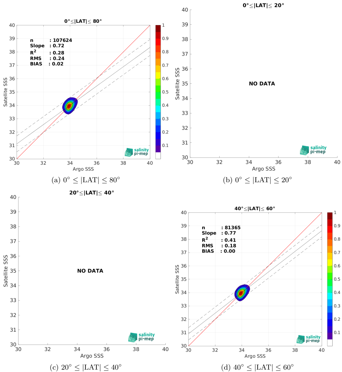
Figure 10: Contour maps of the concentration of SMOS SSS L3 Southern Ocean v1 - 9-Day running mean (BEC) SSS (y-axis) versus Argo SSS (x-axis) at match-up pairs for different latitude bands. For each plot, the red line shows x=y . The black thin and dashed lines indicate a linear fit through the data cloud and the \pm 95\% confidence levels, respectively. The number match-up pairs n , the slope and R^2 coefficient of the linear fit, the root mean square (RMS) and the mean bias between satellite and in situ data are indicated for each latitude band in each plots.
