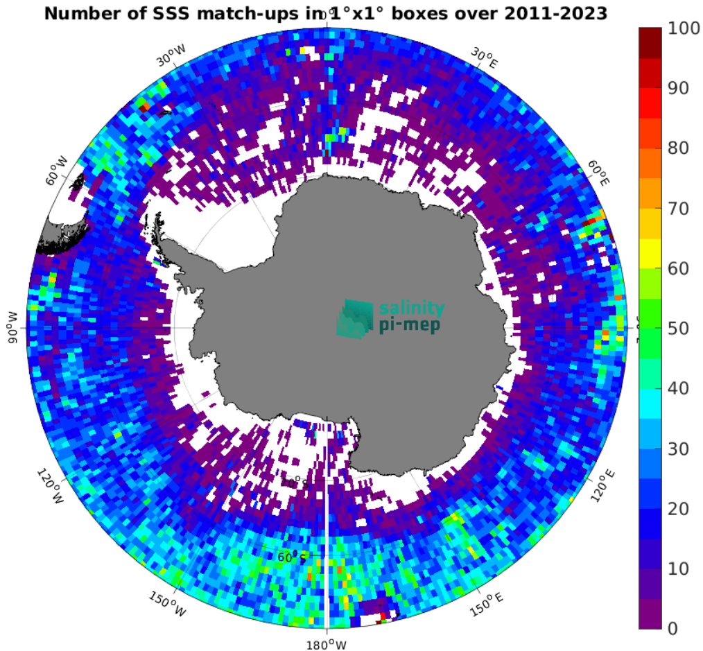
Figure 5: Number of SSS match-ups between Argo SSS and the SMOS SSS L3 Southern Ocean v1 - 9-Day running mean (BEC) SSS product for the Southern Ocean Pi-MEP region over 1^\circ \times 1^\circ boxes and for the full satellite product period.
