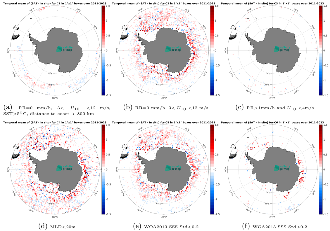
Figure 14: Temporal mean gridded over spatial boxes of size 1^\circ \times 1^\circ of \Delta\text{SSS} (SMOS SSS L3 Southern Ocean v1 - 9-Day running mean (BEC) - Argo) for 6 different subdatasets corresponding to:RR=0 mm/h, 3 < U_{10} < 12 m/s, SST>5°C, distance to coast > 800 km (a), RR=0 mm/h, 3 < U_{10} < 12 m/s (b), RR>1mm/h and U_{10} < 4 m/s (c),MLD<20m (d),WOA2013 SSS Std<0.2 (e),WOA2013 SSS Std>0.2 (f).
