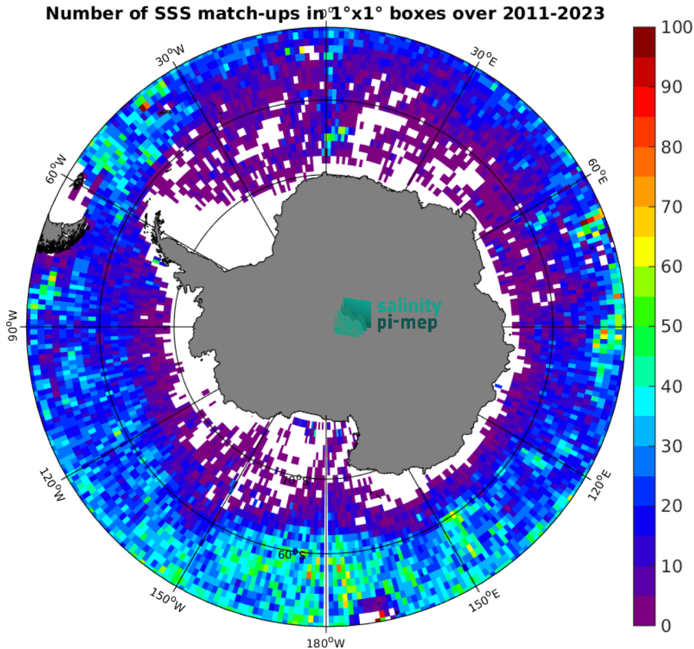
Figure 5: Number of SSS match-ups between Argo SSS and the SMOS SSS L3 Southern Ocean v1 - 9-Day running mean (BEC) SSS product for the Southern Ocean Pi-MEP region over 1^\circ \times 1^\circ boxes and for the full satellite product period.
