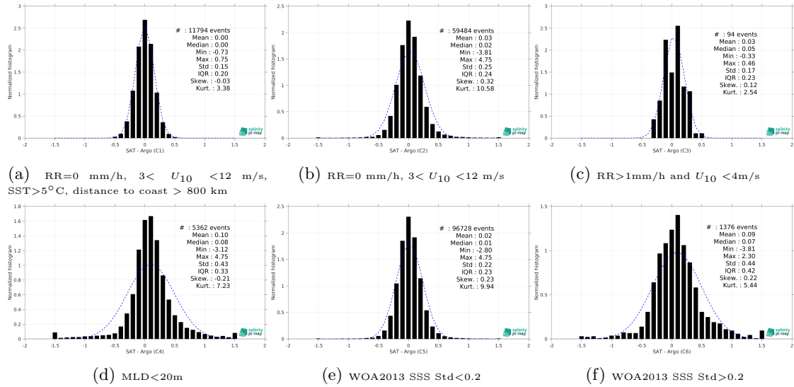
Figure 15: Normalized histogram of \Delta\text{SSS} (SMOS SSS L3 Southern Ocean v1 - 9-Day running mean (BEC) - Argo) for 6 different subdatasets corresponding to: RR=0 mm/h, 3 < U_{10} < 12 m/s, SST>5°C, distance to coast > 800 km (a), RR=0 mm/h, 3 < U_{10} < 12 m/s (b), RR>1mm/h and U_{10} < 4 m/s (c), MLD<20m (d), WOA2013 SSS Std<0.2 (e), WOA2013 SSS Std>0.2 (f).
