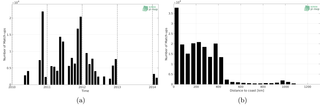
Figure 1: Number of match-ups between TSG-SAMOS and SMOS-L3-BEC-OA-V1-9DAYS-0.25DEG SSS as a function of time (a) and as function of the distance to coast (b) over the Southern Ocean Pi-MEP region and for the full satellite product period.
