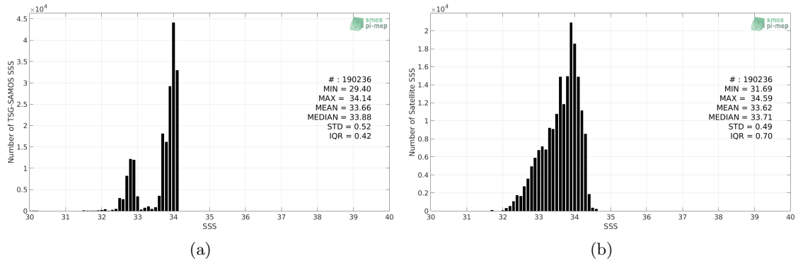
Figure 2: Histograms of SSS from TSG-SAMOS (a) and SMOS-L3-BEC-OA-V1-9DAYS-0.25DEG (b) considering all match-up pairs per bins of 0.1 over the Southern Ocean Pi-MEP region and for the full satellite product period.
