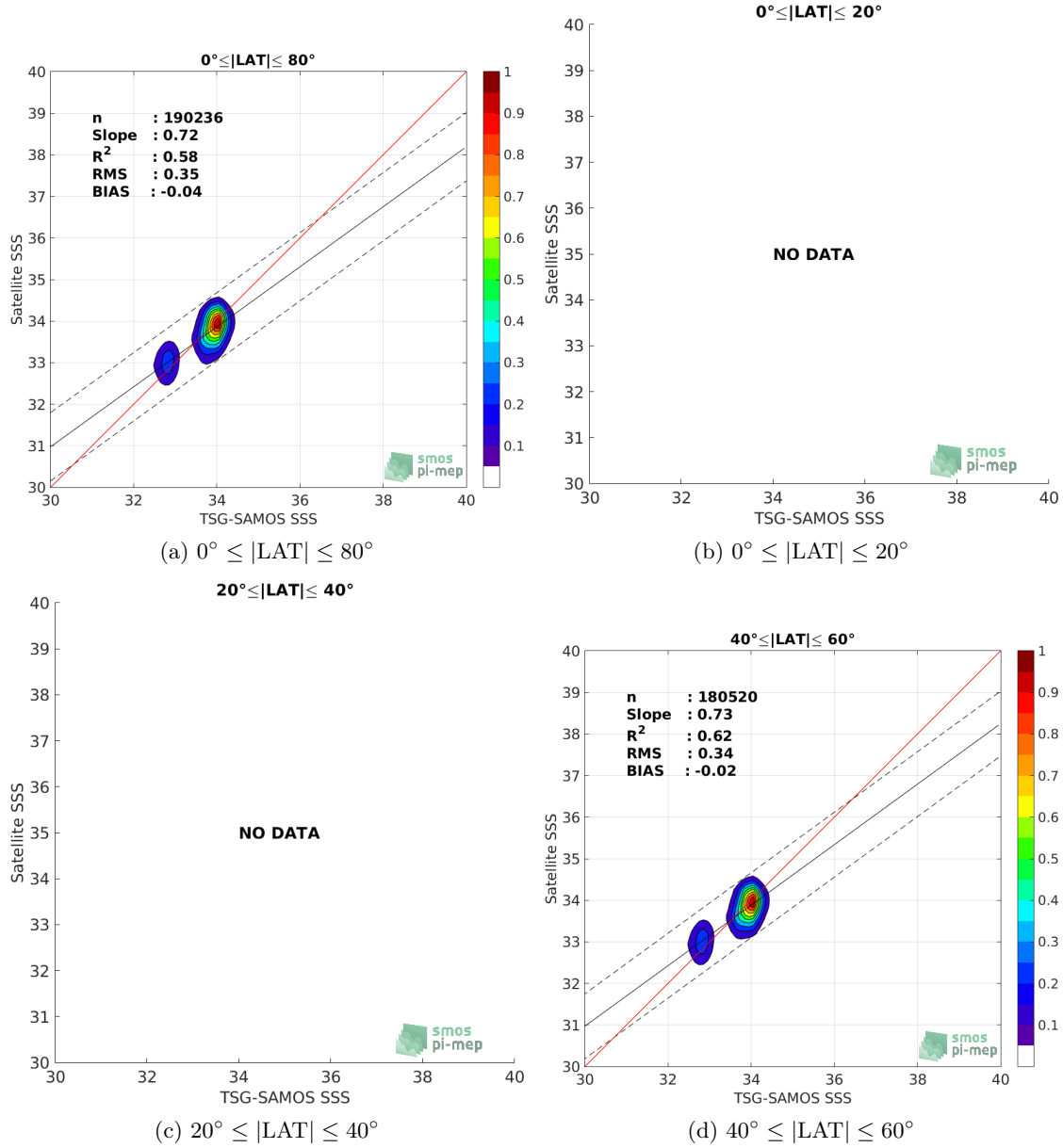
Figure 9: Contour maps of the concentration of SMOS-L3-BEC-OA-V1-9DAYS-0.25DEG SSS (y-axis) versus TSG-SAMOS SSS (x-axis) at match-up pairs for different latitude bands. For each plot, the red line shows x=y . The black thin and dashed lines indicate a linear fit through the data cloud and the \pm 95\% confidence levels, respectively. The number match-up pairs n , the slope and R^2 coefficient of the linear fit, the root mean square (RMS) and the mean bias between satellite and in situ data are indicated for each latitude band in each plots.
