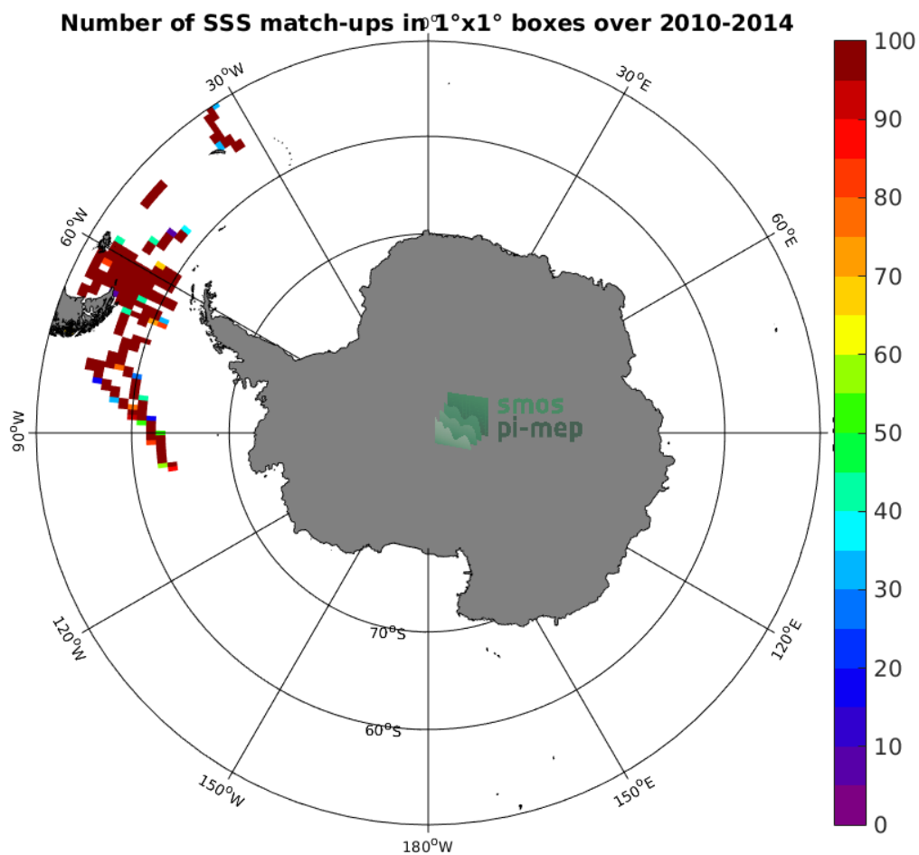
Figure 4: Number of SSS match-ups between TSG-SAMOS SSS and the SMOS-L3-BEC-OA-V1-9DAYS-0.25DEG SSS product for the Southern Ocean Pi-MEP region over 1^\circ \times 1^\circ boxes and for the full satellite product period.
