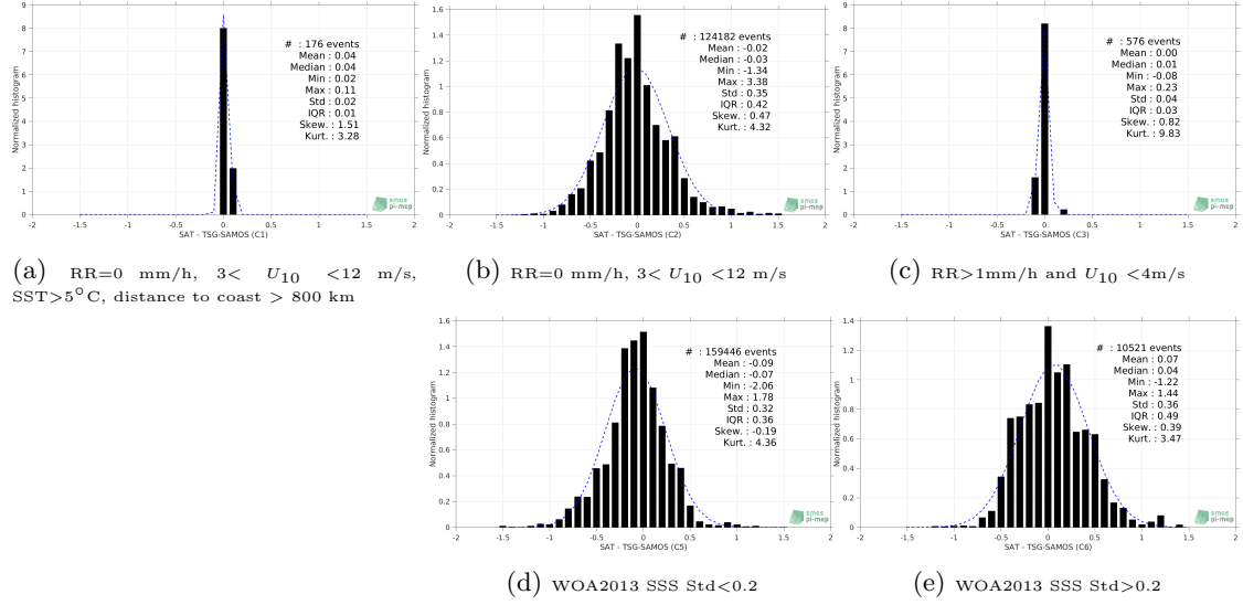
Figure 13: Normalized histogram of \Delta SSS (SMOS-L3-BEC-OA-V1-9DAYS-0.25DEG - TSG-SAMOS) for 5 different subdatasets corresponding to: RR=0 mm/h, 3 < U_{10} < 12 m/s, SST>5°C, distance to coast > 800 km (a), RR=0 mm/h, 3 < U_{10} < 12 m/s (b), RR>1mm/h and U_{10} < 4 m/s (c), WOA2013 SSS Std<0.2 (d), WOA2013 SSS Std>0.2 (e).
