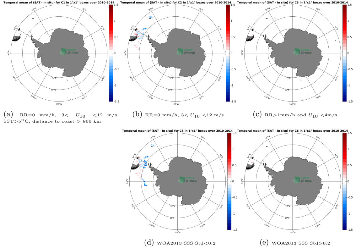
Figure 12: Temporal mean gridded over spatial boxes of size 1^\circ \times 1^\circ of \Delta SSS (SMOS-L3-BEC-OA-V1-9DAYS-0.25DEG - TSG-SAMOS) for 5 different subdatasets corresponding to:RR=0 mm/h, 3 < U_{10} < 12 m/s, SST>5°C, distance to coast > 800 km (a), RR=0 mm/h, 3 < U_{10} < 12 m/s (b), RR>1mm/h and U_{10} < 4 m/s (c), WOA2013 SSS Std<0.2 (d), WOA2013 SSS Std>0.2 (e).
