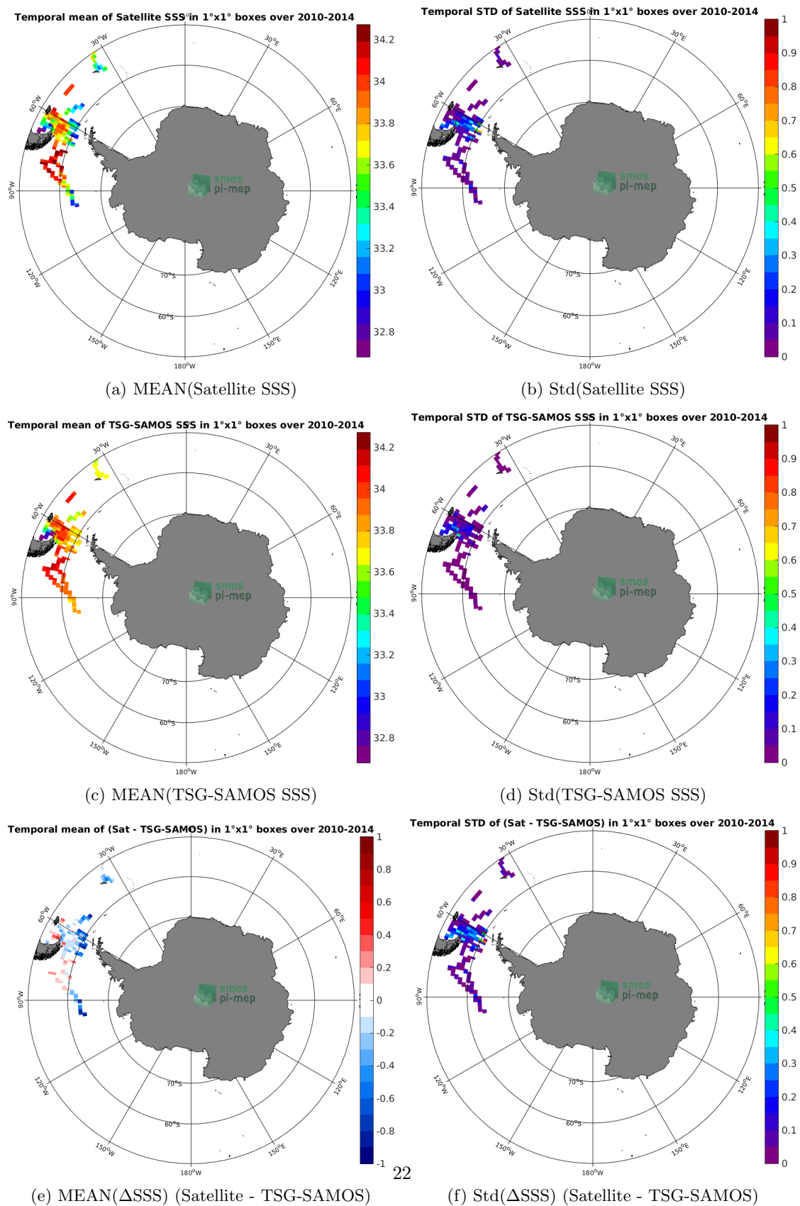
Figure 6: Temporal mean (left) and Std (right) of SSS from SMOS-L3-BEC-OA-V1-9DAYS-0.25DEG (top), TSG-SAMOS (middle), and of \Delta SSS (Satellite - TSG-SAMOS). Only match-up pairs are used to generate these maps.
