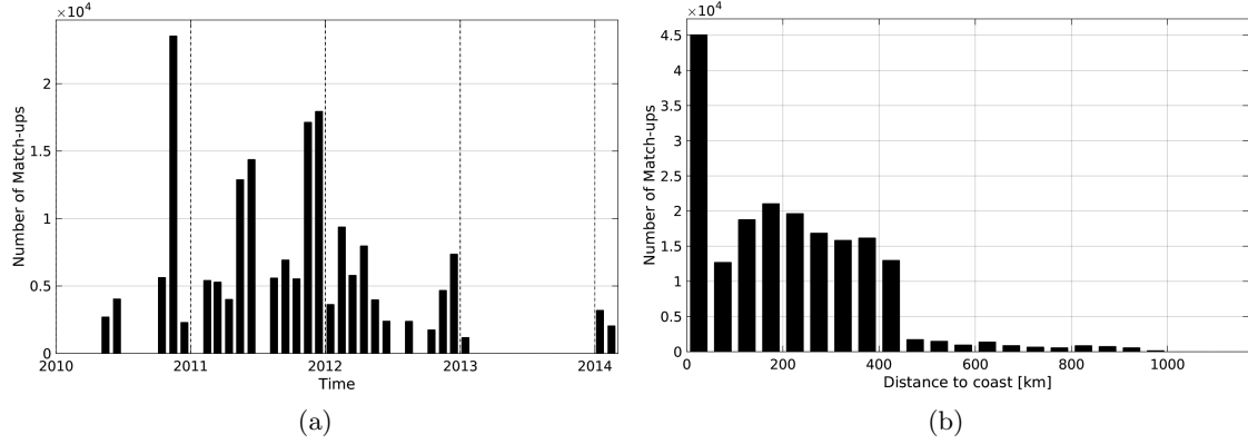
Figure 1: Number of match-ups between TSG-SAMOS and SMOS-L3-BEC-OA-V1-9DAYS-0.25DEG SSS as a function of time (a) and as function of the distance to coast (b) over the Southern Ocean Pi-MEP region and for the full satellite product period.
