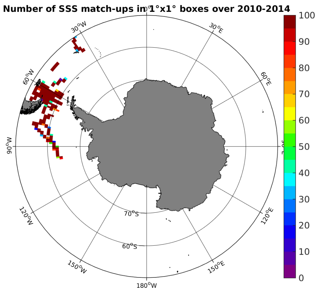
Figure 4: Number of SSS match-ups between TSG-SAMOS SSS and the SMOS-L3-BEC-OA-V1-9DAYS-0.25DEG SSS product for the Southern Ocean Pi-MEP region over 1^\circ \times 1^\circ boxes and for the full satellite product period.
