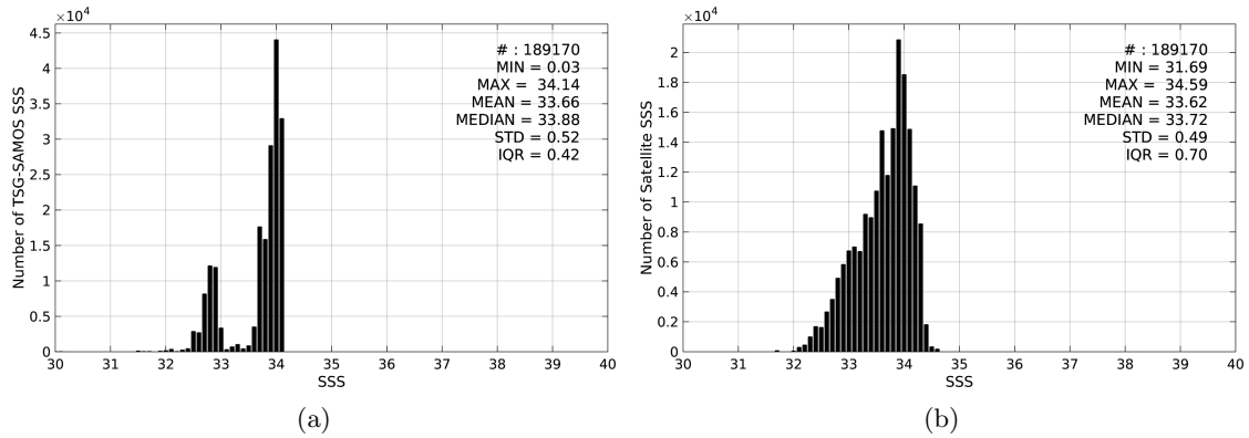
Figure 2: Histograms of SSS from TSG-SAMOS (a) and SMOS-L3-BEC-OA-V1-9DAYS-0.25DEG (b) considering all match-up pairs per bins of 0.1 over the Southern Ocean Pi-MEP region and for the full satellite product period.
