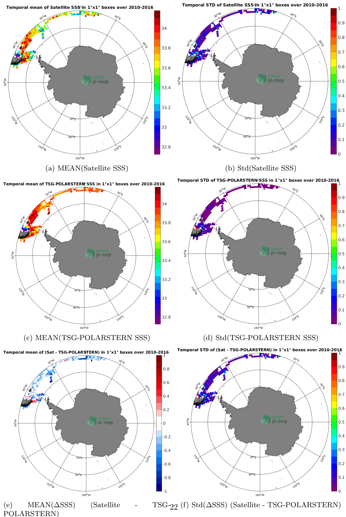
Figure 6: Temporal mean (left) and Std (right) of SSS from SMOS-L3-BEC-OA-V1-9DAYS-0.25DEG (top), TSG-POLARSTERN (middle), and of \Delta SSS (Satellite - TSG-POLARSTERN). Only match-up pairs are used to generate these maps.
