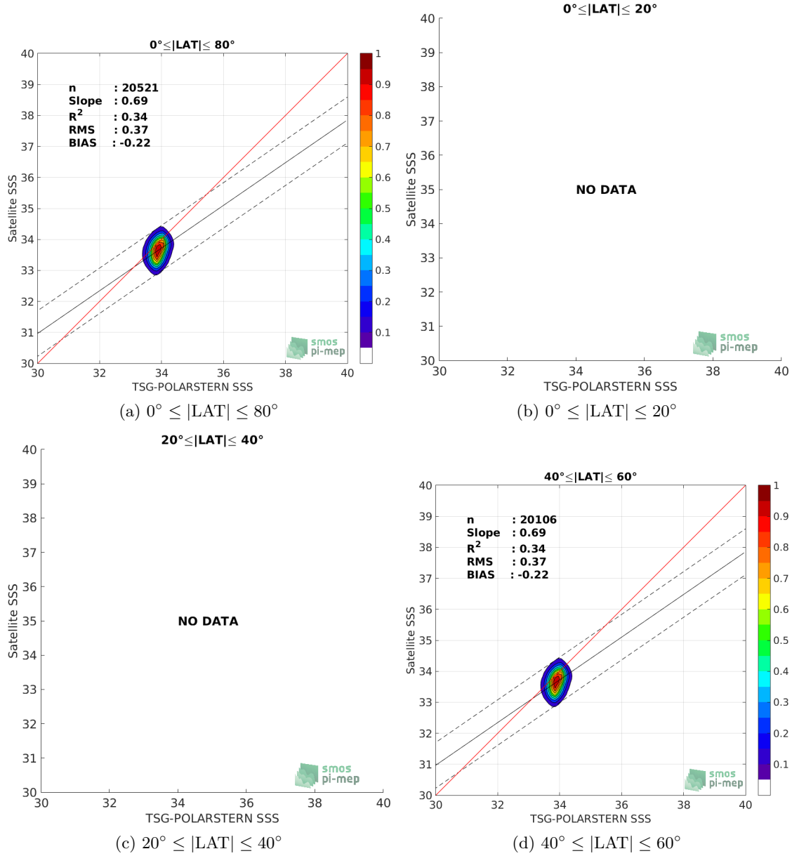
Figure 9: Contour maps of the concentration of SMOS-L3-BEC-OA-V1-9DAYS-0.25DEG SSS (y-axis) versus TSG-POLARSTERN SSS (x-axis) at match-up pairs for different latitude bands. For each plot, the red line shows x=y . The black thin and dashed lines indicate a linear fit through the data cloud and the \pm 95\% confidence levels, respectively. The number match-up pairs n , the slope and R^2 coefficient of the linear fit, the root mean square (RMS) and the mean bias between satellite and in situ data are indicated for each latitude band in each plots.
