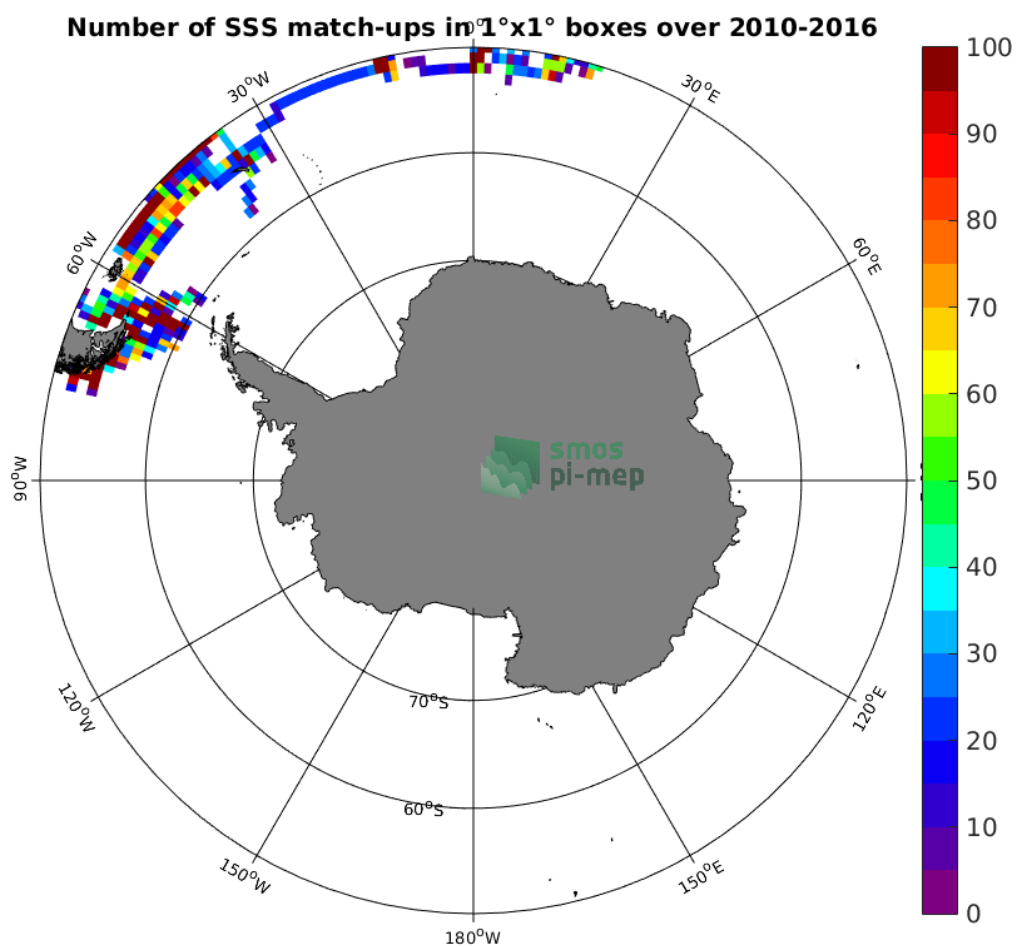
Figure 4: Number of SSS match-ups between TSG-POLARSTERN SSS and the SMOS-L3-BEC-OA-V1-9DAYS-0.25DEG SSS product for the Southern Ocean Pi-MEP region over 1^\circ \times 1^\circ boxes and for the full satellite product period.
