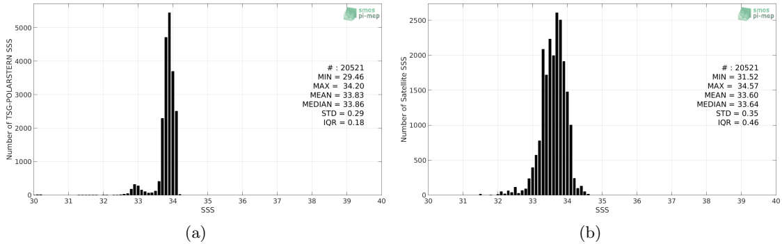
Figure 2: Histograms of SSS from TSG-POLARSTERN (a) and SMOS-L3-BEC-OA-V1-9DAYS-0.25DEG (b) considering all match-up pairs per bins of 0.1 over the Southern Ocean Pi-MEP region and for the full satellite product period.
