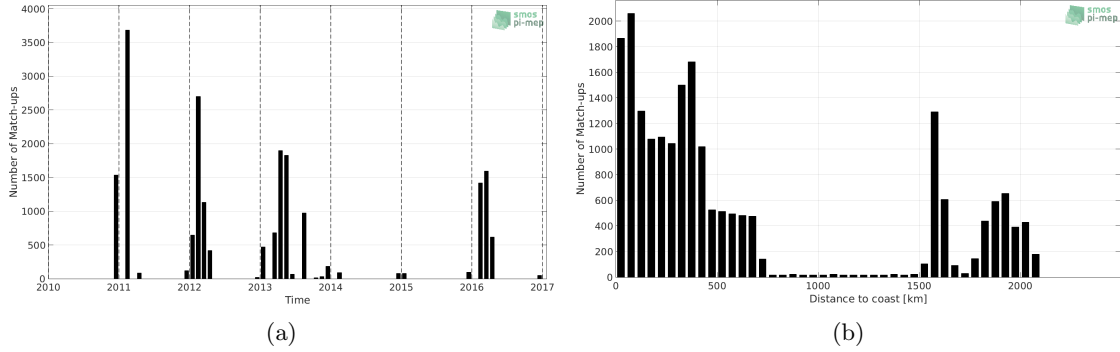
Figure 1: Number of match-ups between TSG-POLARSTERN and SMOS-L3-BEC-OA-V1-9DAYS-0.25DEG SSS as a function of time (a) and as function of the distance to coast (b) over the Southern Ocean Pi-MEP region and for the full satellite product period.
