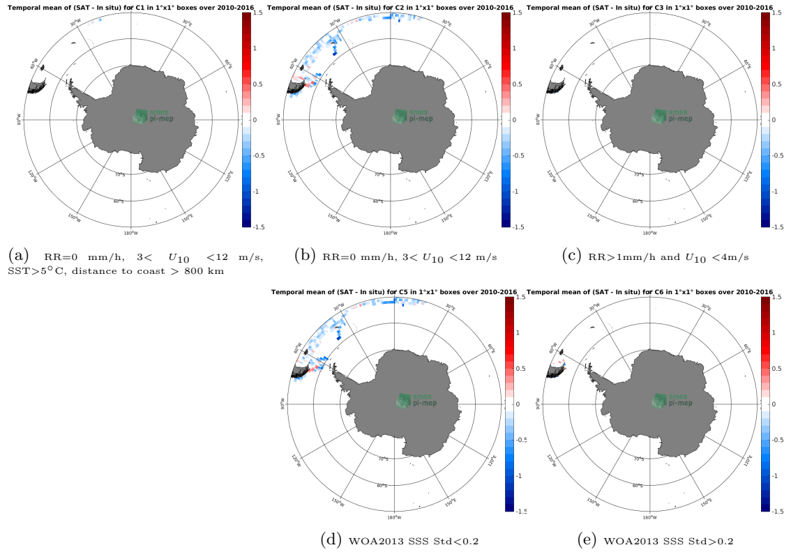
Figure 12: Temporal mean gridded over spatial boxes of size 1^\circ \times 1^\circ of \Delta SSS (SMOS-L3-BEC-OA-V1-9DAYS-0.25DEG - TSG-POLARSTERN) for 5 different subdatasets corresponding to: RR=0 mm/h, 3 < U_{10} < 12 m/s, SST >5^\circ\text{C} , distance to coast > 800 km (a), RR=0 mm/h, 3 < U_{10} < 12 m/s (b), RR >1 mm/h and U_{10} < 4 m/s (c), WOA2013 SSS Std <0.2 (d), WOA2013 SSS Std >0.2 (e).
