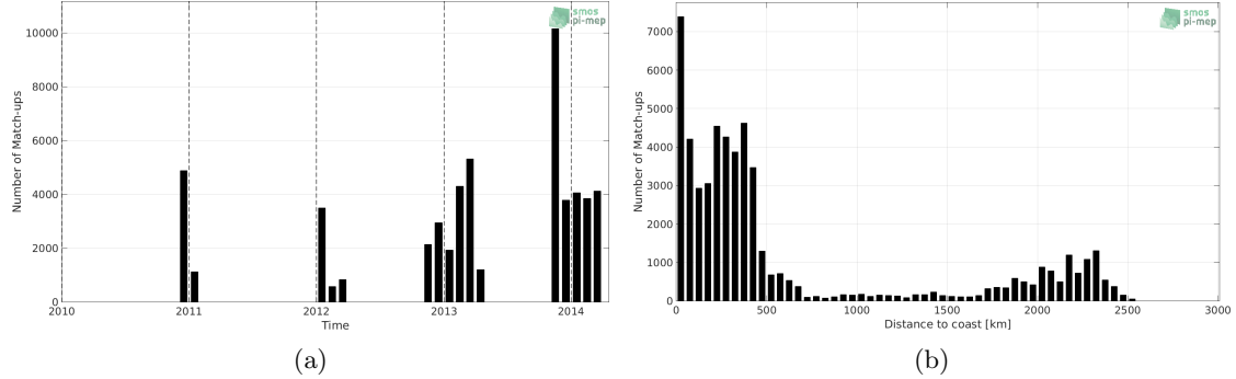
Figure 1: Number of match-ups between TSG-GOSUD-Sailing-ship and SMOS-L3-BEC-OA-V1-9DAYS-0.25DEG SSS as a function of time (a) and as function of the distance to coast (b) over the Southern Ocean Pi-MEP region and for the full satellite product period.
