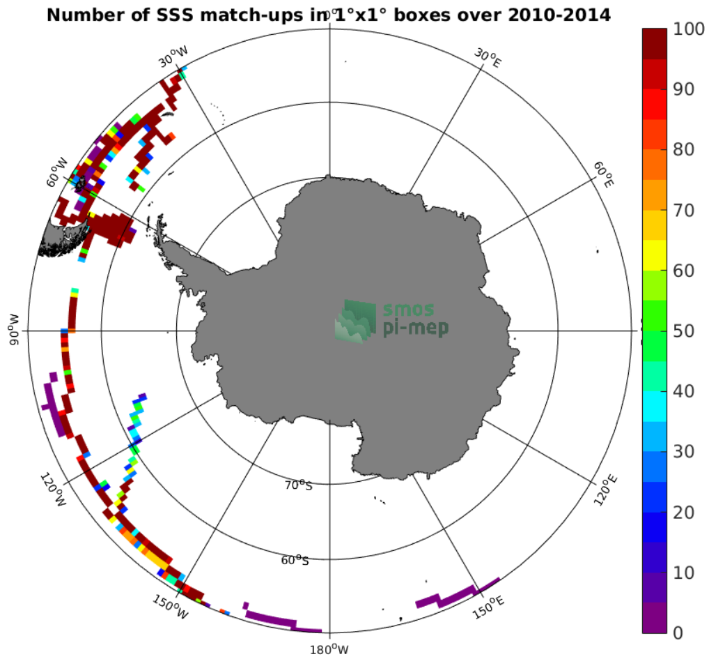
Figure 4: Number of SSS match-ups between TSG-GOSUD-Sailing-ship SSS and the SMOS-L3-BEC-OA-V1-9DAYS-0.25DEG SSS product for the Southern Ocean Pi-MEP region over 1^\circ \times 1^\circ boxes and for the full satellite product period.
