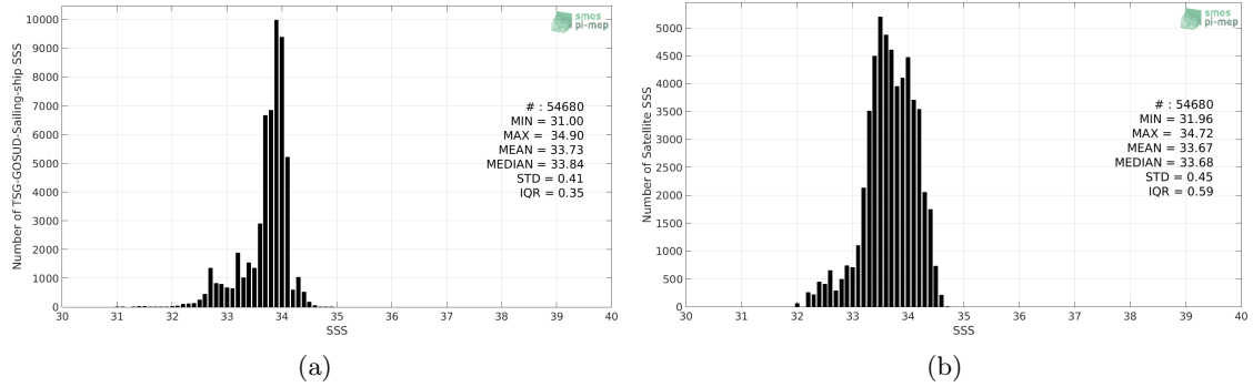
Figure 2: Histograms of SSS from TSG-GOSUD-Sailing-ship (a) and SMOS-L3-BEC-OA-V1-9DAYS-0.25DEG (b) considering all match-up pairs per bins of 0.1 over the Southern Ocean Pi-MEP region and for the full satellite product period.
