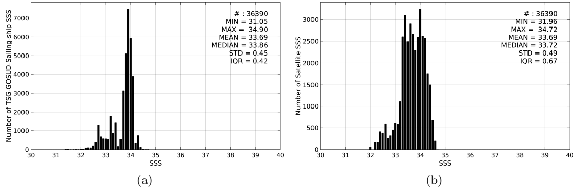
Figure 2: Histograms of SSS from TSG-GOSUD-Sailing-ship (a) and SMOS-L3-BEC-OA-V1-9DAYS-0.25DEG (b) considering all match-up pairs per bins of 0.1 over the Southern Ocean Pi-MEP region and for the full satellite product period.
