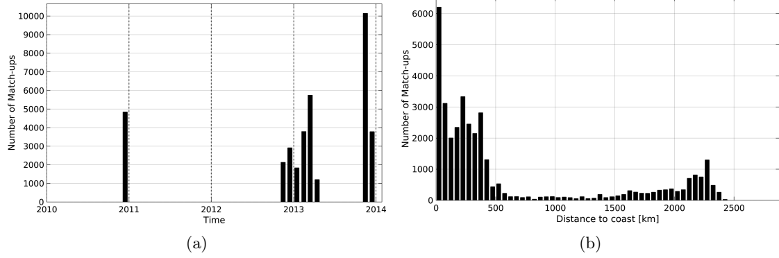
Figure 1: Number of match-ups between TSG-GOSUD-Sailing-ship and SMOS-L3-BEC-OA-V1-9DAYS-0.25DEG SSS as a function of time (a) and as function of the distance to coast (b) over the Southern Ocean Pi-MEP region and for the full satellite product period.
