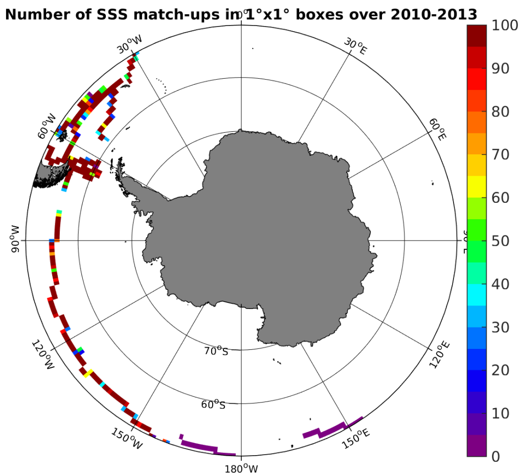
Figure 4: Number of SSS match-ups between TSG-GOSUD-Sailing-ship SSS and the SMOS-L3-BEC-OA-V1-9DAYS-0.25DEG SSS product for the Southern Ocean Pi-MEP region over 1^\circ \times 1^\circ boxes and for the full satellite product period.
