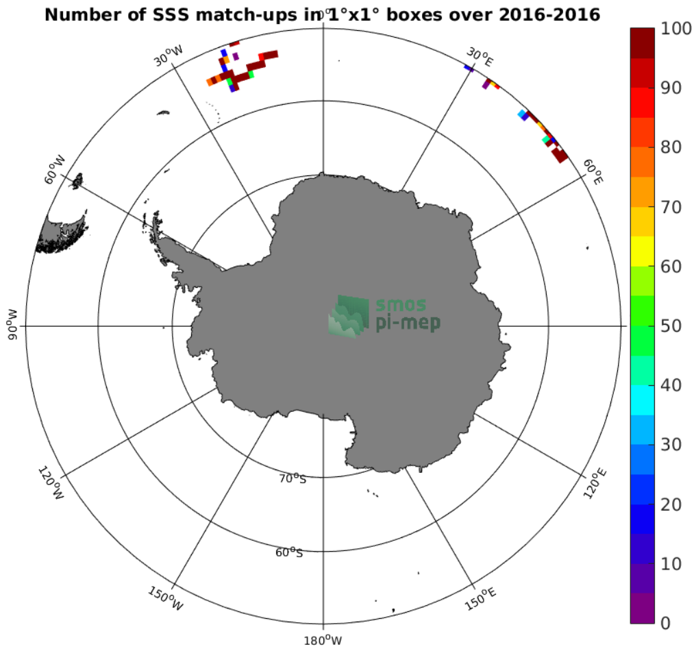
Figure 3: Number of SSS match-ups between Surface drifters SSS and the SMOS-L3-BEC-OA-V1-9DAYS-0.25DEG SSS product for the Southern Ocean Pi-MEP region over 1^\circ \times 1^\circ boxes and for the full satellite product period.
