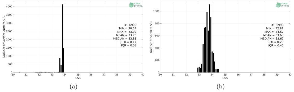
Figure 2: Histograms of SSS from Surface drifters (a) and SMOS-L3-BEC-OA-V1-9DAYS-0.25DEG (b) considering all match-up pairs per bins of 0.1 over the Southern Ocean Pi-MEP region and for the full satellite product period.
