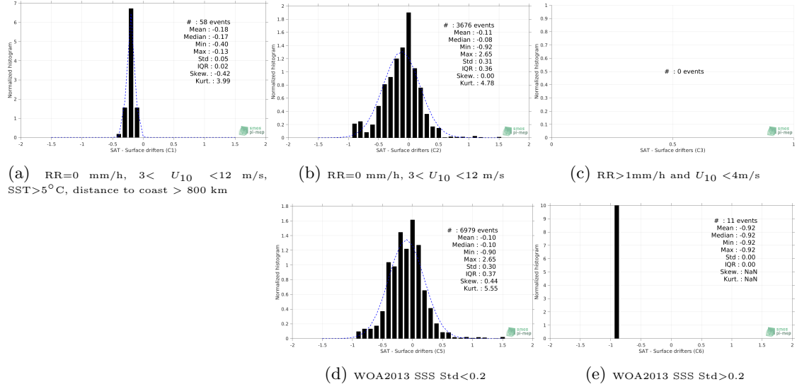
Figure 12: Normalized histogram of \Delta SSS (SMOS-L3-BEC-OA-V1-9DAYS-0.25DEG - Surface drifters) for 5 different subdatasets corresponding to: RR=0 mm/h, 3 < U_{10} < 12 m/s, SST > 5^\circ C , distance to coast > 800 km (a), RR=0 mm/h, 3 < U_{10} < 12 m/s (b), RR > 1 mm/h and U_{10} < 4 m/s (c), WOA2013 SSS Std < 0.2 (d), WOA2013 SSS Std > 0.2 (e).
