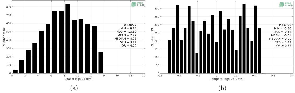
Figure 4: Histograms of the spatial (a) and temporal (b) lags between the time of the Surface drifters measurements and the date of the corresponding SMOS-L3-BEC-OA-V1-9DAYS-0.25DEG SSS product.
