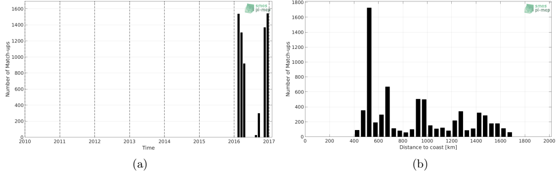
Figure 1: Number of match-ups between Surface drifters and SMOS-L3-BEC-OA-V1-9DAYS-0.25DEG SSS as a function of time (a) and as function of the distance to coast (b) over the Southern Ocean Pi-MEP region and for the full satellite product period.
