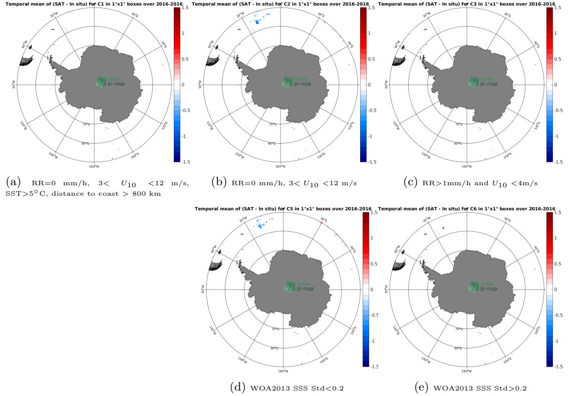
Figure 11: Temporal mean gridded over spatial boxes of size 1^\circ \times 1^\circ of \Delta SSS (SMOS-L3-BEC-OA-V1-9DAYS-0.25DEG - Surface drifters) for 5 different subdatasets corresponding to: RR=0 mm/h, 3 < U_{10} < 12 m/s, SST > 5^\circ C , distance to coast > 800 km (a), RR=0 mm/h, 3 < U_{10} < 12 m/s (b), RR > 1 mm/h and U_{10} < 4 m/s (c), WOA2013 SSS Std < 0.2 (d), WOA2013 SSS Std > 0.2 (e).
