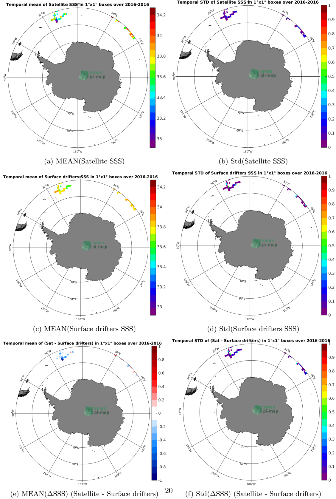
Figure 5: Temporal mean (left) and Std (right) of SSS from SMOS-L3-BEC-OA-V1-9DAYS-0.25DEG (top), Surface drifters (middle), and of \Delta SSS (Satellite - Surface drifters). Only match-up pairs are used to generate these maps.
