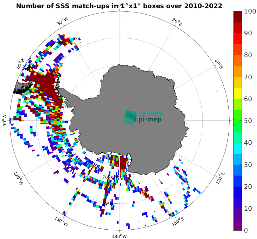
Figure 5: Number of SSS match-ups between TSG (SAMOS) SSS and the SMOS SSS L2 v700 (ESA) SSS product for the Southern Ocean Pi-MEP region over 1^{\circ} \times 1^{\circ} boxes and for the full satellite product period.
