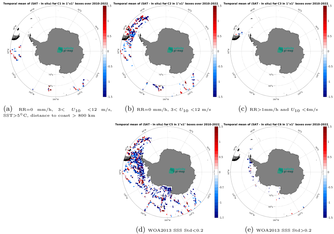
Figure 12: Temporal mean gridded over spatial boxes of size 1^{\circ}\times 1^{\circ} of \Delta\text{SSS} (SMOS SSS L2 v700 (ESA) - TSG (SAMOS)) for 5 different subdatasets corresponding to: \text{RR}=0 mm/h, 3 < U_{10} < 12 m/s, \text{SST} > 5^{\circ}\text{C} , distance to coast > 800 km (a), \text{RR}=0 mm/h, 3 < U_{10} < 12 m/s (b), \text{RR} > 1 mm/h and U_{10} < 4 m/s (c), WOA2013 SSS Std < 0.2 (d), WOA2013 SSS Std > 0.2 (e).
