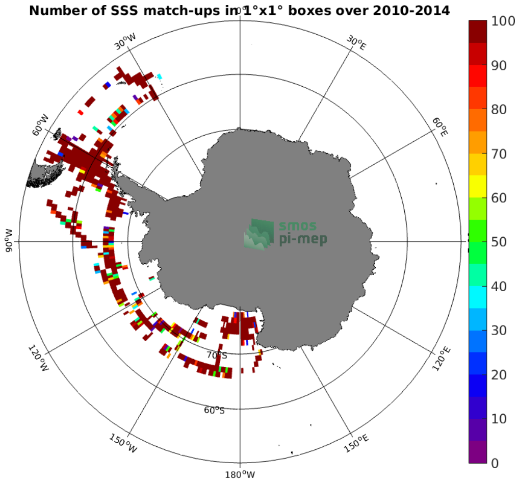
Figure 4: Number of SSS match-ups between TSG (SAMOS) SSS and the SMOS SSS L2 v700 (ESA) SSS product for the Southern Ocean Pi-MEP region over 1^{\circ} \times 1^{\circ} boxes and for the full satellite product period.
