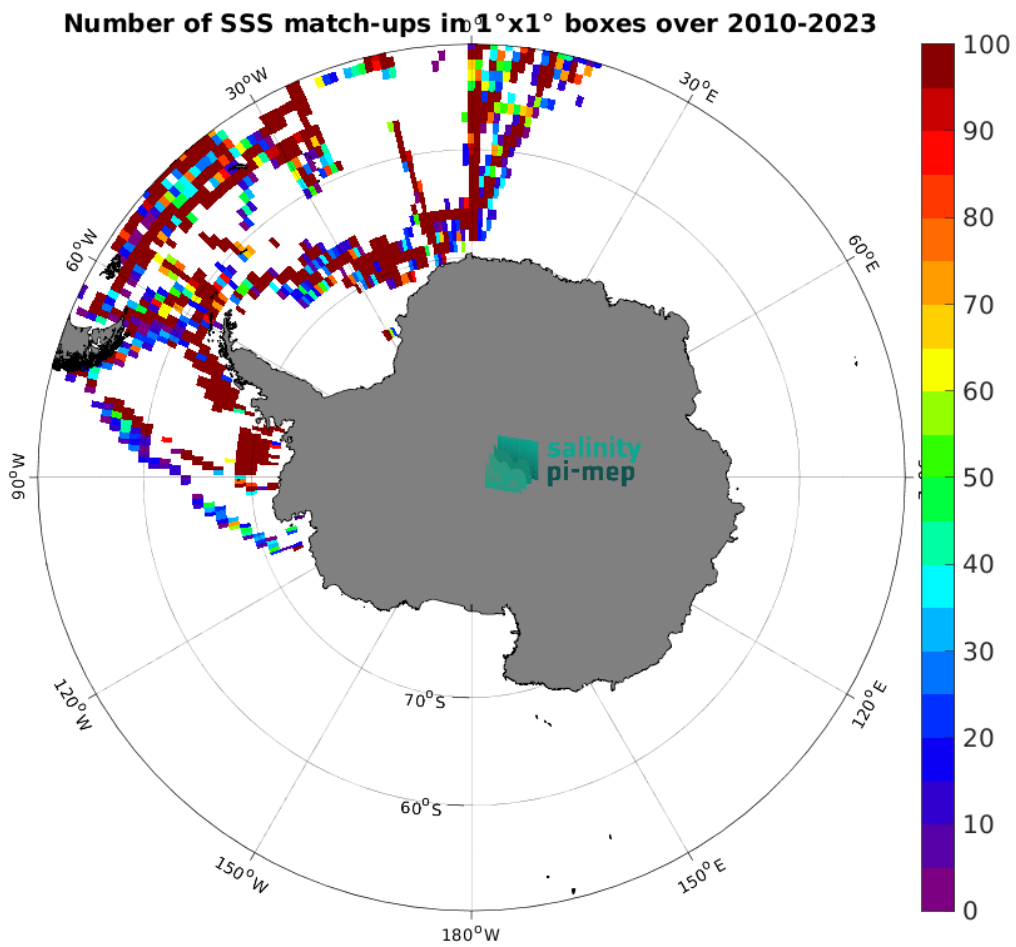
Figure 5: Number of SSS match-ups between TSG (Polarstern) SSS and the SMOS SSS L2 v700 (ESA) SSS product for the Southern Ocean Pi-MEP region over 1^\circ \times 1^\circ boxes and for the full satellite product period.
