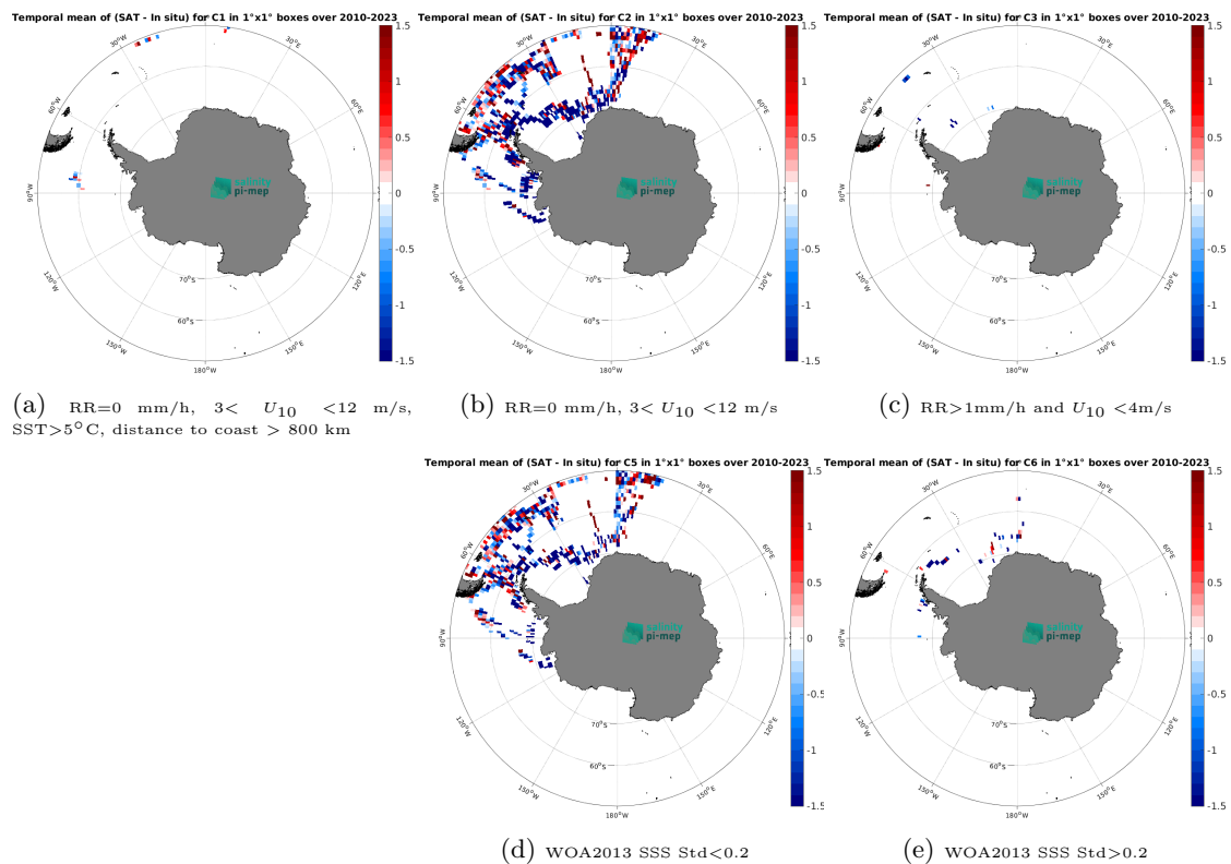
Figure 14: Temporal mean gridded over spatial boxes of size 1^\circ \times 1^\circ of \Delta SSS (SMOS SSS L2 v700 (ESA) - TSG (Polarstern)) for 5 different subdatasets corresponding to:RR=0 mm/h, 3 < U_{10} < 12 m/s, SST>5°C, distance to coast > 800 km (a), RR=0 mm/h, 3 < U_{10} < 12 m/s (b), RR>1mm/h and U_{10} < 4 m/s (c), WOA2013 SSS Std<0.2 (d), WOA2013 SSS Std>0.2 (e).
