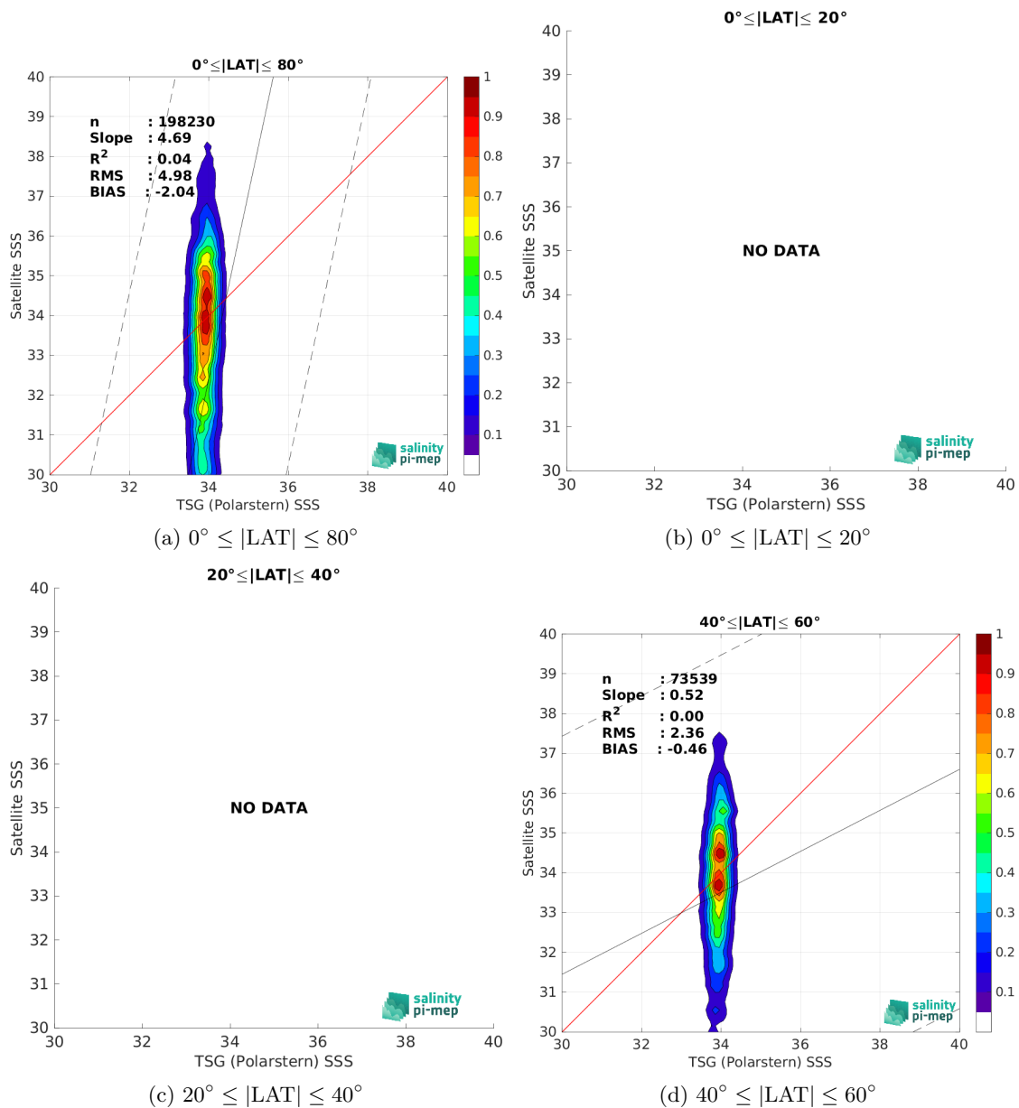
Figure 10: Contour maps of the concentration of SMOS SSS L2 v700 (ESA) SSS (y-axis) versus TSG (Polarstern) SSS (x-axis) at match-up pairs for different latitude bands. For each plot, the red line shows x=y . The black thin and dashed lines indicate a linear fit through the data cloud and the \pm 95\% confidence levels, respectively. The number match-up pairs n , the slope and R^2 coefficient of the linear fit, the root mean square (RMS) and the mean bias between satellite and in situ data are indicated for each latitude band in each plots.
