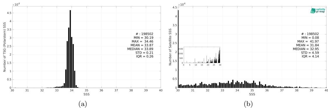
Figure 3: Histograms of SSS from TSG (Polarstern) (a) and SMOS SSS L2 v700 (ESA) (b) considering all match-up pairs per bins of 0.1 over the Southern Ocean Pi-MEP region and for the full satellite product period.
