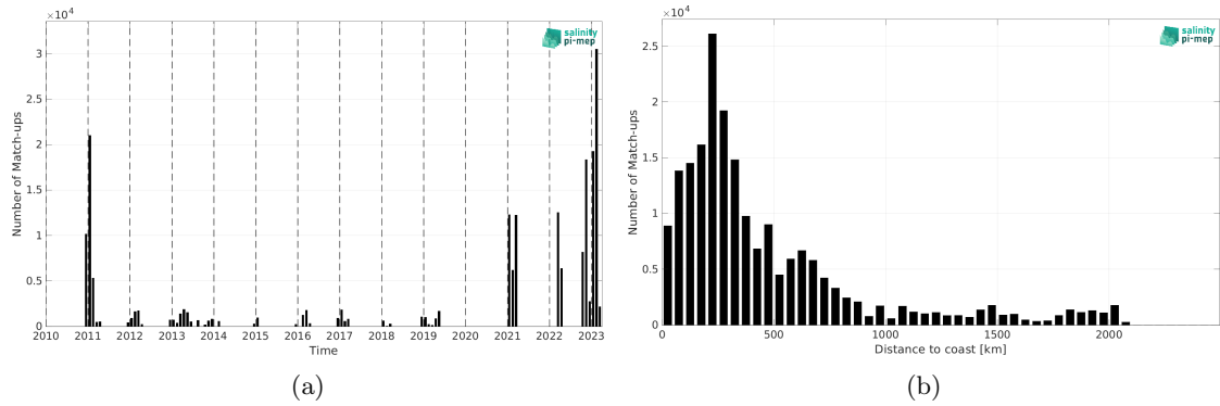
Figure 2: Number of match-ups between TSG (Polarstern) and SMOS SSS L2 v700 (ESA) SSS as a function of time (a) and as function of the distance to coast (b) over the Southern Ocean Pi-MEP region and for the full satellite product period.
