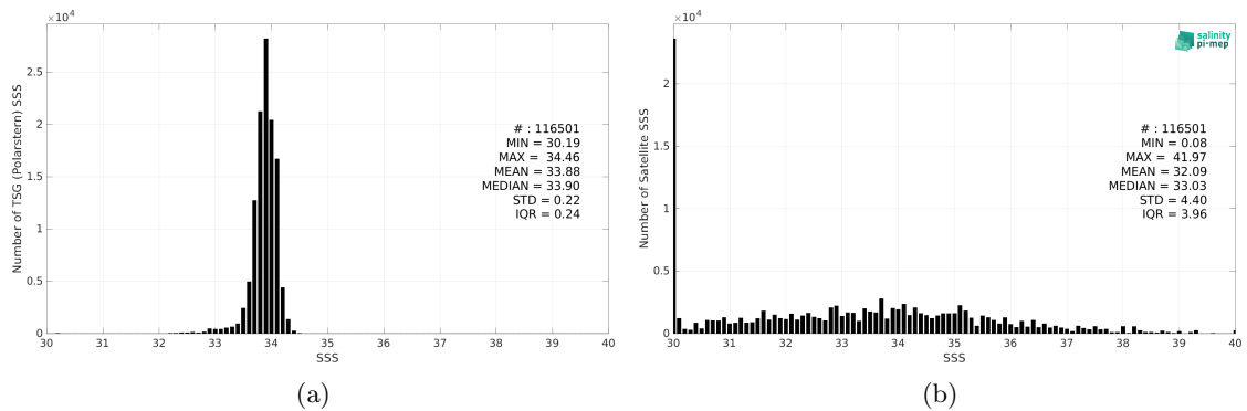
Figure 2: Histograms of SSS from TSG (Polarstern) (a) and SMOS SSS L2 v700 (ESA) (b) considering all match-up pairs per bins of 0.1 over the Southern Ocean Pi-MEP region and for the full satellite product period.
