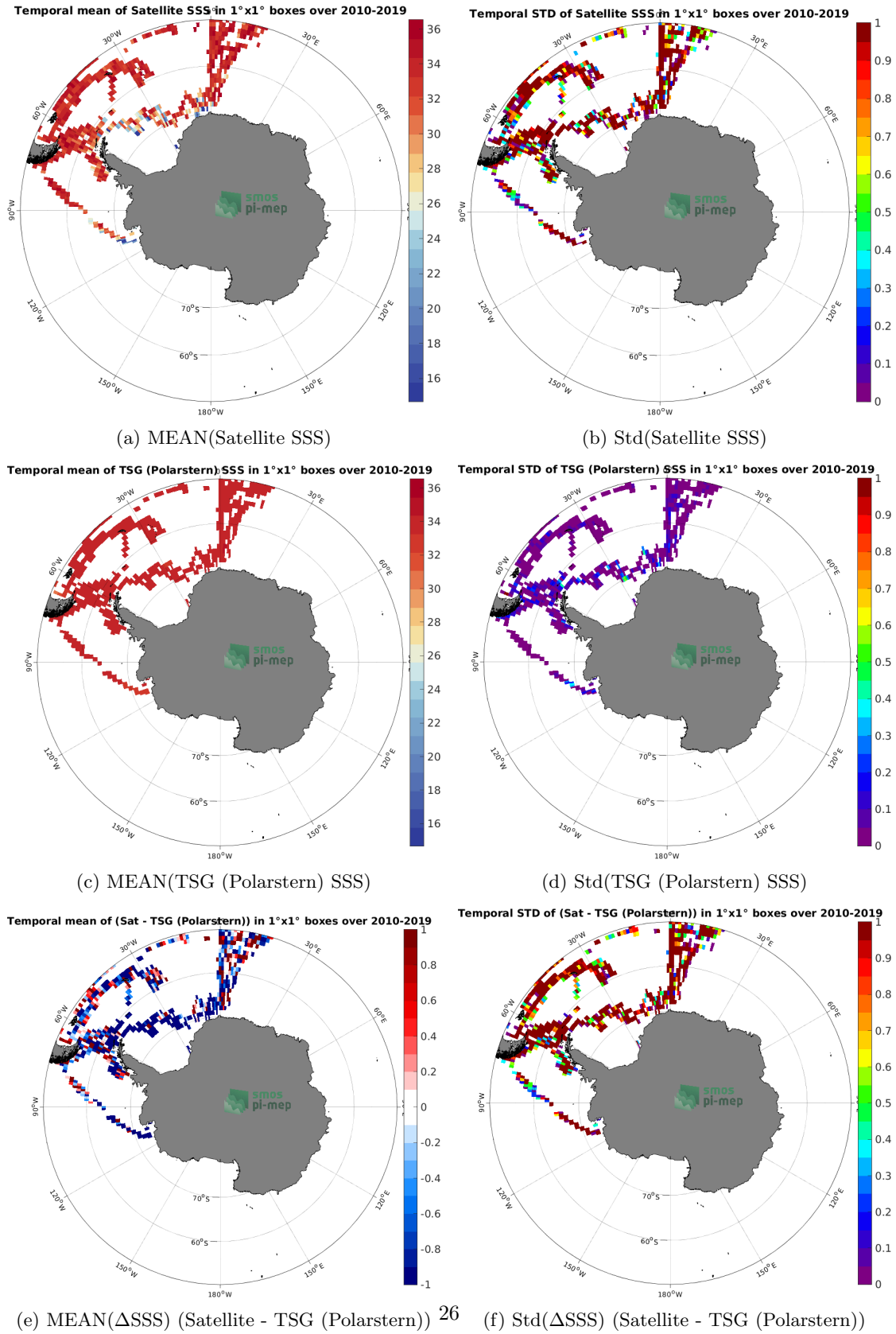
Figure 6: Temporal mean (left) and Std (right) of SSS from SMOS SSS L2 v700 (ESA) (top), TSG (Polarstern) (middle), and of \Delta SSS (Satellite - TSG (Polarstern)). Only match-up pairs are used to generate these maps.
