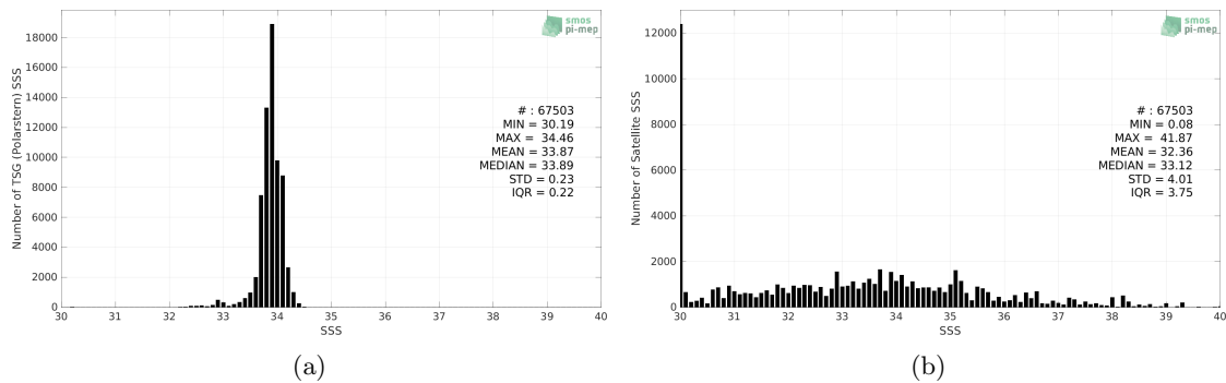
Figure 2: Histograms of SSS from TSG (Polarstern) (a) and SMOS SSS L2 v700 (ESA) (b) considering all match-up pairs per bins of 0.1 over the Southern Ocean Pi-MEP region and for the full satellite product period.
