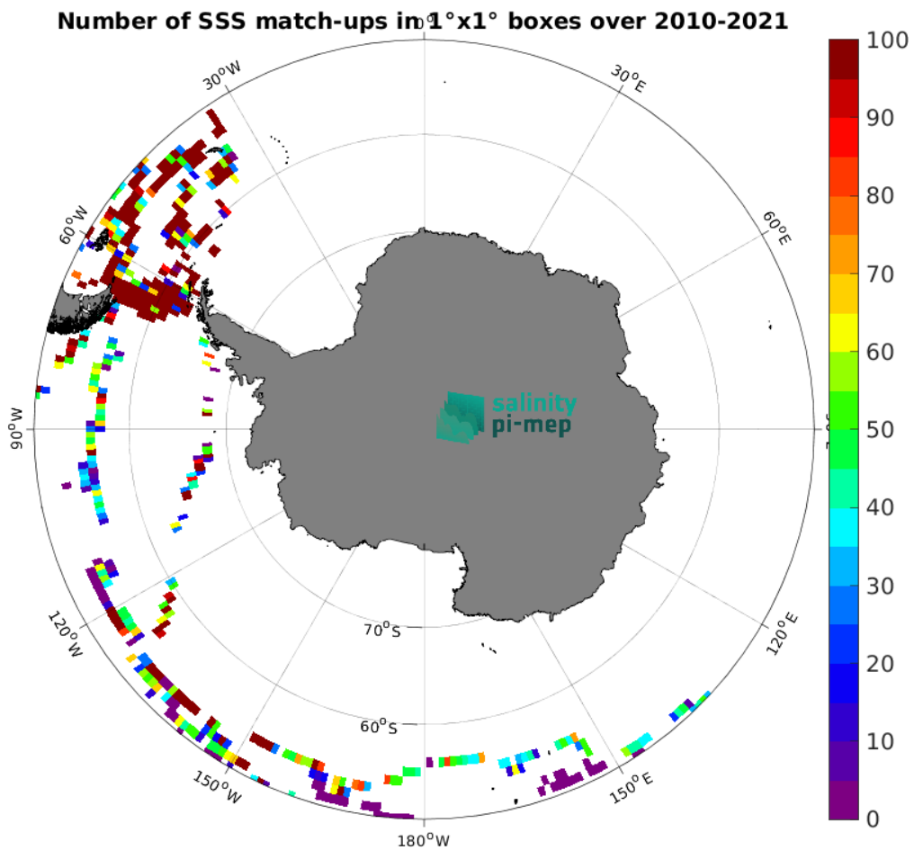
Figure 5: Number of SSS match-ups between TSG (GOSUD-Sailing-ship) SSS and the SMOS SSS L2 v700 (ESA) SSS product for the Southern Ocean Pi-MEP region over 1^\circ \times 1^\circ boxes and for the full satellite product period.
