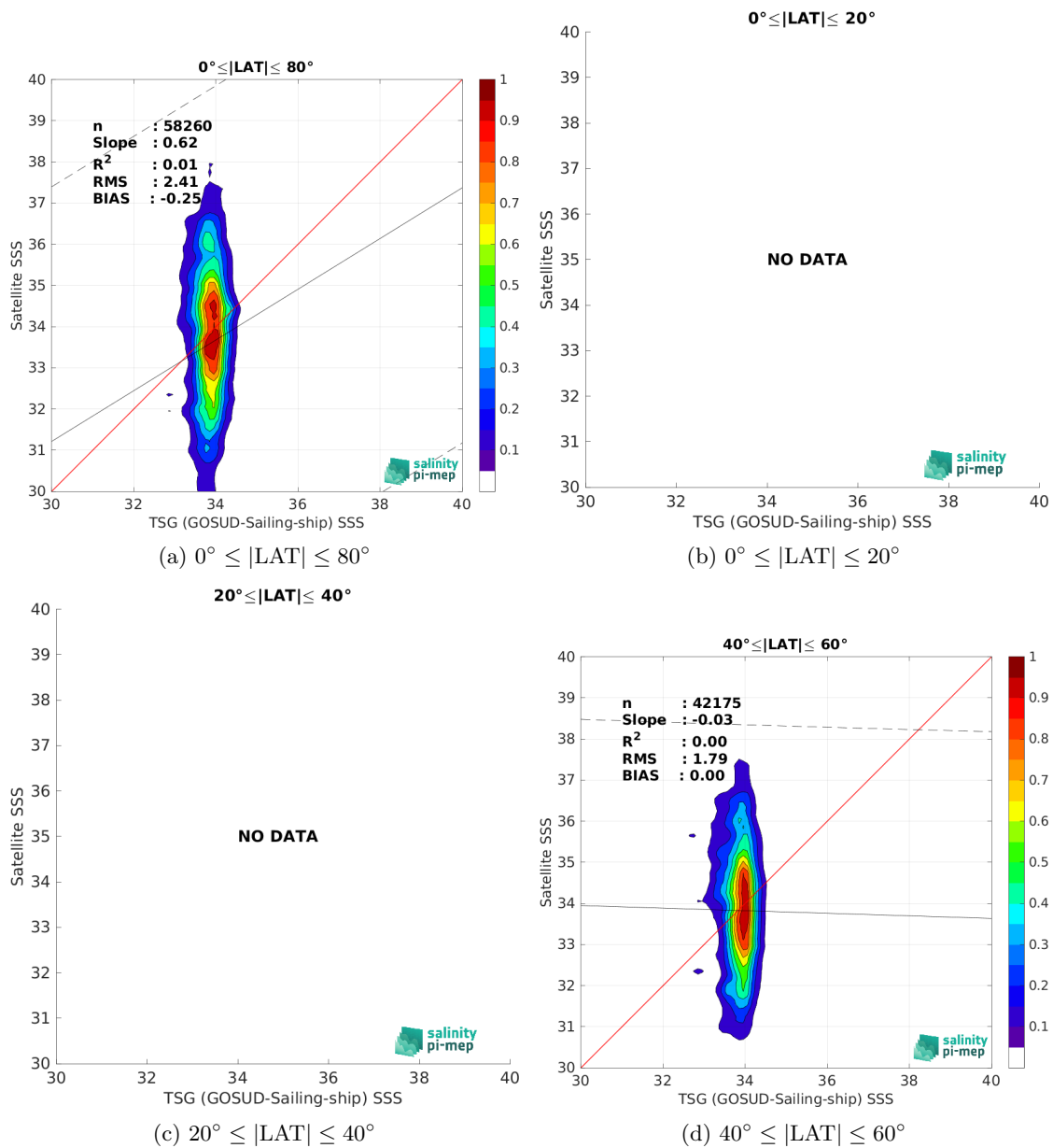
Figure 10: Contour maps of the concentration of SMOS SSS L2 v700 (ESA) SSS (y-axis) versus TSG (GOSUD-Sailing-ship) SSS (x-axis) at match-up pairs for different latitude bands. For each plot, the red line shows x=y . The black thin and dashed lines indicate a linear fit through the data cloud and the \pm 95\% confidence levels, respectively. The number match-up pairs n , the slope and R^2 coefficient of the linear fit, the root mean square (RMS) and the mean bias between satellite and in situ data are indicated for each latitude band in each plots.
