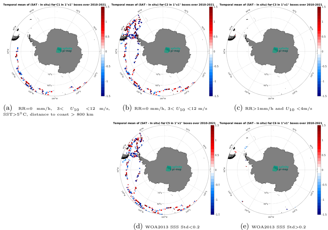
Figure 14: Temporal mean gridded over spatial boxes of size 1^\circ \times 1^\circ of \Delta\text{SSS} (SMOS SSS L2 v700 (ESA) - TSG (GOSUD-Sailing-ship)) for 5 different subdatasets corresponding to: RR=0 mm/h, 3 < U_{10} < 12 m/s, SST > 5°C, distance to coast > 800 km (a), RR=0 mm/h, 3 < U_{10} < 12 m/s (b), RR > 1mm/h and U_{10} < 4 m/s (c), WOA2013 SSS Std < 0.2 (d), WOA2013 SSS Std > 0.2 (e).
