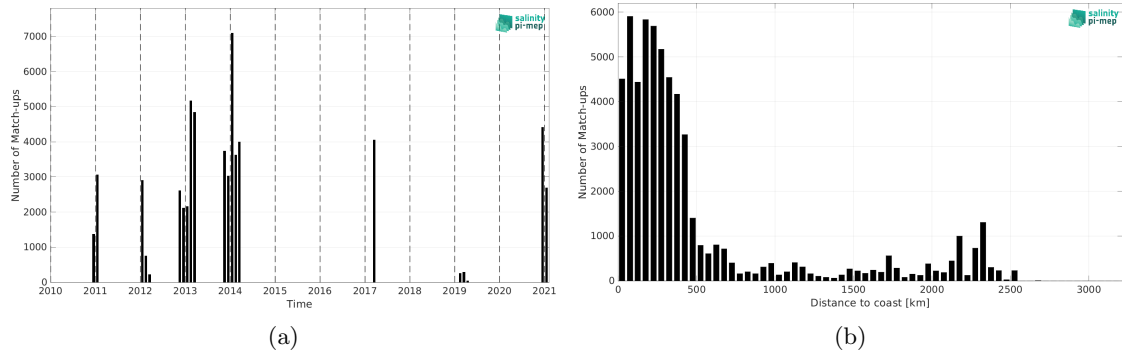
Figure 2: Number of match-ups between TSG (GOSUD-Sailing-ship) and SMOS SSS L2 v700 (ESA) SSS as a function of time (a) and as function of the distance to coast (b) over the Southern Ocean Pi-MEP region and for the full satellite product period.
