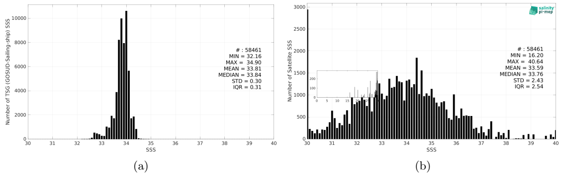
Figure 3: Histograms of SSS from TSG (GOSUD-Sailing-ship) (a) and SMOS SSS L2 v700 (ESA) (b) considering all match-up pairs per bins of 0.1 over the Southern Ocean Pi-MEP region and for the full satellite product period.
