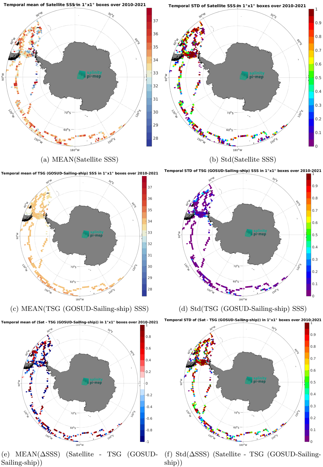
Figure 7: Temporal mean (left) and Std (right) of SSS from SMOS SSS L2 v700 (ESA) (top), TSG (GOSUD-Sailing-ship) (middle), and of \Delta SSS (Satellite - TSG (GOSUD-Sailing-ship)). Only match-up pairs are used to generate these maps.
