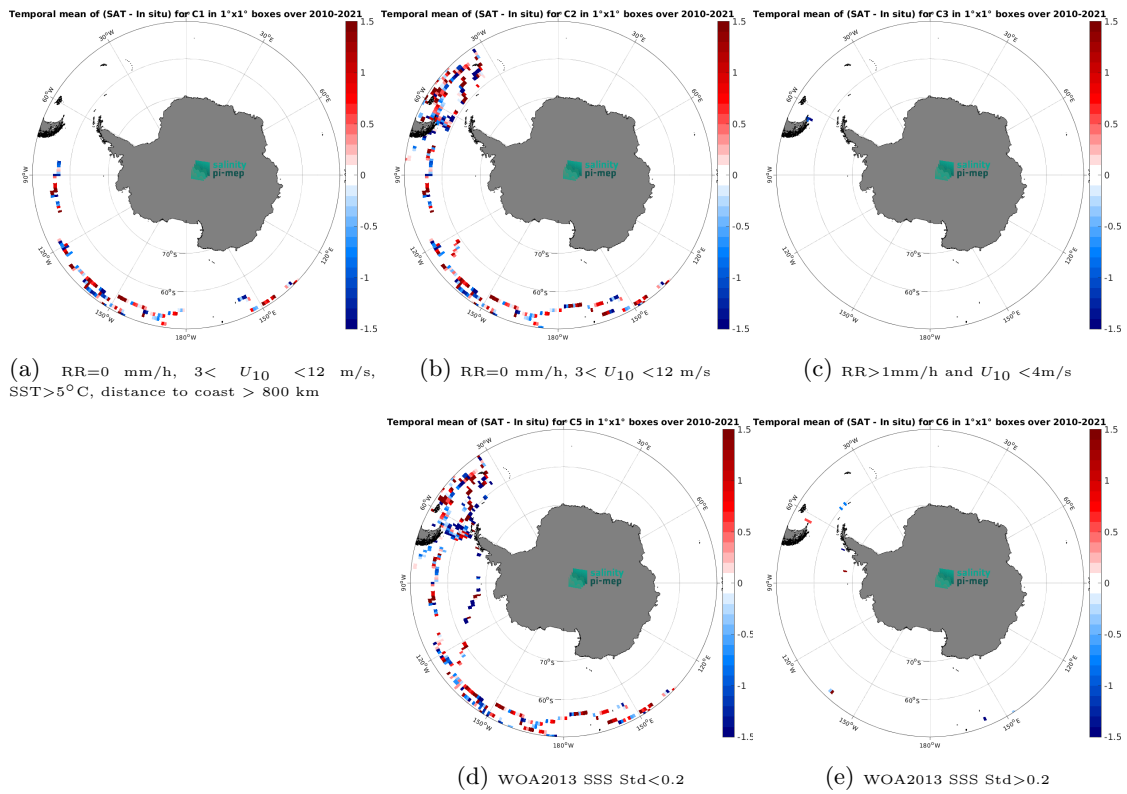
Figure 12: Temporal mean gridded over spatial boxes of size 1^\circ \times 1^\circ of \Delta SSS (SMOS SSS L2 v700 (ESA) - TSG (GOSUD-Sailing-ship)) for 5 different subdatasets corresponding to: RR=0 mm/h, 3 < U_{10} < 12 m/s, SST > 5°C, distance to coast > 800 km (a), RR=0 mm/h, 3 < U_{10} < 12 m/s (b), RR > 1mm/h and U_{10} < 4 m/s (c), WOA2013 SSS Std < 0.2 (d), WOA2013 SSS Std > 0.2 (e).
