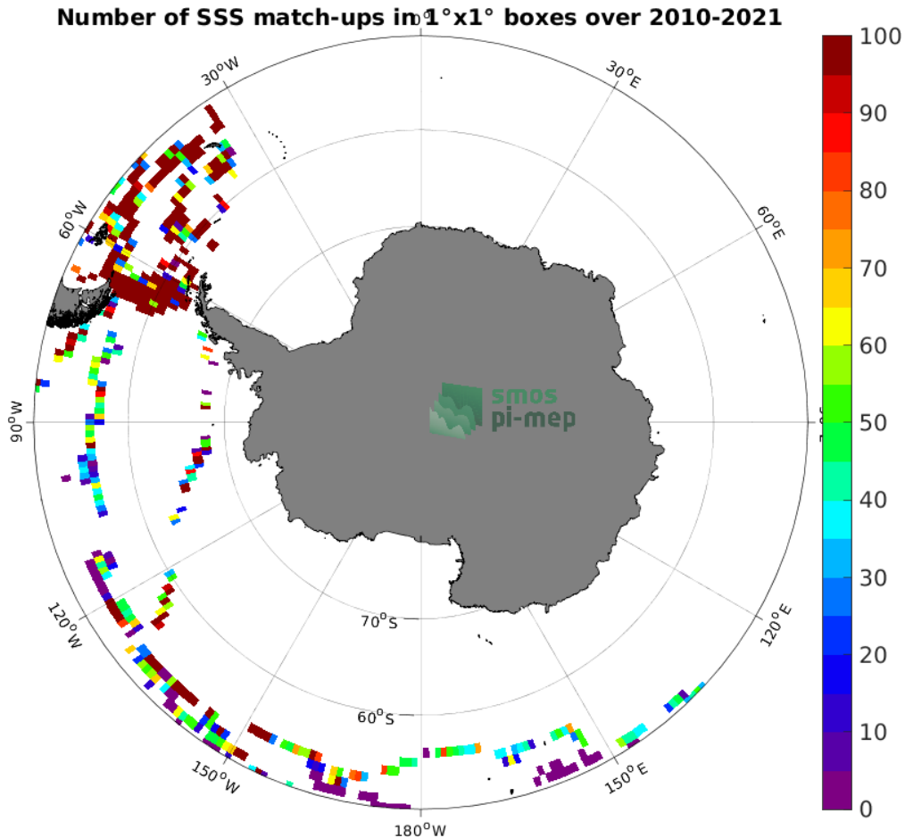
Figure 4: Number of SSS match-ups between TSG (GOSUD-Sailing-ship) SSS and the SMOS SSS L2 v700 (ESA) SSS product for the Southern Ocean Pi-MEP region over 1^\circ \times 1^\circ boxes and for the full satellite product period.
