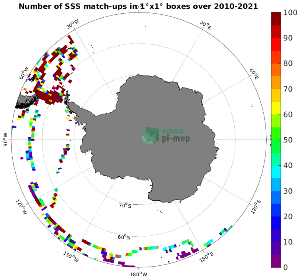
Figure 4: Number of SSS match-ups between TSG (GOSUD-Sailing-ship) SSS and the SMOS SSS L2 v700 (ESA) SSS product for the Southern Ocean Pi-MEP region over 1^\circ \times 1^\circ boxes and for the full satellite product period.
