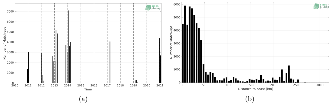
Figure 1: Number of match-ups between TSG (GOSUD-Sailing-ship) and SMOS SSS L2 v700 (ESA) SSS as a function of time (a) and as function of the distance to coast (b) over the Southern Ocean Pi-MEP region and for the full satellite product period.
