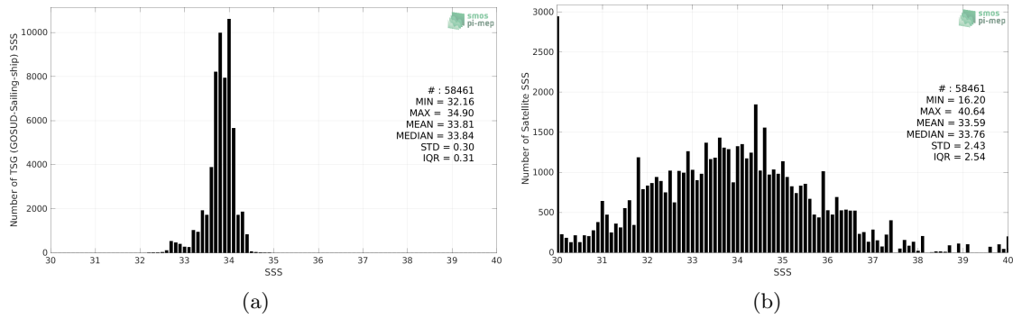
Figure 2: Histograms of SSS from TSG (GOSUD-Sailing-ship) (a) and SMOS SSS L2 v700 (ESA) (b) considering all match-up pairs per bins of 0.1 over the Southern Ocean Pi-MEP region and for the full satellite product period.
