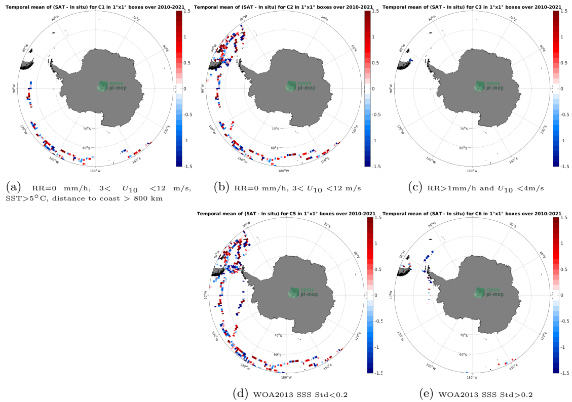
Figure 12: Temporal mean gridded over spatial boxes of size 1^\circ \times 1^\circ of \Delta SSS (SMOS SSS L2 v700 (ESA) - TSG (GOSUD-Sailing-ship)) for 5 different subdatasets corresponding to:RR=0 mm/h, 3 < U_{10} < 12 m/s, SST>5°C, distance to coast > 800 km (a), RR=0 mm/h, 3 < U_{10} < 12 m/s (b), RR>1mm/h and U_{10} < 4 m/s (c), WOA2013 SSS Std<0.2 (d), WOA2013 SSS Std>0.2 (e).
