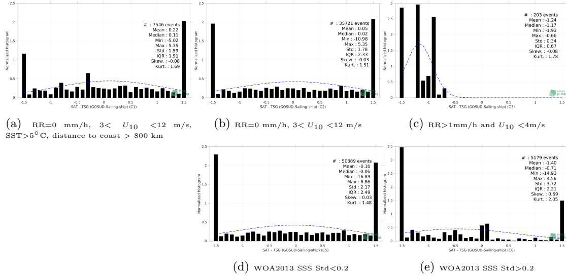
Figure 13: Normalized histogram of \Delta SSS (SMOS SSS L2 v700 (ESA) - TSG (GOSUD-Sailing-ship)) for 5 different subdatasets corresponding to: RR=0 mm/h, 3 < U_{10} < 12 m/s, SST > 5°C, distance to coast > 800 km (a), RR=0 mm/h, 3 < U_{10} < 12 m/s (b), RR > 1mm/h and U_{10} < 4 m/s (c), WOA2013 SSS Std < 0.2 (d), WOA2013 SSS Std > 0.2 (e).
