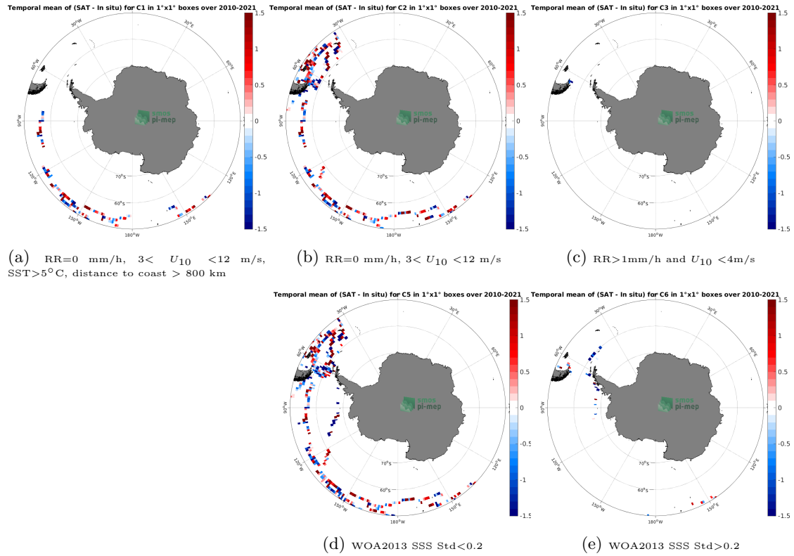
Figure 12: Temporal mean gridded over spatial boxes of size 1^{\circ} \times 1^{\circ} of \Delta SSS (SMOS SSS L2 v700 (ESA) - TSG (GOSUD-Sailing-ship)) for 5 different subdatasets corresponding to: RR=0 mm/h, 3 < U_{10} < 12 m/s, SST > 5^{\circ}C , distance to coast > 800 km (a), RR=0 mm/h, 3 < U_{10} < 12 m/s (b), RR > 1 mm/h and U_{10} < 4 m/s (c), WOA2013 SSS Std < 0.2 (d), WOA2013 SSS Std > 0.2 (e).
