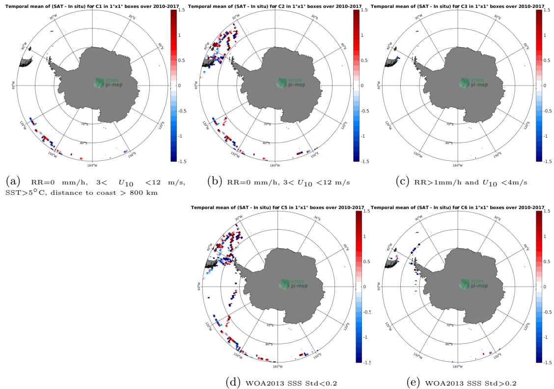
Figure 12: Temporal mean gridded over spatial boxes of size 1^{\circ}\times 1^{\circ} of \Delta SSS (SMOS SSS L2 v700 (ESA) - TSG (GOSUD-Sailing-ship)) for 5 different subdatasets corresponding to:RR=0 mm/h, 3 < U_{10} < 12 m/s, SST >5^{\circ}\text{C} , distance to coast > 800 km (a), RR=0 mm/h, 3 < U_{10} < 12 m/s (b), RR >1 mm/h and U_{10} < 4 m/s (c), WOA2013 SSS Std <0.2 (d), WOA2013 SSS Std >0.2 (e).
