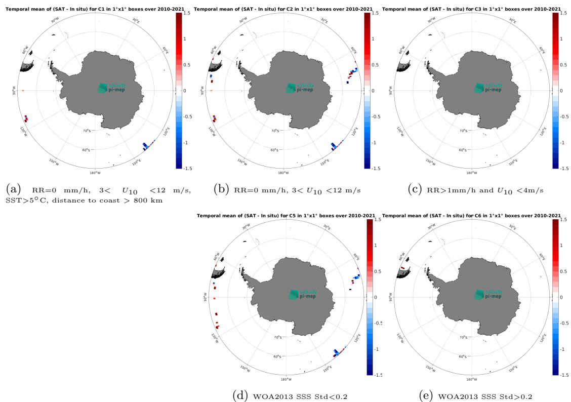
Figure 14: Temporal mean gridded over spatial boxes of size 1^\circ \times 1^\circ of \Delta\text{SSS} (SMOS SSS L2 v700 (ESA) - TSG (GOSUD-Research-vessel)) for 5 different subdatasets corresponding to:RR=0 mm/h, 3 < U_{10} < 12 m/s, SST>5°C, distance to coast > 800 km (a), RR=0 mm/h, 3 < U_{10} < 12 m/s (b), RR>1mm/h and U_{10} < 4 m/s (c), WOA2013 SSS Std<0.2 (d), WOA2013 SSS Std>0.2 (e).
