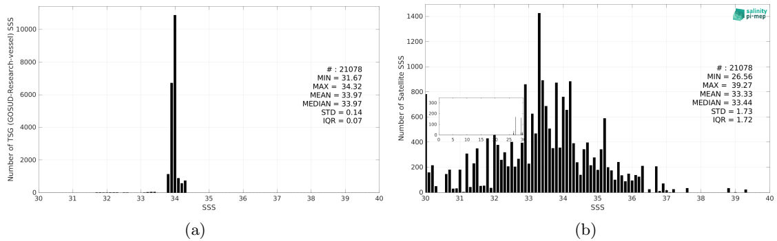
Figure 3: Histograms of SSS from TSG (GOSUD-Research-vessel) (a) and SMOS SSS L2 v700 (ESA) (b) considering all match-up pairs per bins of 0.1 over the Southern Ocean Pi-MEP region and for the full satellite product period.
