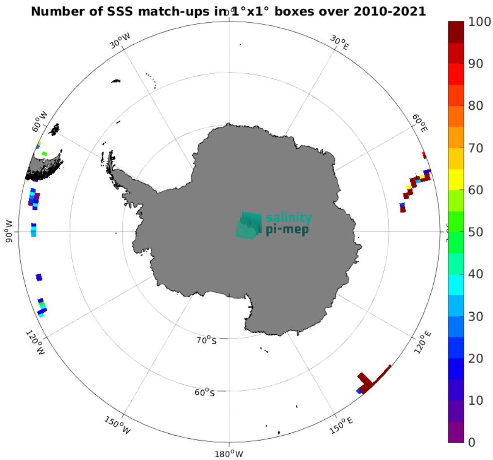
Figure 5: Number of SSS match-ups between TSG (GOSUD-Research-vessel) SSS and the SMOS SSS L2 v700 (ESA) SSS product for the Southern Ocean Pi-MEP region over 1^\circ \times 1^\circ boxes and for the full satellite product period.
