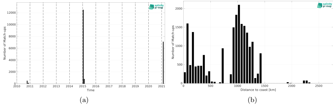
Figure 2: Number of match-ups between TSG (GOSUD-Research-vessel) and SMOS SSS L2 v700 (ESA) SSS as a function of time (a) and as function of the distance to coast (b) over the Southern Ocean Pi-MEP region and for the full satellite product period.
