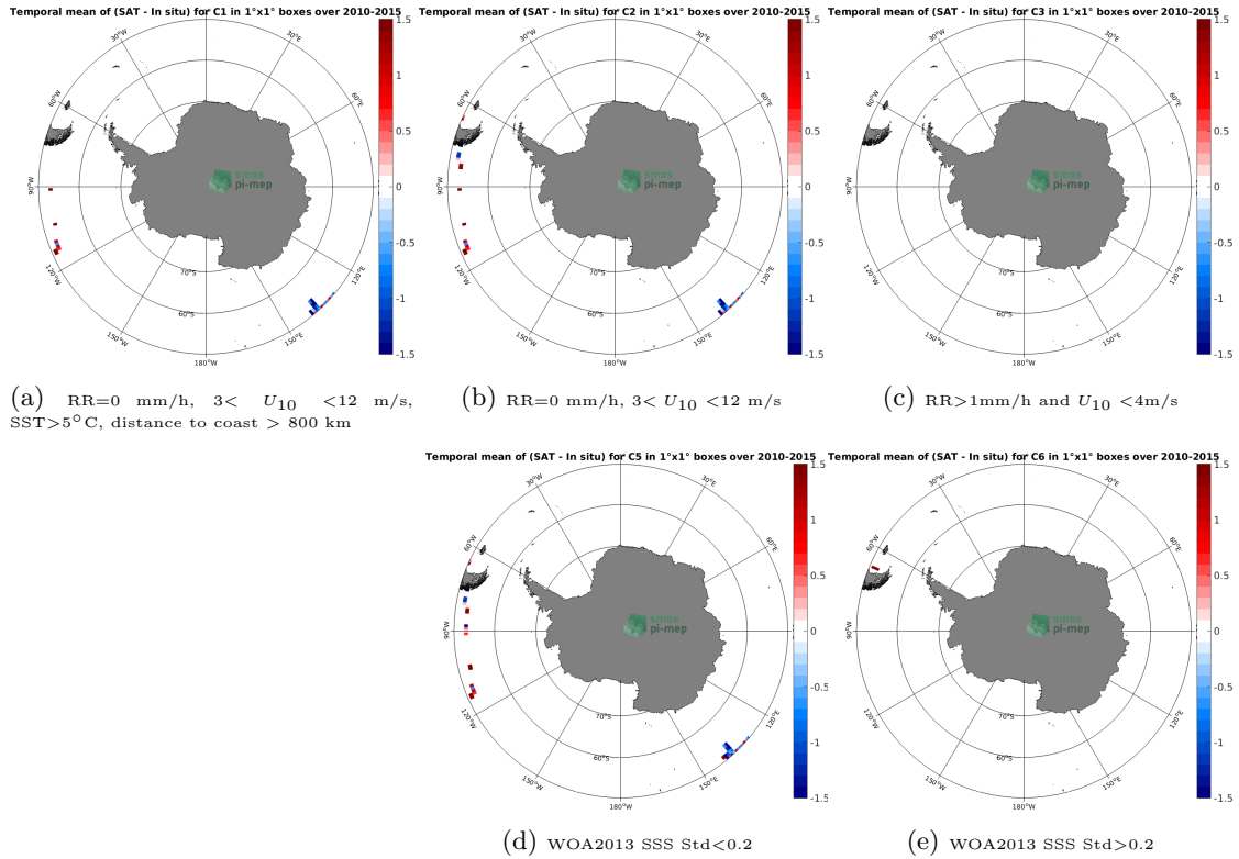
Figure 12: Temporal mean gridded over spatial boxes of size 1^\circ \times 1^\circ of \Delta SSS (SMOS SSS L2 v700 (ESA) - TSG (GOSUD-Research-vessel)) for 5 different subdatasets corresponding to:RR=0 mm/h, 3 < U_{10} < 12 m/s, SST>5°C, distance to coast > 800 km (a), RR=0 mm/h, 3 < U_{10} < 12 m/s (b), RR>1mm/h and U_{10} < 4 m/s (c), WOA2013 SSS Std<0.2 (d), WOA2013 SSS Std>0.2 (e).
