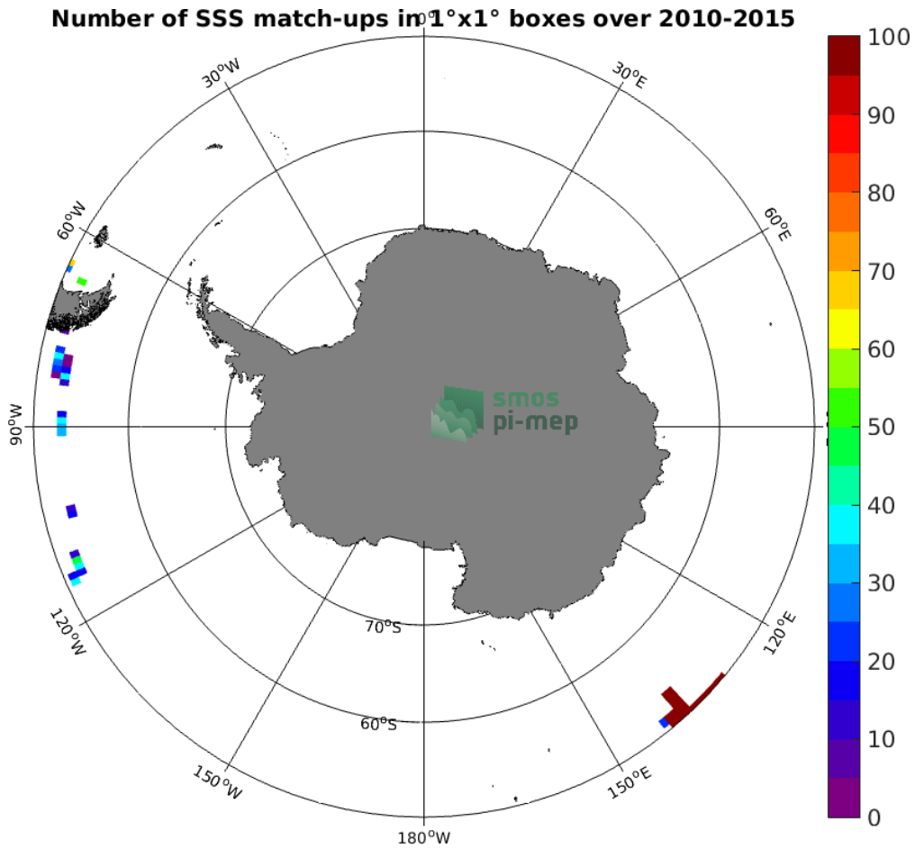
Figure 4: Number of SSS match-ups between TSG (GOSUD-Research-vessel) SSS and the SMOS SSS L2 v700 (ESA) SSS product for the Southern Ocean Pi-MEP region over 1^\circ \times 1^\circ boxes and for the full satellite product period.
