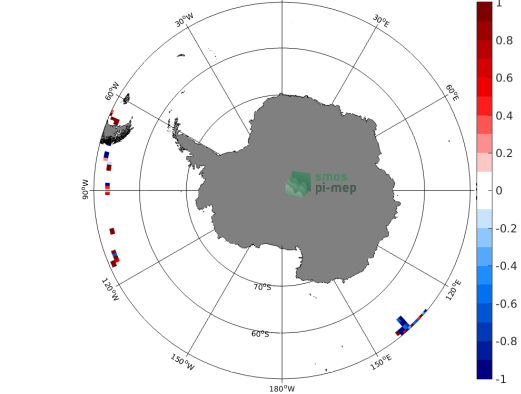
(e) MEAN( \Delta SSS) (Satellite - TSG (GOSUD-Research-vessel))
