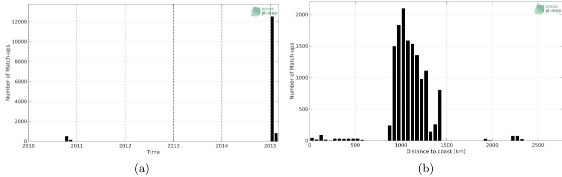
Figure 1: Number of match-ups between TSG (GOSUD-Research-vessel) and SMOS SSS L2 v700 (ESA) SSS as a function of time (a) and as function of the distance to coast (b) over the Southern Ocean Pi-MEP region and for the full satellite product period.
