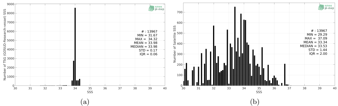
Figure 2: Histograms of SSS from TSG (GOSUD-Research-vessel) (a) and SMOS SSS L2 v700 (ESA) (b) considering all match-up pairs per bins of 0.1 over the Southern Ocean Pi-MEP region and for the full satellite product period.
