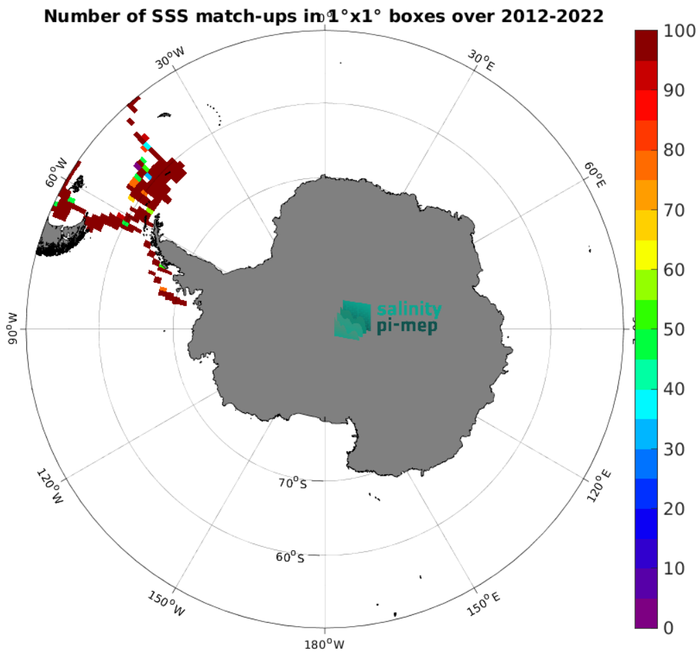
Figure 4: Number of SSS match-ups between TSG (CSIC-UTM) SSS and the SMOS SSS L2 v700 (ESA) SSS product for the Southern Ocean Pi-MEP region over 1^\circ \times 1^\circ boxes and for the full satellite product period.
