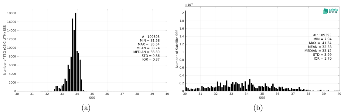
Figure 2: Histograms of SSS from TSG (CSIC-UTM) (a) and SMOS SSS L2 v700 (ESA) (b) considering all match-up pairs per bins of 0.1 over the Southern Ocean Pi-MEP region and for the full satellite product period.
