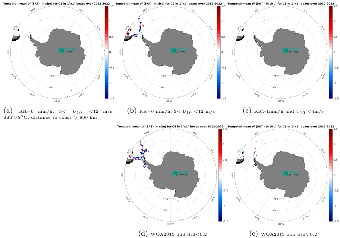
Figure 12: Temporal mean gridded over spatial boxes of size 1^{\circ}\times 1^{\circ} of \Delta\text{SSS} (SMOS SSS L2 v700 (ESA) - TSG (CSIC-UTM)) for 5 different subdatasets corresponding to:RR=0 mm/h, 3 < U_{10} < 12 m/s, SST >5^{\circ}\text{C} , distance to coast > 800 km (a), RR=0 mm/h, 3 < U_{10} < 12 m/s (b), RR >1 mm/h and U_{10} < 4 m/s (c), WOA2013 SSS Std <0.2 (d), WOA2013 SSS Std >0.2 (e).
