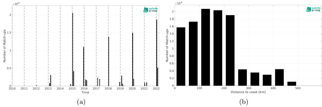
Figure 1: Number of match-ups between TSG (CSIC-UTM) and SMOS SSS L2 v700 (ESA) SSS as a function of time (a) and as function of the distance to coast (b) over the Southern Ocean Pi-MEP region and for the full satellite product period.
