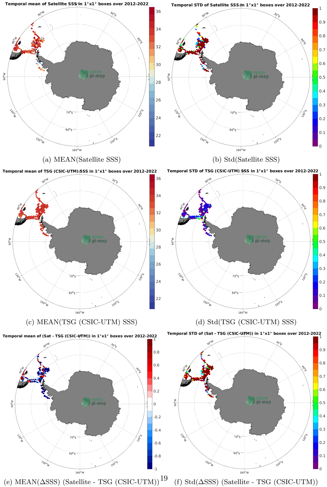
Figure 6: Temporal mean (left) and Std (right) of SSS from SMOS SSS L2 v700 (ESA) (top), TSG (CSIC-UTM) (middle), and of \Delta SSS (Satellite - TSG (CSIC-UTM)). Only match-up pairs are used to generate these maps.
