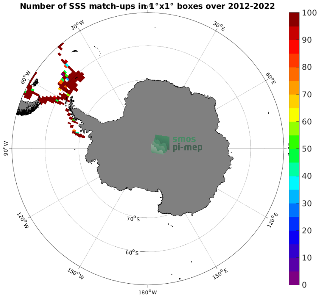
Figure 4: Number of SSS match-ups between TSG (CSIC-UTM) SSS and the SMOS SSS L2 v700 (ESA) SSS product for the Southern Ocean Pi-MEP region over 1^\circ \times 1^\circ boxes and for the full satellite product period.
