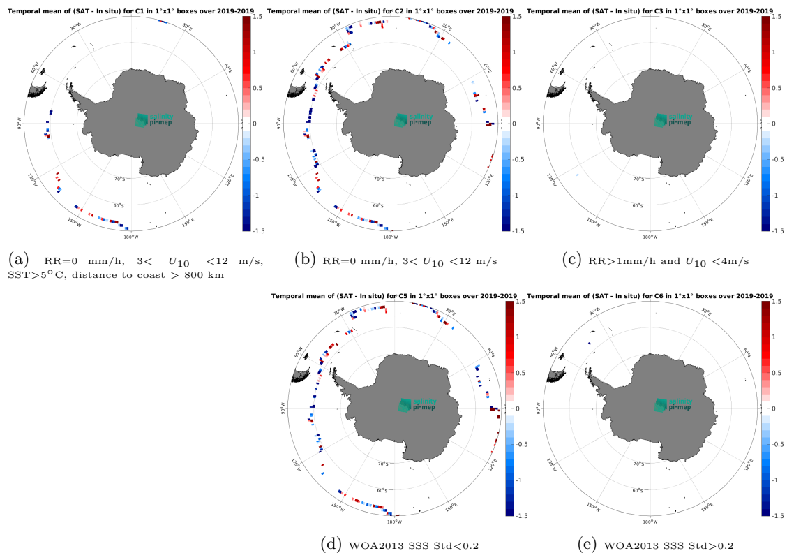
Figure 14: Temporal mean gridded over spatial boxes of size 1^\circ \times 1^\circ of \Delta SSS (SMOS SSS L2 v700 (ESA) - Sairdrone) for 5 different subdatasets corresponding to:RR=0 mm/h, 3 < U_{10} < 12 m/s, SST>5°C, distance to coast > 800 km (a), RR=0 mm/h, 3 < U_{10} < 12 m/s (b), RR>1mm/h and U_{10} < 4 m/s (c), WOA2013 SSS Std<0.2 (d), WOA2013 SSS Std>0.2 (e).
