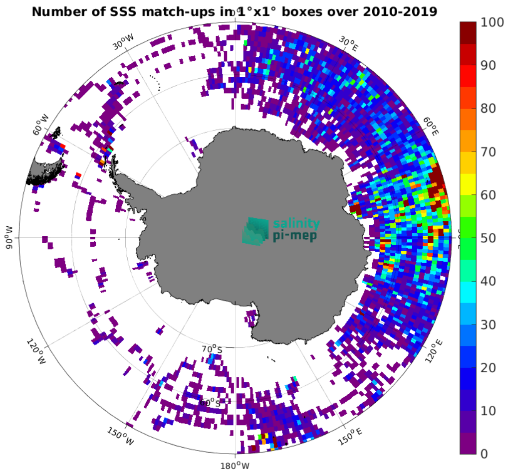
Figure 4: Number of SSS match-ups between Marine mammals SSS and the SMOS SSS L2 v700 (ESA) SSS product for the Southern Ocean Pi-MEP region over 1^{\circ} \times 1^{\circ} boxes and for the full satellite product period.
