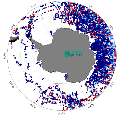
(e) MEAN( \Delta SSS) (Satellite - Marine mammals) 20
