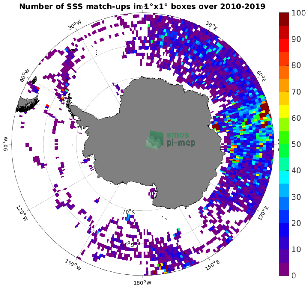
Figure 4: Number of SSS match-ups between Marine mammals SSS and the SMOS SSS L2 v700 (ESA) SSS product for the Southern Ocean Pi-MEP region over 1^\circ \times 1^\circ boxes and for the full satellite product period.
