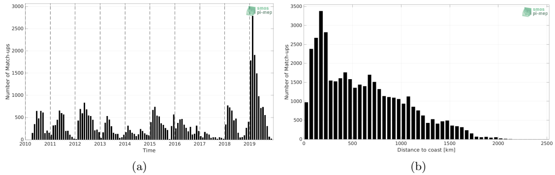
Figure 1: Number of match-ups between Marine mammals and SMOS SSS L2 v700 (ESA) SSS as a function of time (a) and as function of the distance to coast (b) over the Southern Ocean Pi-MEP region and for the full satellite product period.
