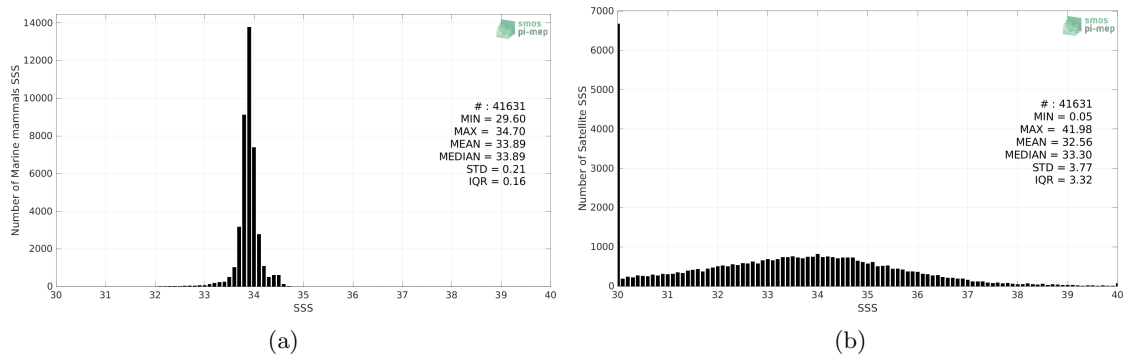
Figure 2: Histograms of SSS from Marine mammals (a) and SMOS SSS L2 v700 (ESA) (b) considering all match-up pairs per bins of 0.1 over the Southern Ocean Pi-MEP region and for the full satellite product period.
