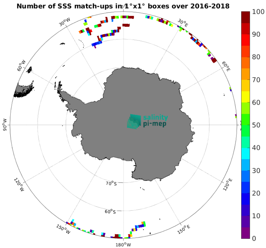
Figure 4: Number of SSS match-ups between Surface drifters SSS and the SMOS SSS L2 v700 (ESA) SSS product for the Southern Ocean Pi-MEP region over 1^{\circ} \times 1^{\circ} boxes and for the full satellite product period.
