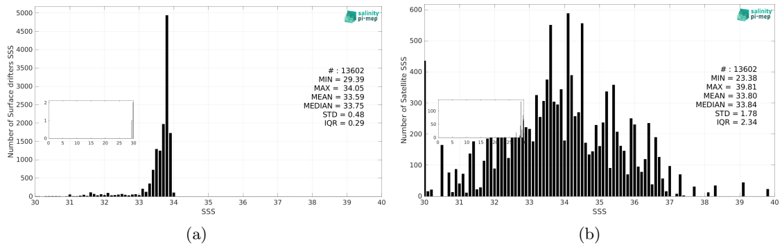
Figure 3: Histograms of SSS from Surface drifters (a) and SMOS SSS L2 v700 (ESA) (b) considering all match-up pairs per bins of 0.1 over the Southern Ocean Pi-MEP region and for the full satellite product period.
