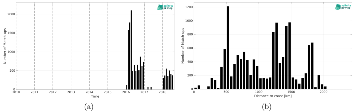
Figure 2: Number of match-ups between Surface drifters and SMOS SSS L2 v700 (ESA) SSS as a function of time (a) and as function of the distance to coast (b) over the Southern Ocean Pi-MEP region and for the full satellite product period.
