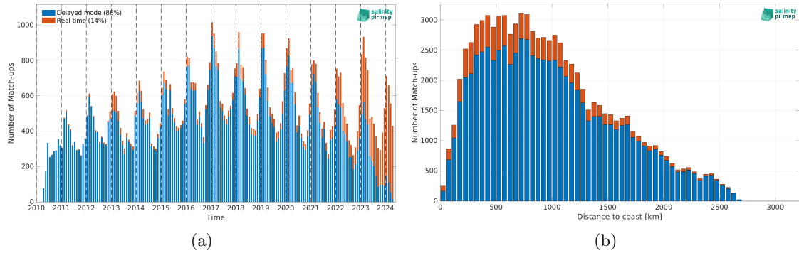
Figure 2: Number of match-ups between Argo and SMOS SSS L2 v700 (ESA) SSS as a function of time (a) and as function of the distance to coast (b) over the Southern Ocean Pi-MEP region and for the full satellite product period.
