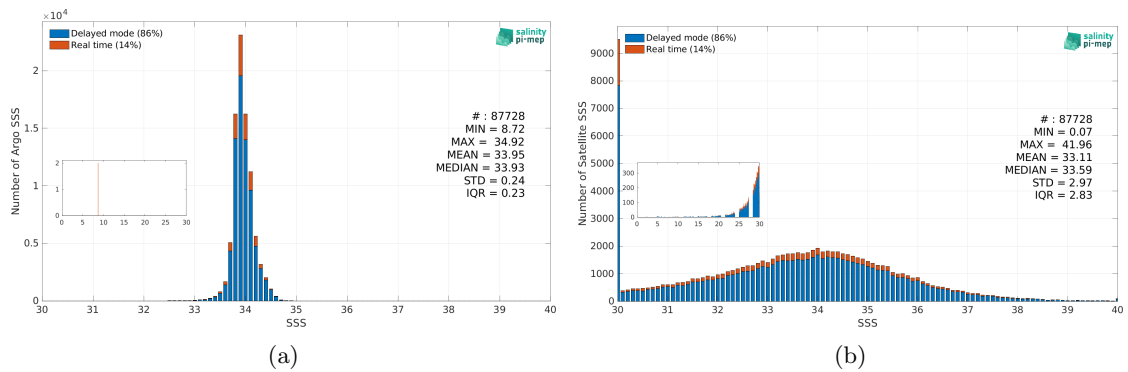
Figure 3: Histograms of SSS from Argo (a) and SMOS SSS L2 v700 (ESA) (b) considering all match-up pairs per bins of 0.1 over the Southern Ocean Pi-MEP region and for the full satellite product period.
