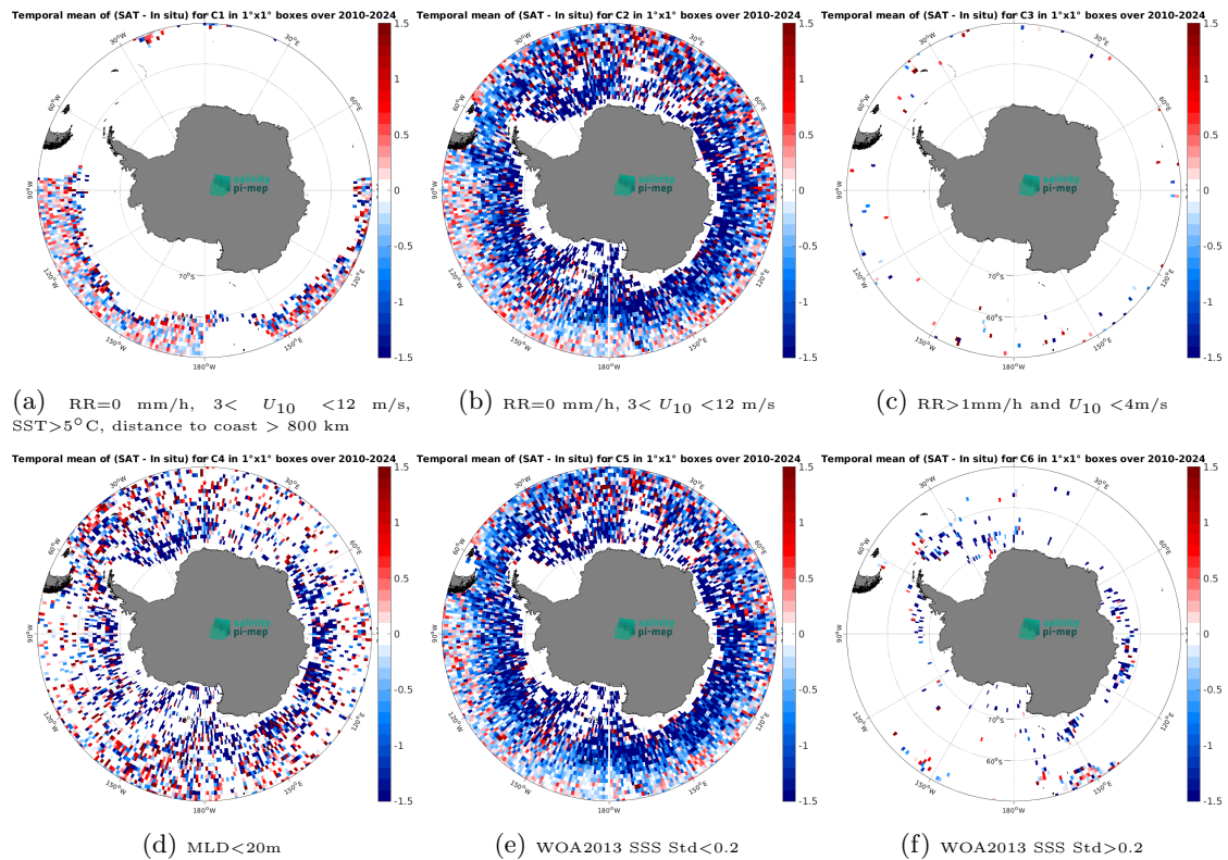
Figure 14: Temporal mean gridded over spatial boxes of size 1^\circ \times 1^\circ of \Delta SSS (SMOS SSS L2 v700 (ESA) - Argo) for 6 different subdatasets corresponding to:RR=0 mm/h, 3 < U_{10} < 12 m/s, SST>5°C, distance to coast > 800 km (a), RR=0 mm/h, 3 < U_{10} < 12 m/s (b), RR>1mm/h and U_{10} < 4 m/s (c),MLD<20m (d),WOA2013 SSS Std<0.2 (e),WOA2013 SSS Std>0.2 (f).
