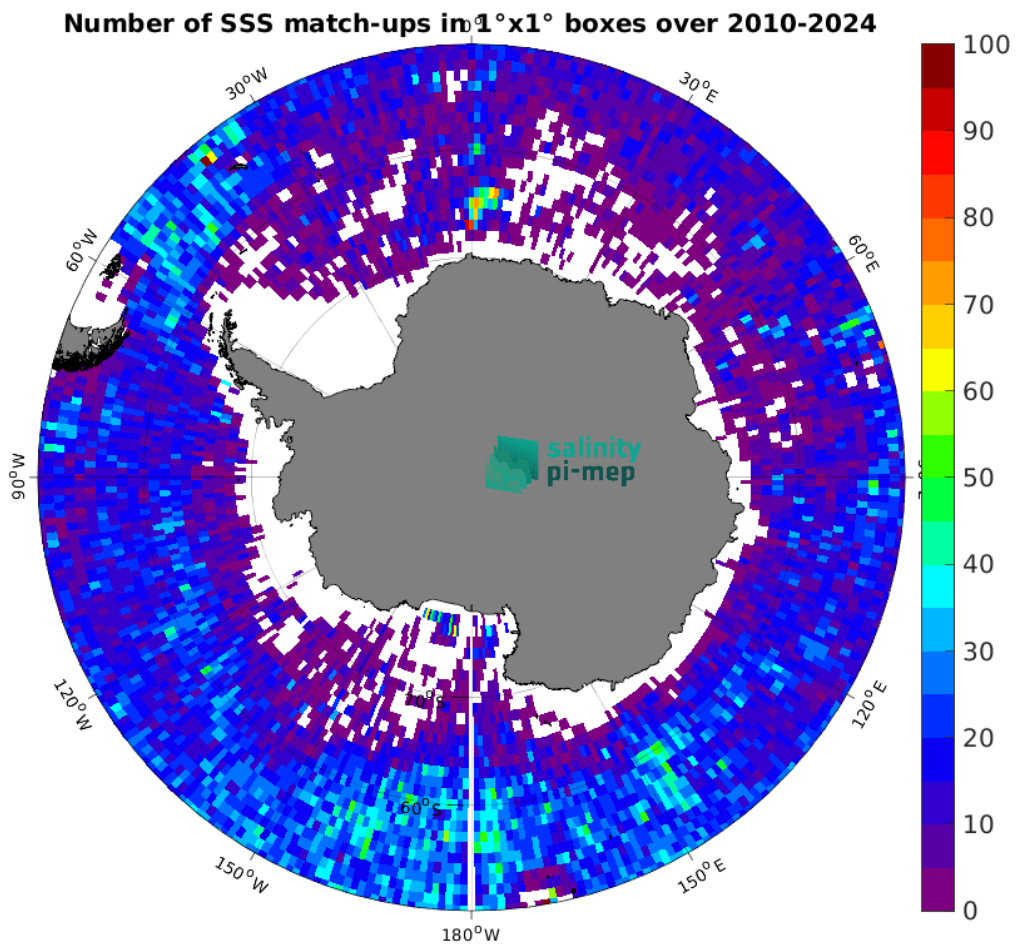
Figure 5: Number of SSS match-ups between Argo SSS and the SMOS SSS L2 v700 (ESA) SSS product for the Southern Ocean Pi-MEP region over 1^\circ \times 1^\circ boxes and for the full satellite product period.
