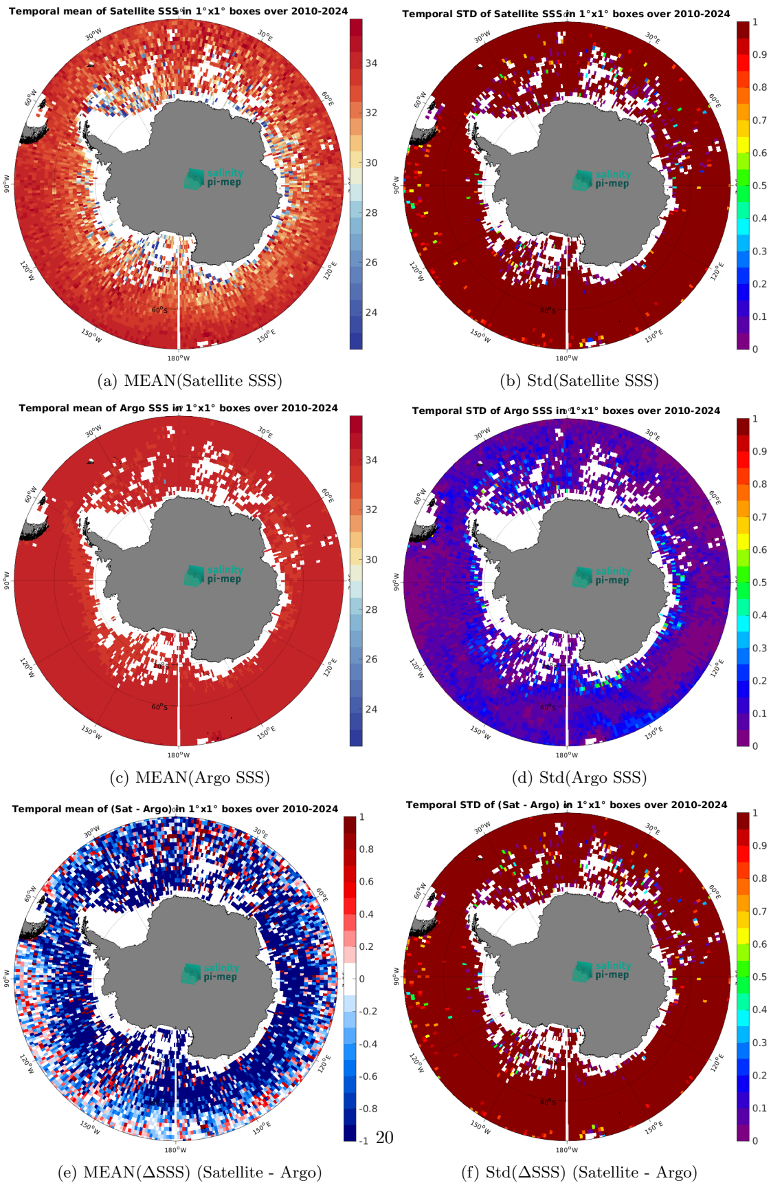
Figure 7: Temporal mean (left) and Std (right) of SSS from SMOS SSS L2 v700 (ESA) (top), Argo (middle), and of \Delta SSS (Satellite - Argo). Only match-up pairs are used to generate these maps.
