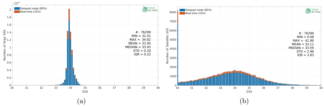
Figure 2: Histograms of SSS from Argo (a) and SMOS SSS L2 v700 (ESA) (b) considering all match-up pairs per bins of 0.1 over the Southern Ocean Pi-MEP region and for the full satellite product period.
