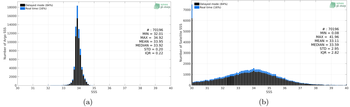
Figure 2: Histograms of SSS from Argo (a) and SMOS SSS L2 v700 (ESA) (b) considering all match-up pairs per bins of 0.1 over the Southern Ocean Pi-MEP region and for the full satellite product period.
