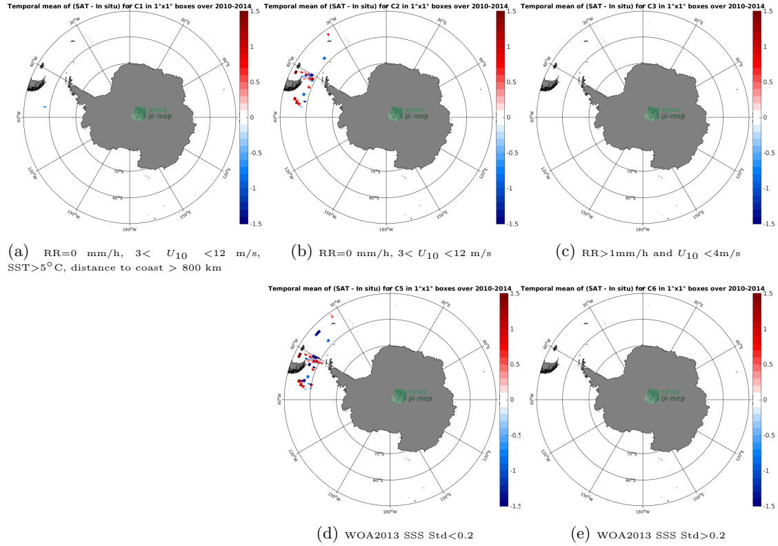
Figure 12: Temporal mean gridded over spatial boxes of size 1^{\circ}\times 1^{\circ} of \Delta\text{SSS} (SMOS SSS L2 v662 (ESA) - TSG (SAMOS)) for 5 different subdatasets corresponding to:RR=0 mm/h, 3 < U_{10} < 12 m/s, SST >5^{\circ}\text{C} , distance to coast > 800 km (a), RR=0 mm/h, 3 < U_{10} < 12 m/s (b), RR >1 mm/h and U_{10} < 4 m/s (c), WOA2013 SSS Std <0.2 (d), WOA2013 SSS Std >0.2 (e).
