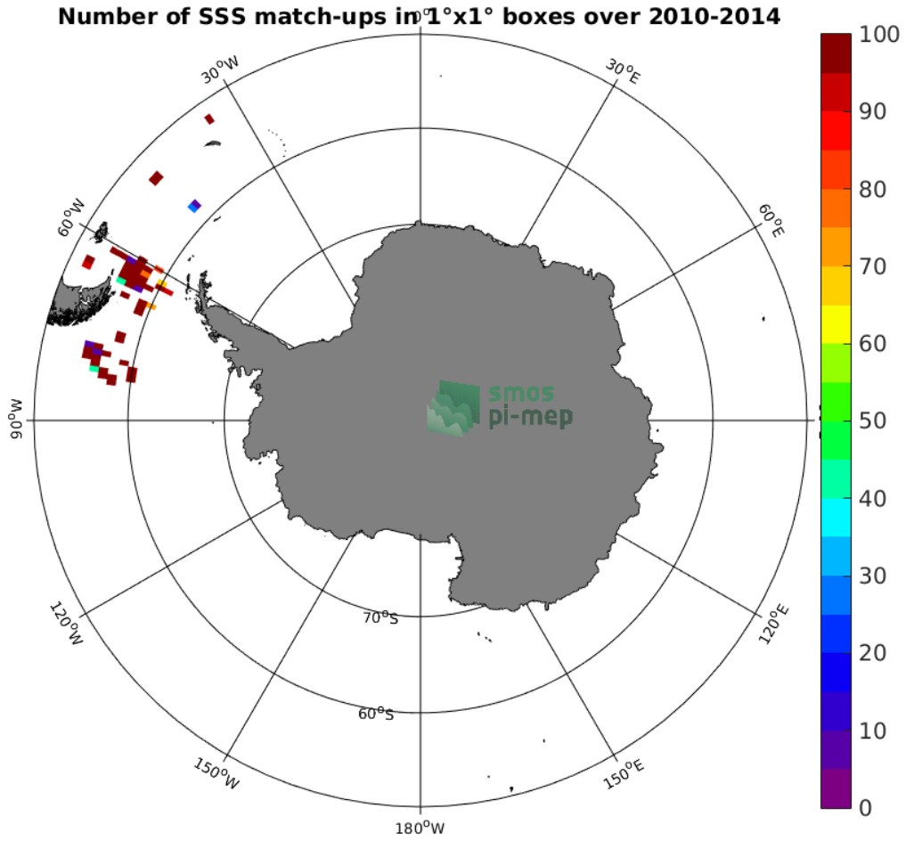
Figure 4: Number of SSS match-ups between TSG (SAMOS) SSS and the SMOS SSS L2 v662 (ESA) SSS product for the Southern Ocean Pi-MEP region over 1^\circ \times 1^\circ boxes and for the full satellite product period.
