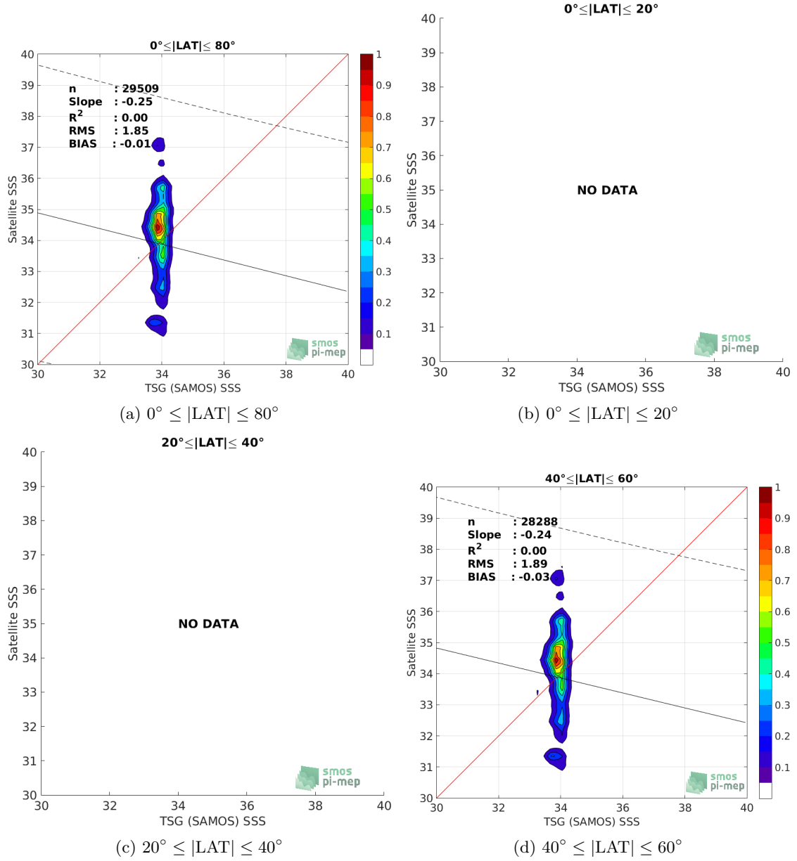
Figure 9: Contour maps of the concentration of SMOS SSS L2 v662 (ESA) SSS (y-axis) versus TSG (SAMOS) SSS (x-axis) at match-up pairs for different latitude bands. For each plot, the red line shows x=y . The black thin and dashed lines indicate a linear fit through the data cloud and the \pm 95\% confidence levels, respectively. The number match-up pairs n , the slope and R^2 coefficient of the linear fit, the root mean square (RMS) and the mean bias between satellite and in situ data are indicated for each latitude band in each plots.
