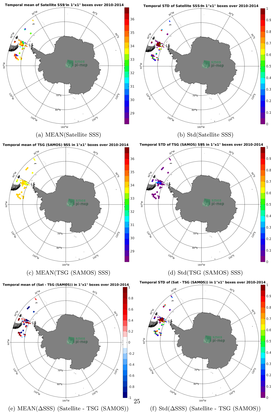
Figure 6: Temporal mean (left) and Std (right) of SSS from SMOS SSS L2 v662 (ESA) (top), TSG (SAMOS) (middle), and of \Delta SSS (Satellite - TSG (SAMOS)). Only match-up pairs are used to generate these maps.
