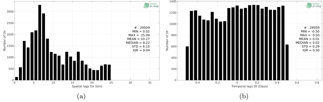
Figure 5: Histograms of the spatial (a) and temporal (b) lags between the location/time of the TSG (SAMOS) measurement and the date of the corresponding SMOS SSS L2 v662 (ESA) SSS pixel.
