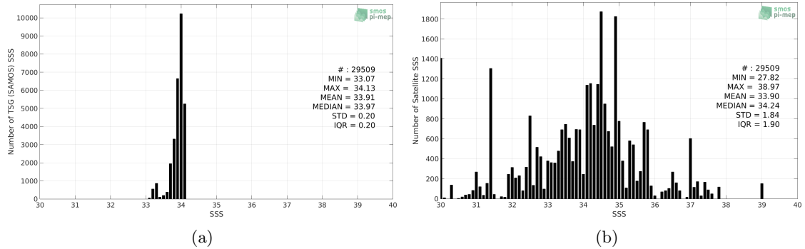
Figure 2: Histograms of SSS from TSG (SAMOS) (a) and SMOS SSS L2 v662 (ESA) (b) considering all match-up pairs per bins of 0.1 over the Southern Ocean Pi-MEP region and for the full satellite product period.
