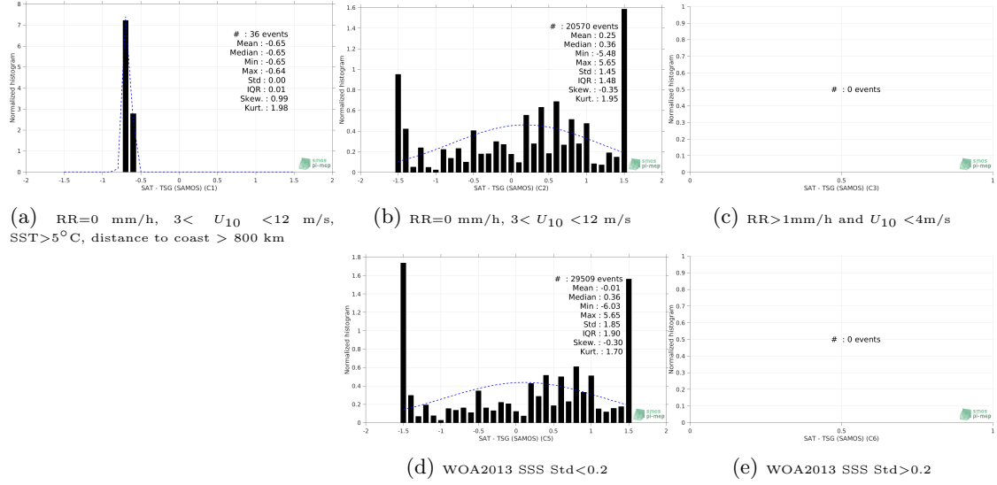
Figure 13: Normalized histogram of \Delta\text{SSS} (SMOS SSS L2 v662 (ESA) - TSG (SAMOS)) for 5 different subdatasets corresponding to: RR=0 mm/h, 3 < U_{10} < 12 m/s, SST > 5^\circ\text{C} , distance to coast > 800 km (a), RR=0 mm/h, 3 < U_{10} < 12 m/s (b), RR > 1\text{mm/h} and U_{10} < 4\text{m/s} (c), WOA2013 SSS Std < 0.2 (d), WOA2013 SSS Std > 0.2 (e).
