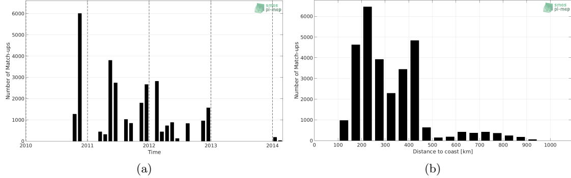
Figure 1: Number of match-ups between TSG (SAMOS) and SMOS SSS L2 v662 (ESA) SSS as a function of time (a) and as function of the distance to coast (b) over the Southern Ocean Pi-MEP region and for the full satellite product period.
