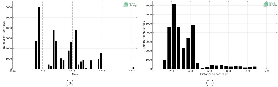
Figure 1: Number of match-ups between TSG-SAMOS and SMOS L2 v662 (ESA) SSS as a function of time (a) and as function of the distance to coast (b) over the Southern Ocean Pi-MEP region and for the full satellite product period.
