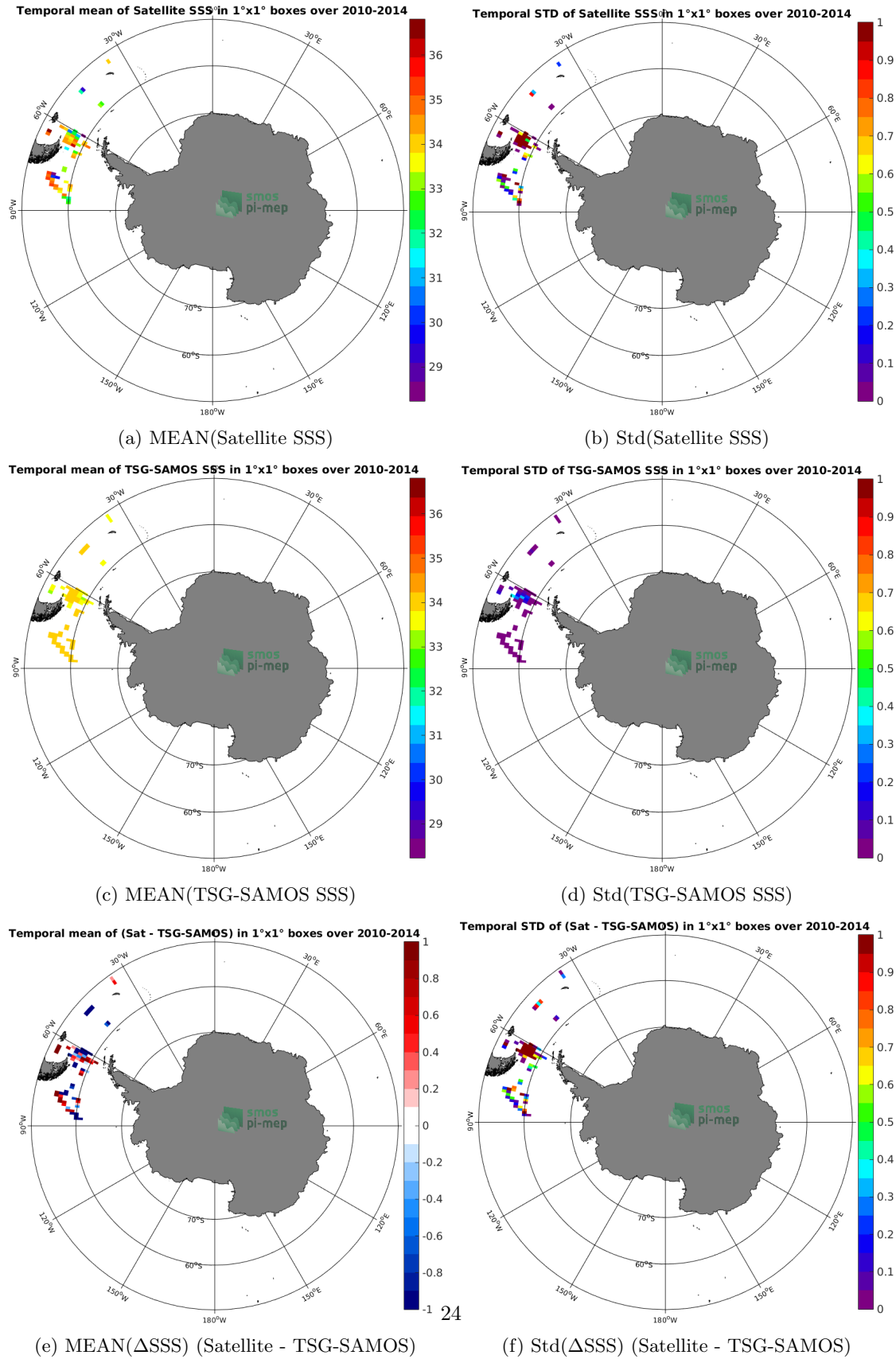
Figure 6: Temporal mean (left) and Std (right) of SSS from SMOS L2 v662 (ESA) (top), TSG-SAMOS (middle), and of \Delta SSS (Satellite - TSG-SAMOS). Only match-up pairs are used to generate these maps.
