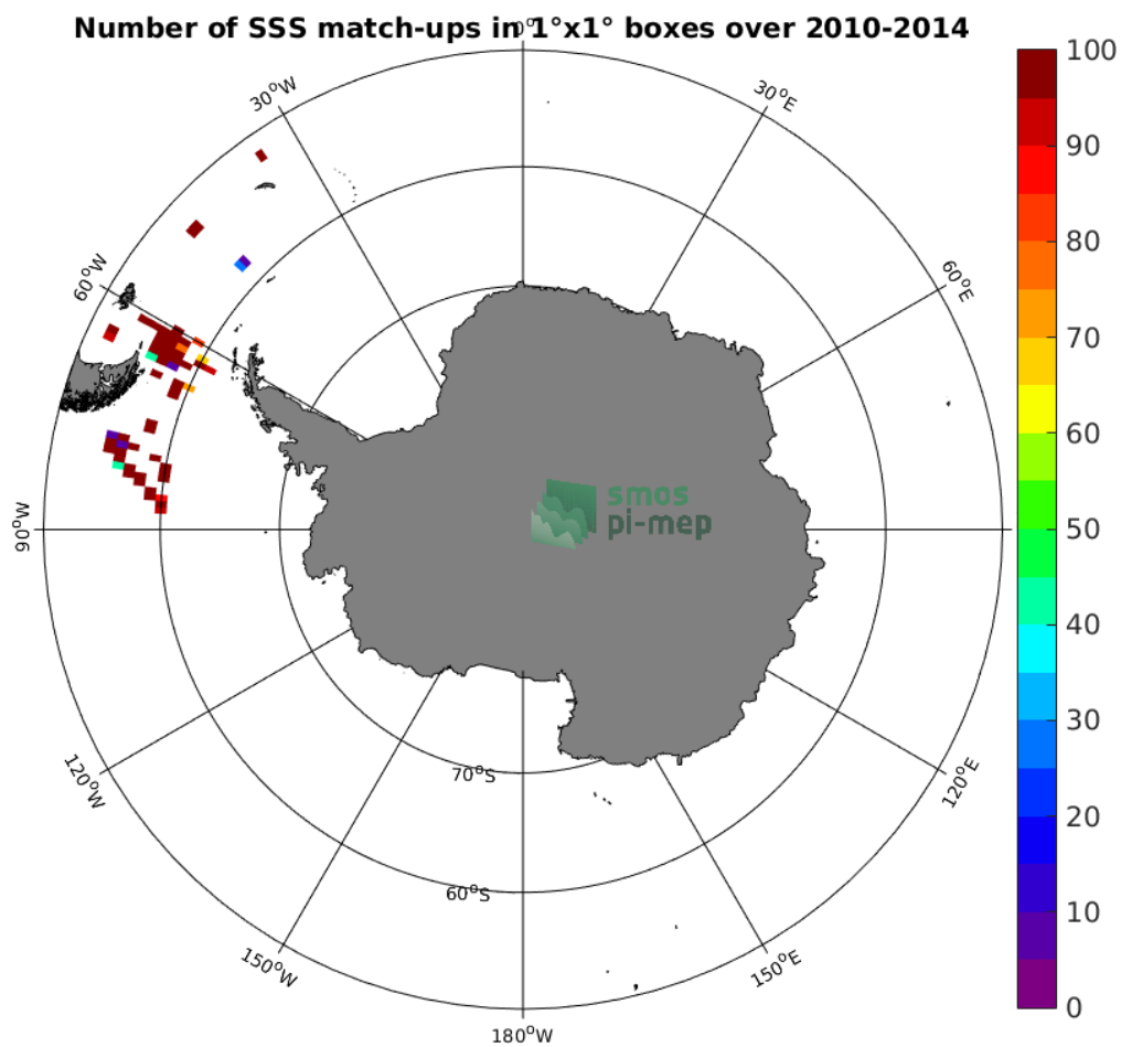
Figure 4: Number of SSS match-ups between TSG-SAMOS SSS and the SMOS L2 v662 (ESA) SSS product for the Southern Ocean Pi-MEP region over 1^\circ \times 1^\circ boxes and for the full satellite product period.
