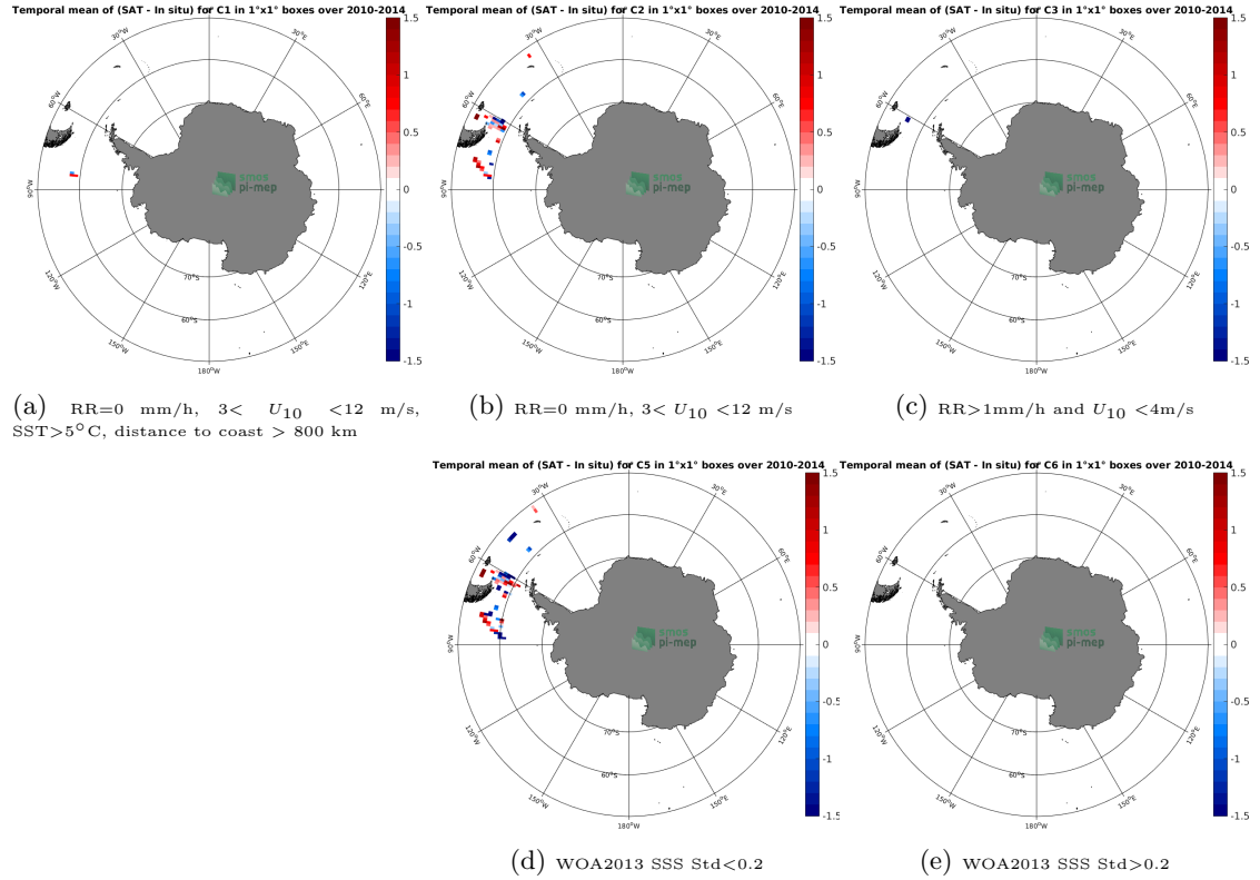
Figure 12: Temporal mean gridded over spatial boxes of size 1^{\circ}\times 1^{\circ} of \Delta\text{SSS} (SMOS L2 v662 (ESA) - TSG-SAMOS) for 5 different subdatasets corresponding to: \text{RR}=0 mm/h, 3 < U_{10} < 12 m/s, \text{SST}>5^{\circ}\text{C} , distance to coast > 800 km (a), \text{RR}=0 mm/h, 3 < U_{10} < 12 m/s (b), \text{RR}>1\text{mm/h} and U_{10} < 4\text{m/s} (c), WOA2013 SSS Std <0.2 (d), WOA2013 SSS Std >0.2 (e).
