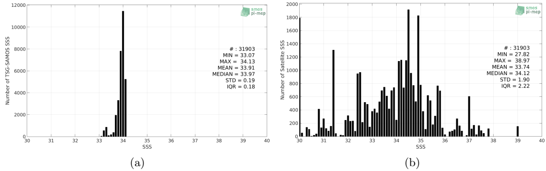
Figure 2: Histograms of SSS from TSG-SAMOS (a) and SMOS L2 v662 (ESA) (b) considering all match-up pairs per bins of 0.1 over the Southern Ocean Pi-MEP region and for the full satellite product period.
