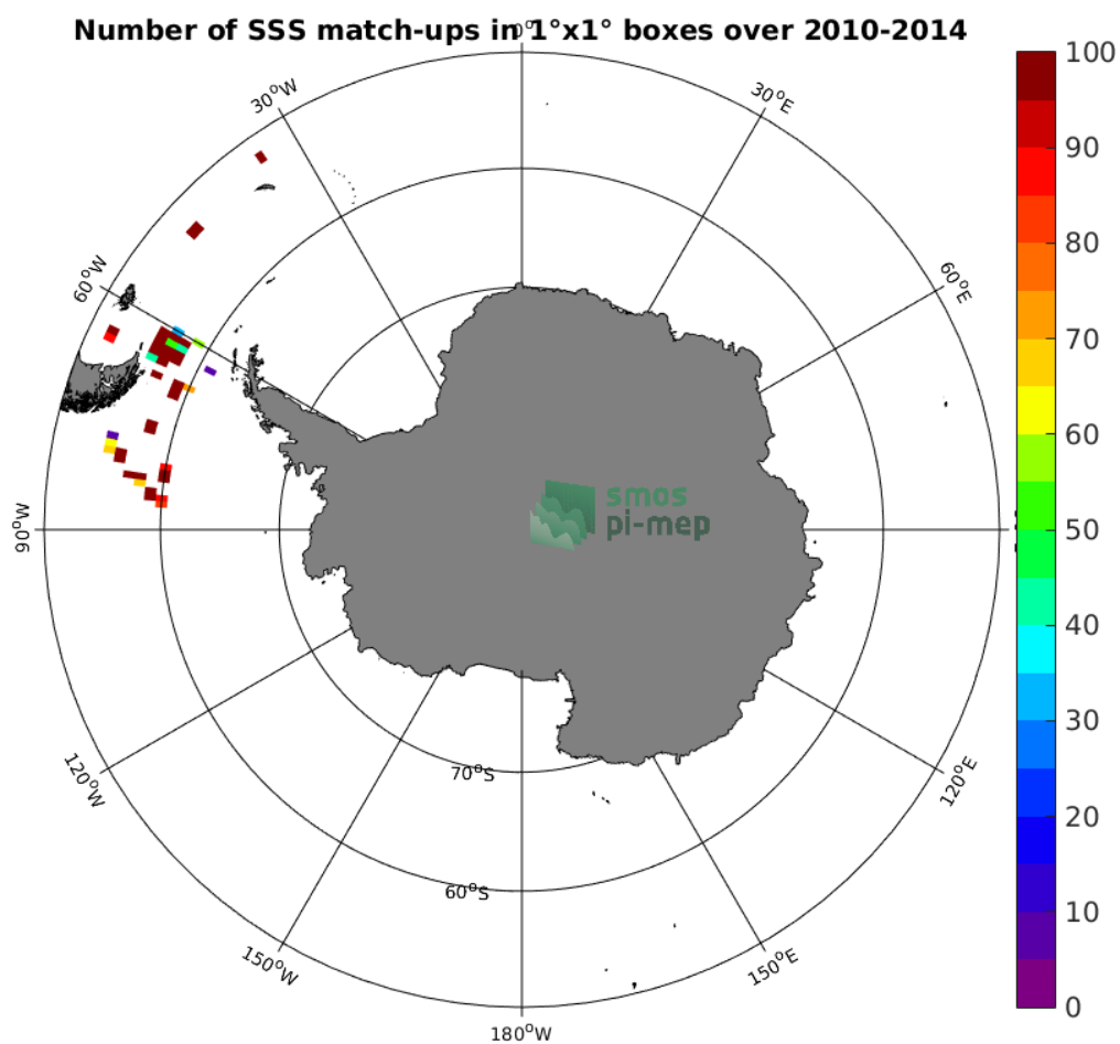
Figure 4: Number of SSS match-ups between TSG-SAMOS SSS and the SMOS-L2-DPGS-v662 SSS product for the Southern Ocean Pi-MEP region over 1^\circ \times 1^\circ boxes and for the full satellite product period.
