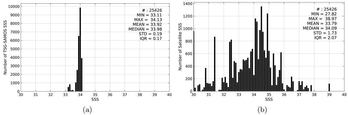
Figure 2: Histograms of SSS from TSG-SAMOS (a) and SMOS-L2-DPGS-v662 (b) considering all match-up pairs per bins of 0.1 over the Southern Ocean Pi-MEP region and for the full satellite product period.
