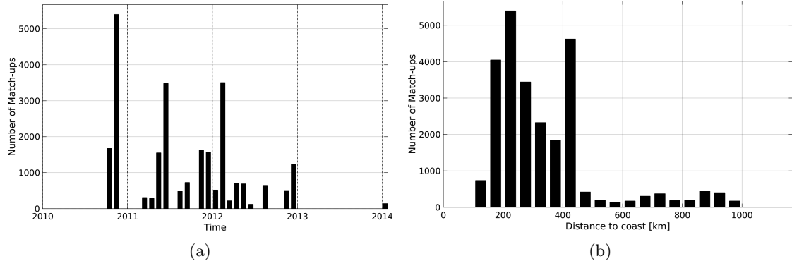
Figure 1: Number of match-ups between TSG-SAMOS and SMOS-L2-DPGS-v662 SSS as a function of time (a) and as function of the distance to coast (b) over the Southern Ocean Pi-MEP region and for the full satellite product period.
